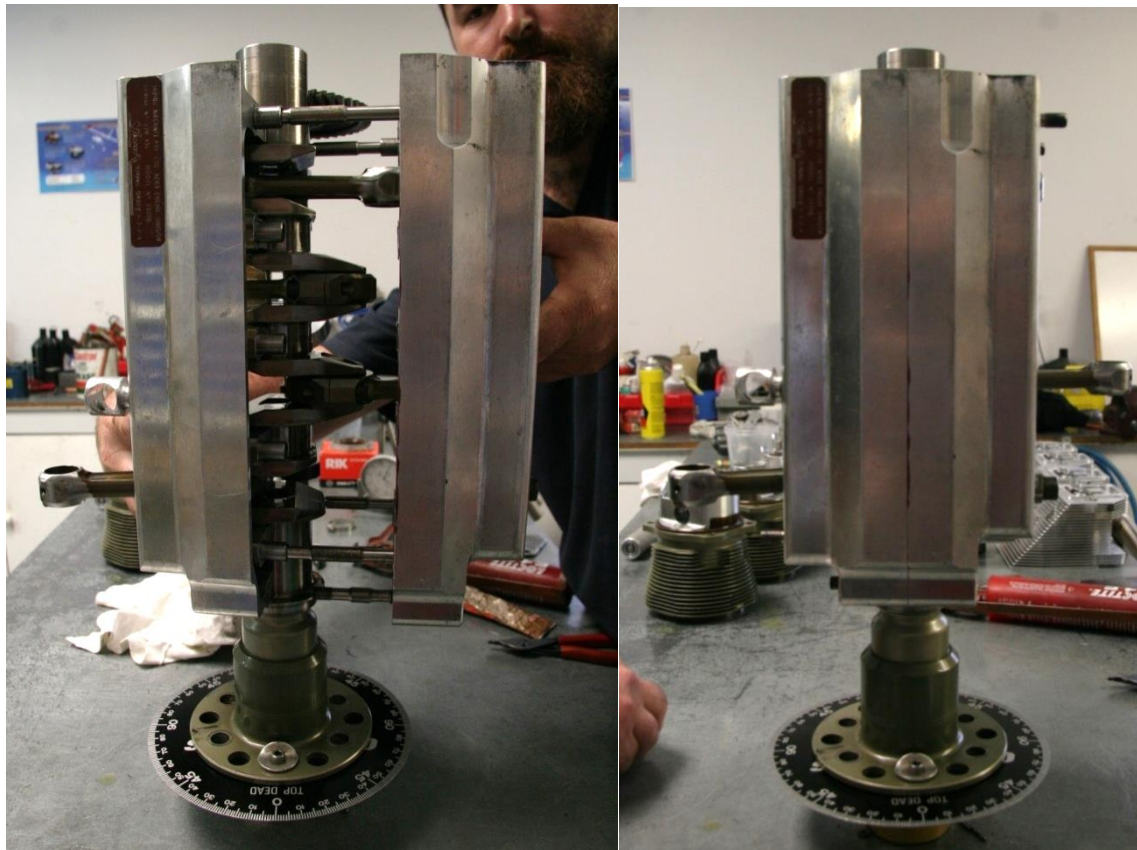
Figure 159 – Fitting The Second Case Half
