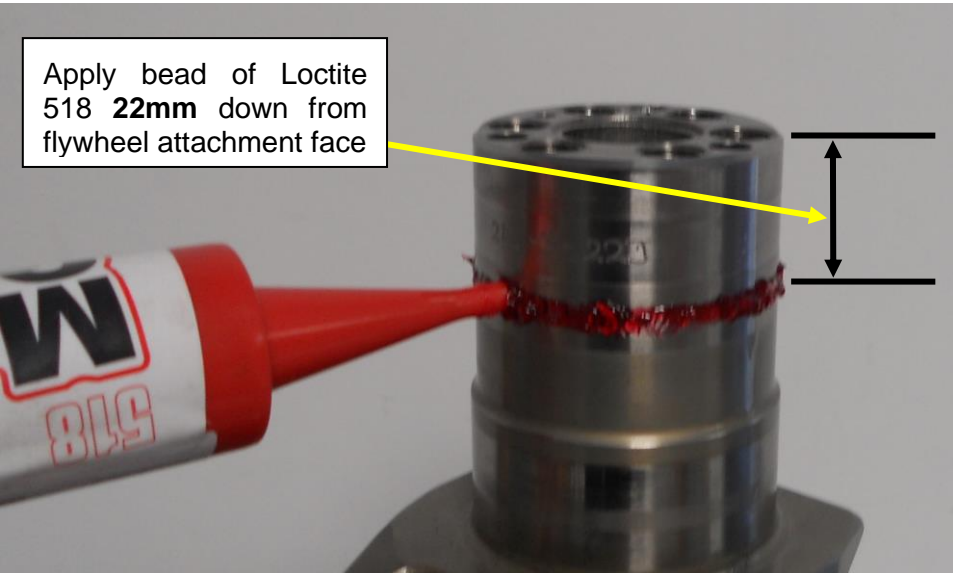
Figure 168 - Apply bead of Loctite 518 around perimeter of crank-gear
