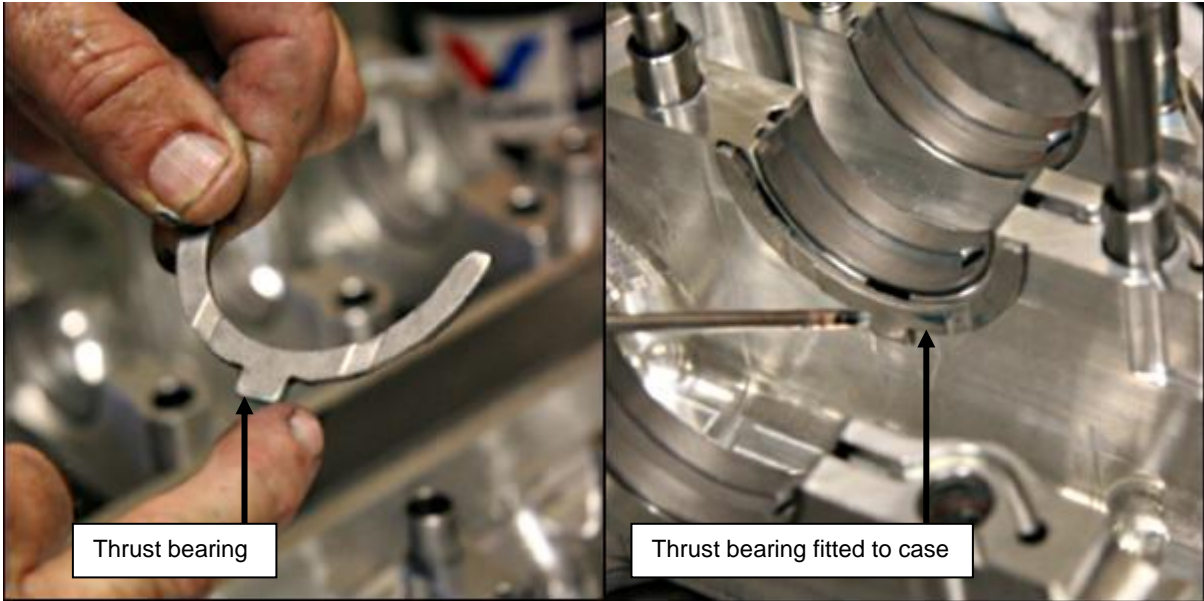
Figure 128 – Fitting Thrust Bearings
