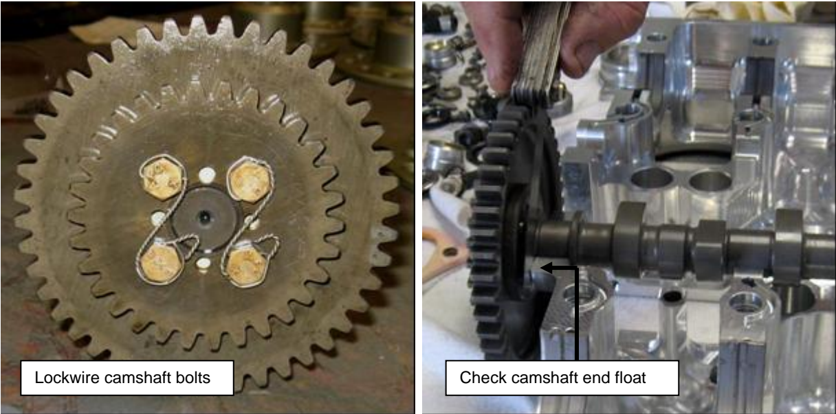
Figure 132 – Assembling Cam & Fitting to Crankcase
