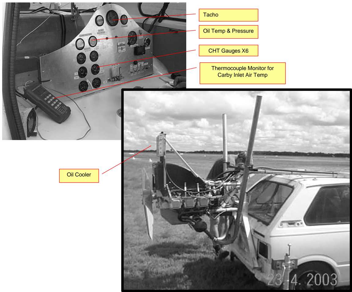
Figure 211 – Engine Ground Running Rig
