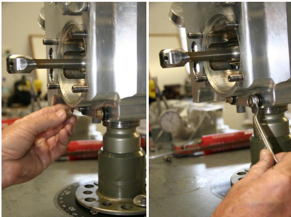
Figure 160 – Tightening The Front Crankcase Studs
