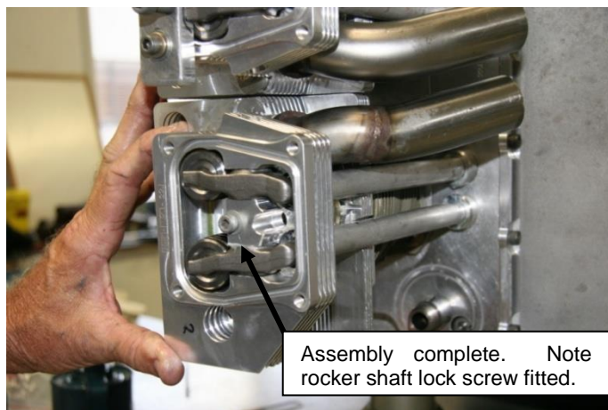
Figure 194 – Fitting Rockers #3
