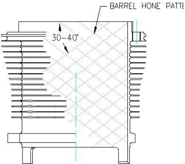
Figure 88 – Cylinder hone Pattern
