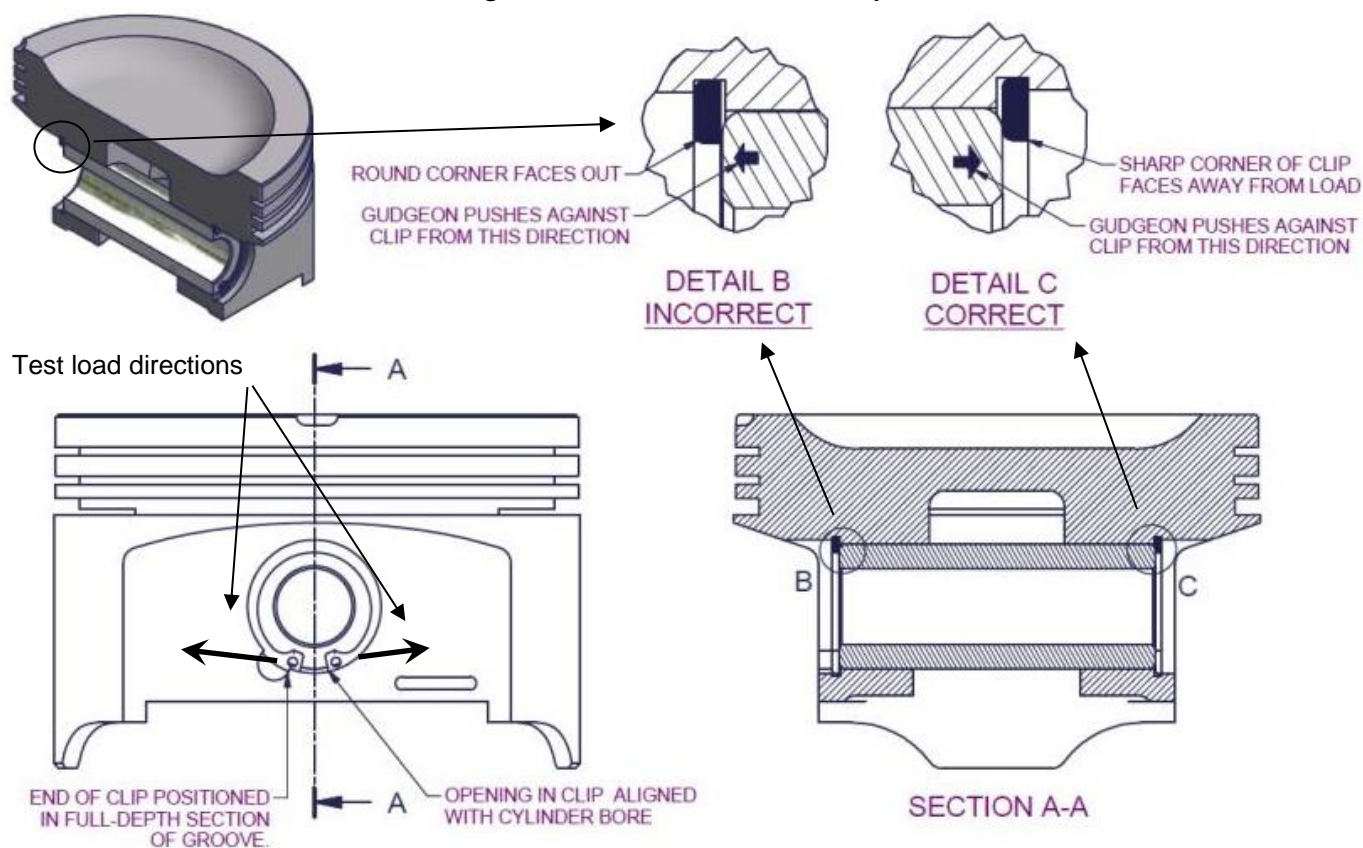
Figure 138 – Clip Installation Detail
