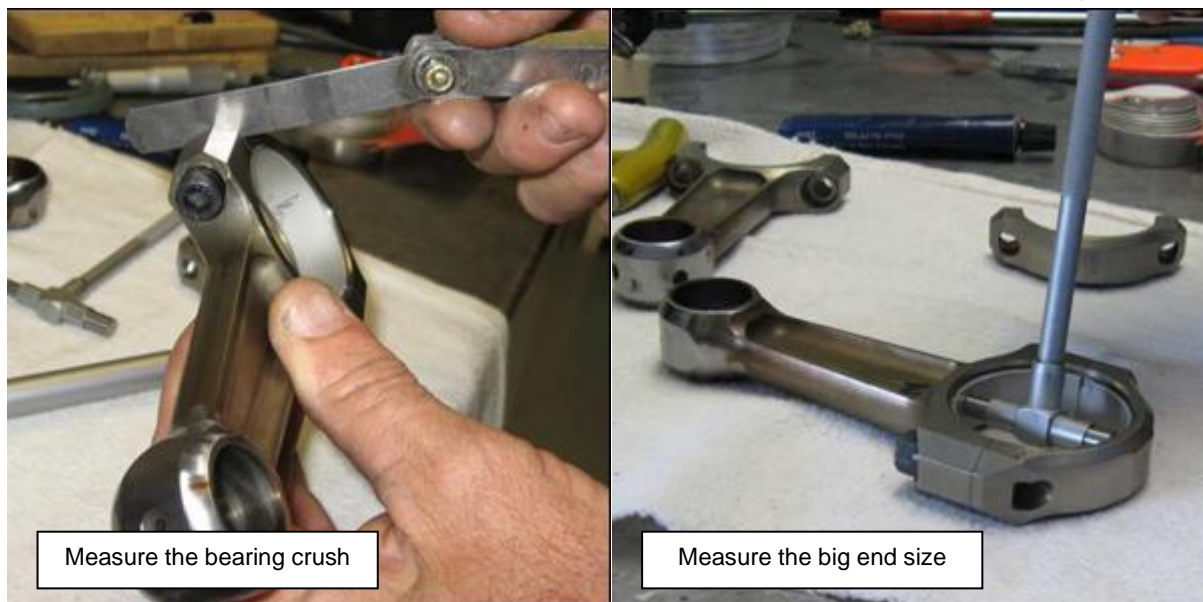
Figure 122 – Measuring Connecting Rods
