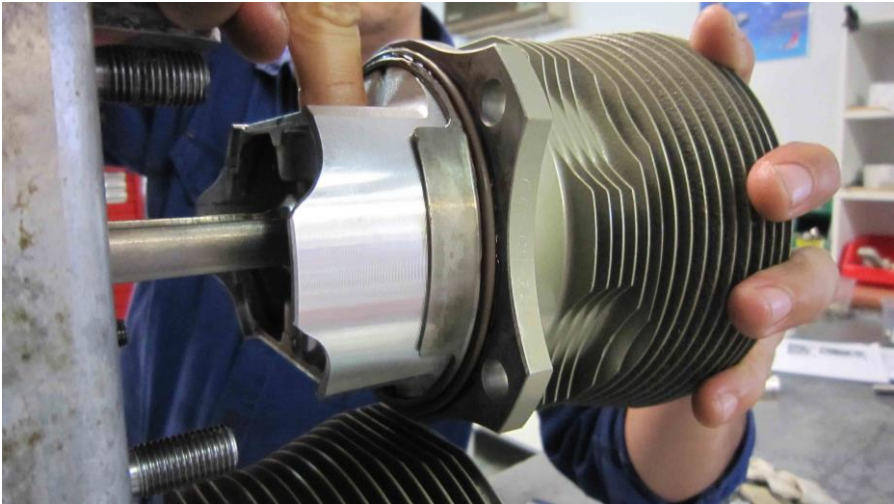
Figure 162 – Fitting Gudgeon Pin
