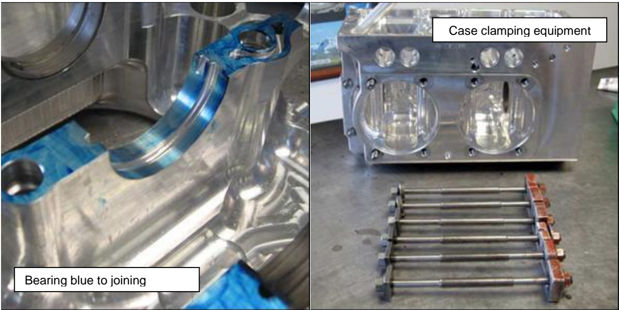
Figure 127 – Crankcase Clamping Preparation
