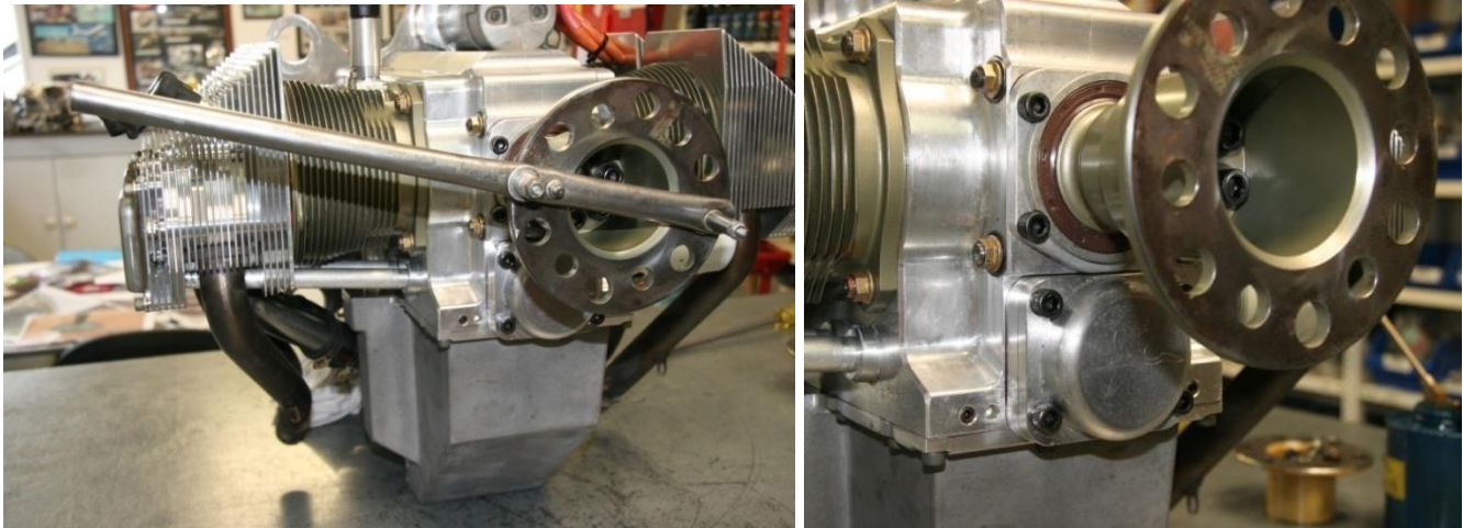
Figure 208 – Engine Turning Tool, Installed Oil Pump
