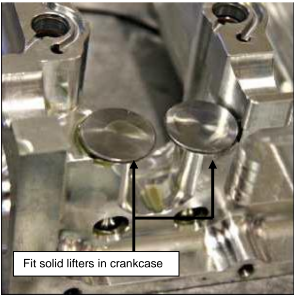
Figure 130 – Checking Crankshaft End Float, Installing Solid Lifters
