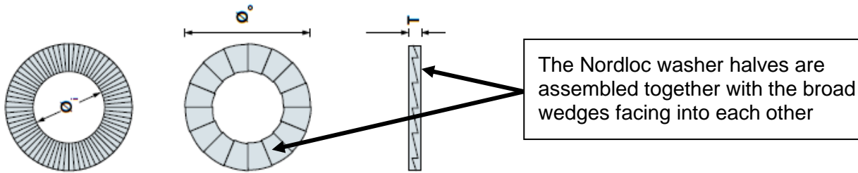
Figure 184 - Nordloc washer halves assembled together
