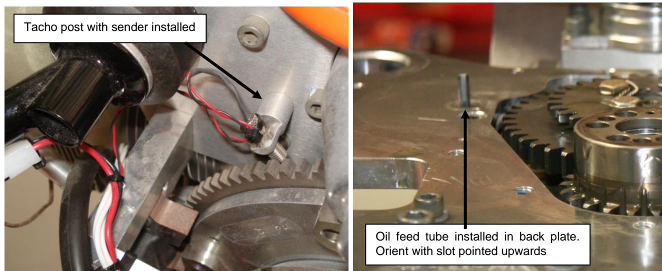
Figure 152 – Installation of Oil Feed Tubes & Tacho Pickup Post
