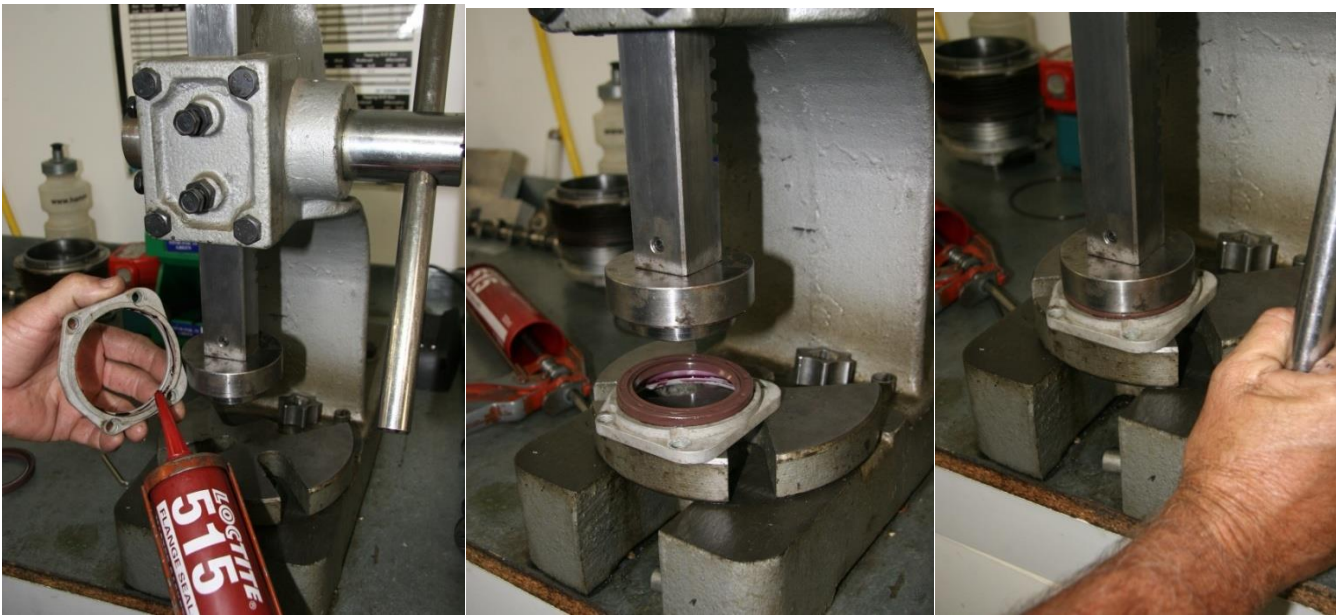
Figure 203 – Fitting Seal To Housing
