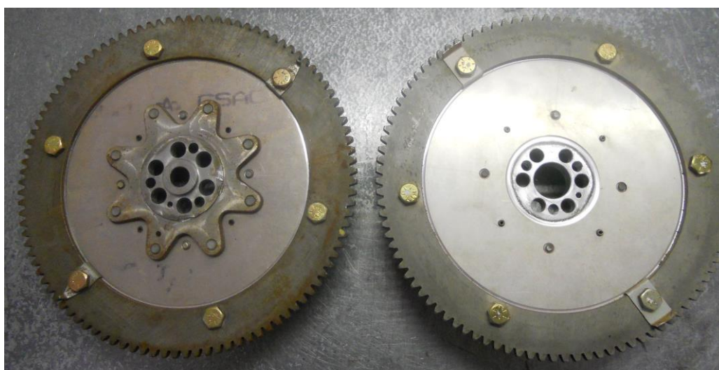
Figure 181 – Steel centred flywheel (left) aluminium flywheel (right).
