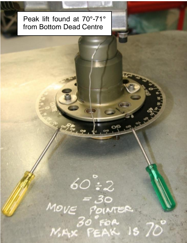
Figure 171 – Checking Cam Timing #2
