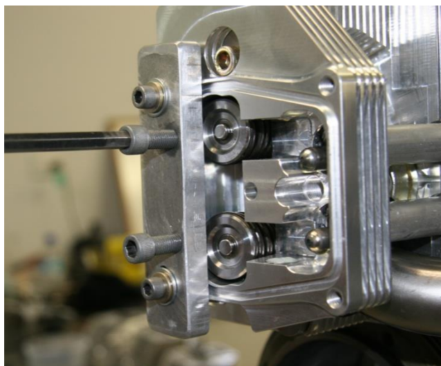
Figure 194 – Fitting Rockers #3
