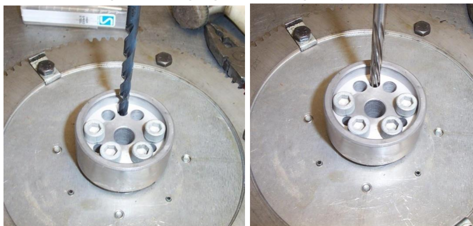
Figure 221 – Drilling & Reaming Flywheel – ILLUSTRATION ONLY.
