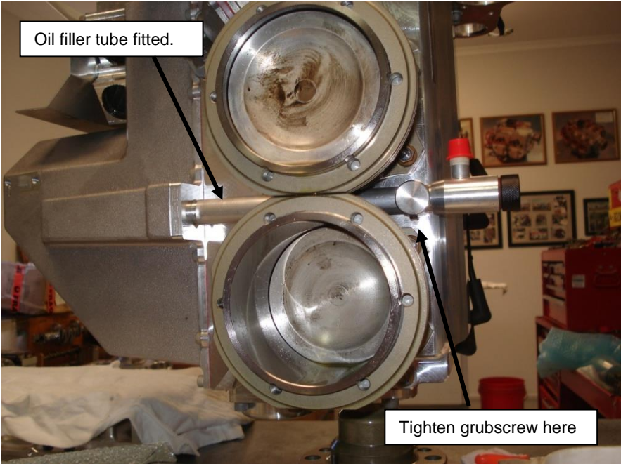
Figure 173 – Oil Filler Tube Installation
