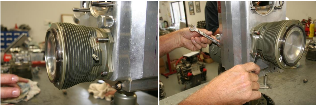
Figure 163 – Fitting Cylinder, Inserting & Tightening Through-Bolts
