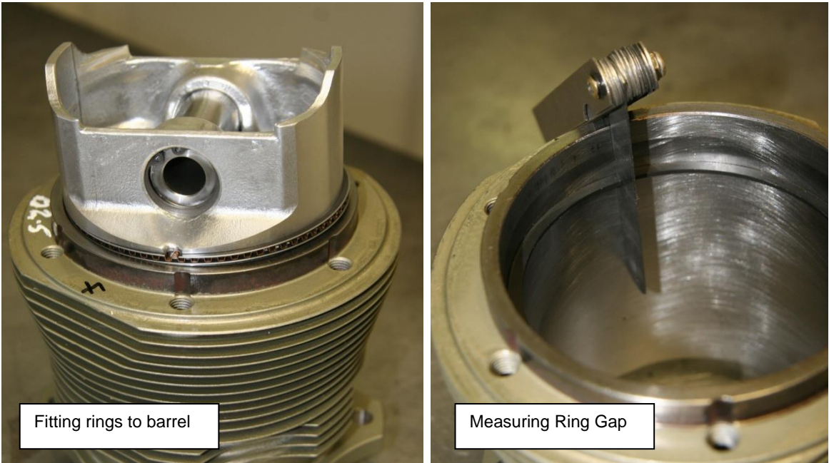
Figure 140 – Checking Piston Ring Gap
