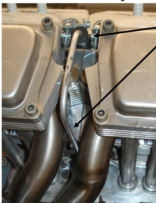
Figure 195 – Rocker Lube (Left) &amp; Crankcase Oil Port Blanking Plug
