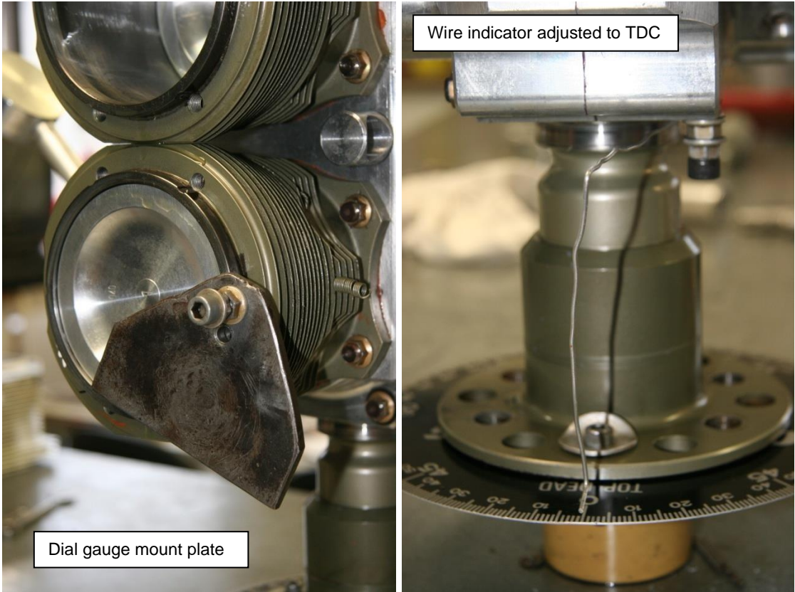
Figure 167 – Measuring Top Dead Centre
