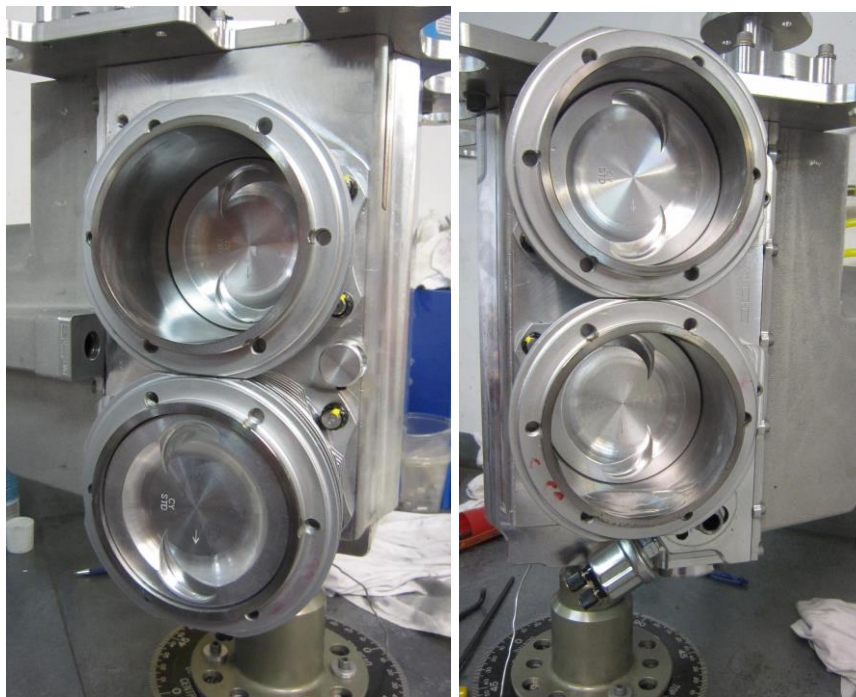
Figure 164 – Piston Orientation
