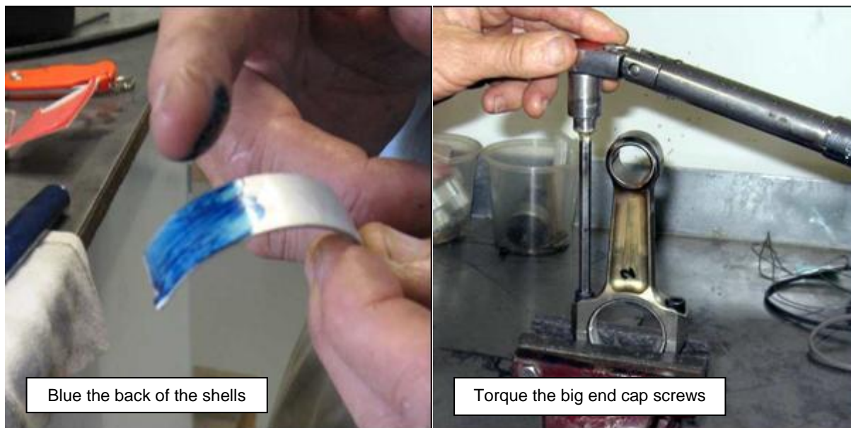
Figure 121 – Blueing Bearings, Assembling Rods
