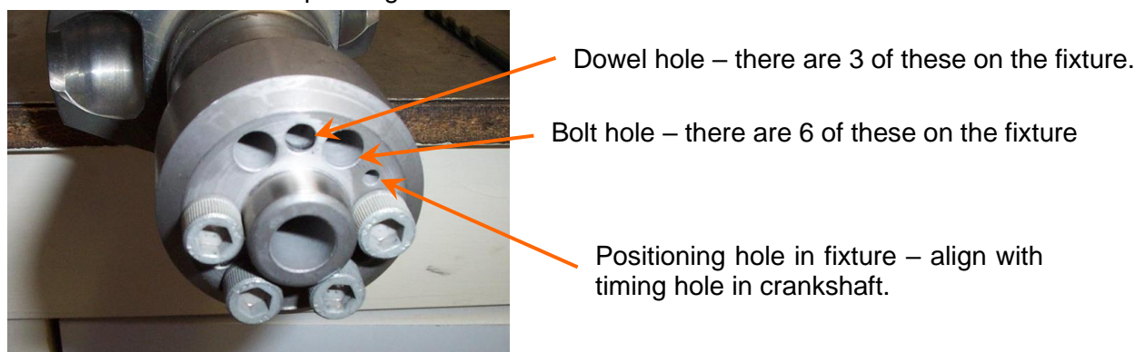
Figure 218 – Guide positioned on crankshaft.
