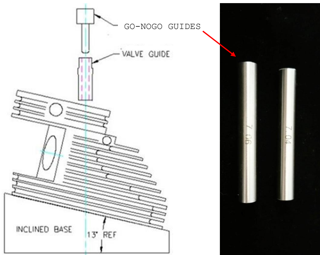
Figure 92 – Valve Guides
