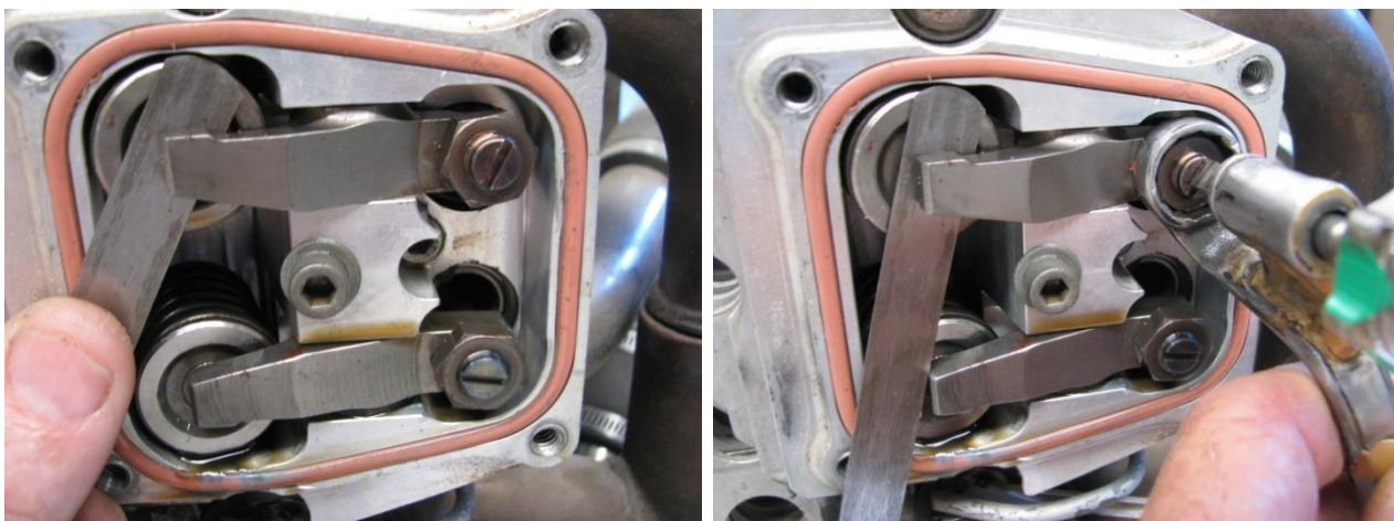
Figure 196 – Valve Clearance Adjustment (Solid Lifter)
