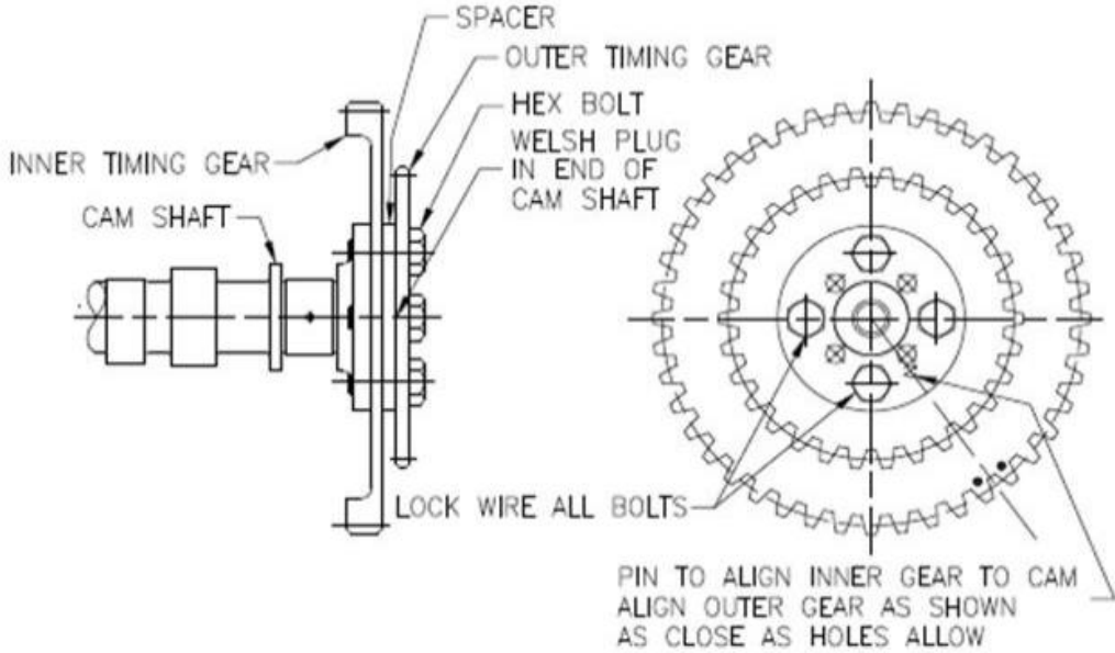
Figure 131 – Cam Timing Gear Assembly
