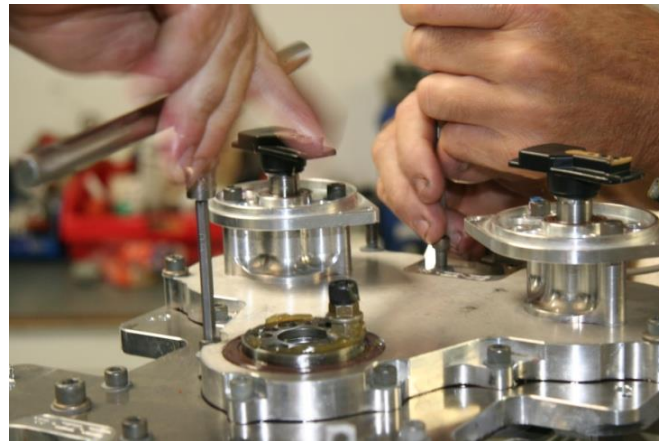
Figure 179 – Checking Rotors, Tightening Distributor Case
