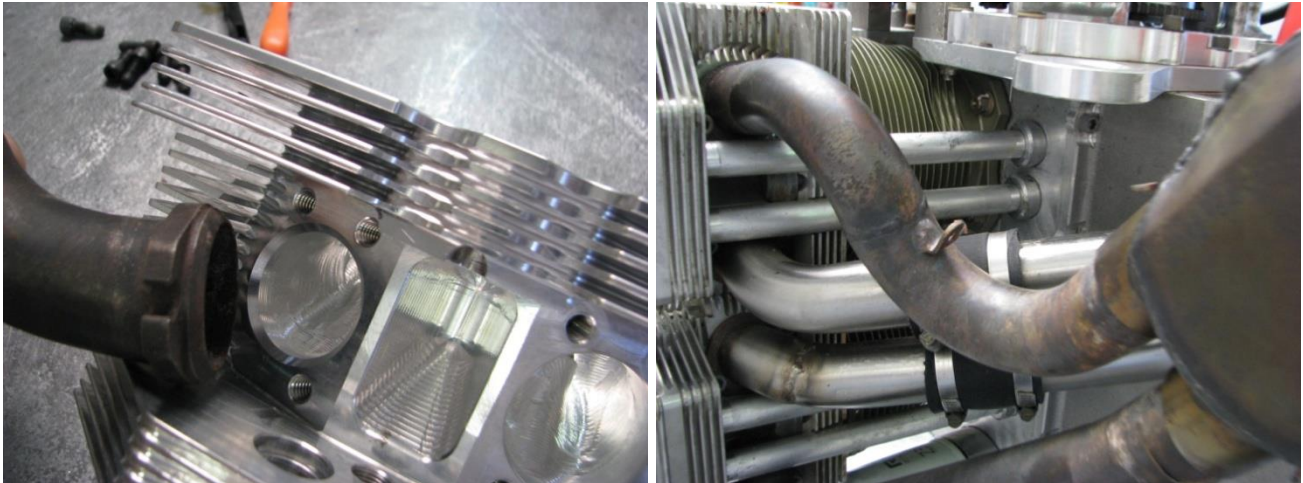
Figure 200 – Exhaust Installation
