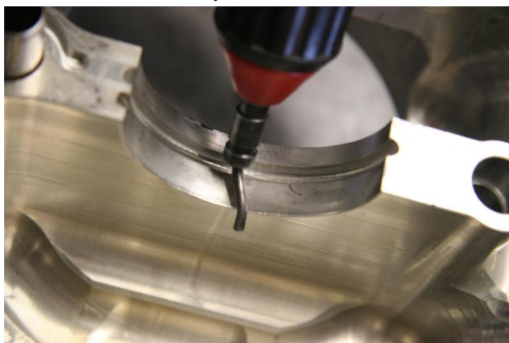
Figure 215 – De-Burring Crankcase After Surfacing & Line Boring
