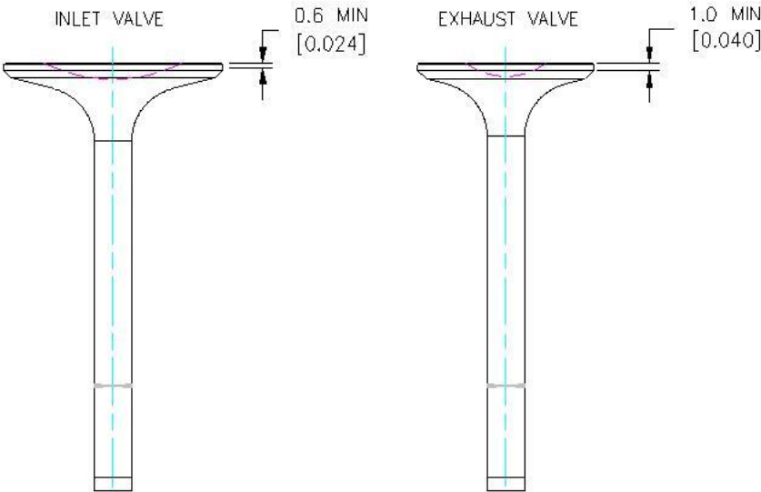
Figure 90 – Valve Measuring
