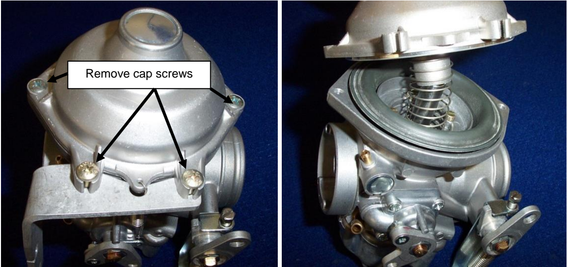
Figure 115 – Disassembling Carburettor #1
