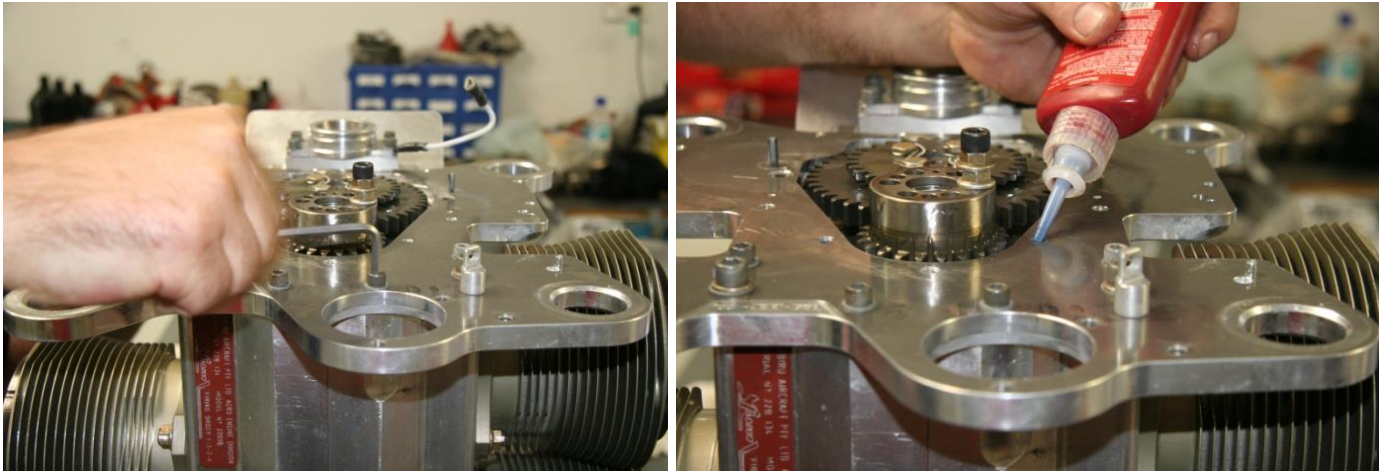
Figure 175 – Fitting Engine Mount Plate
