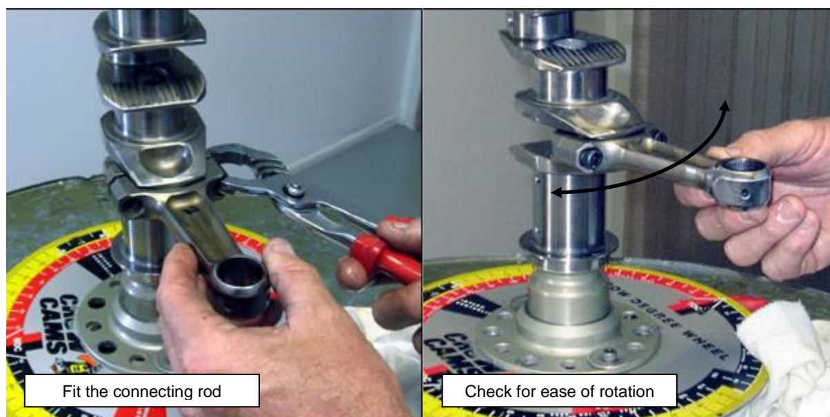
Figure 123 – Fit Connecting Rods
