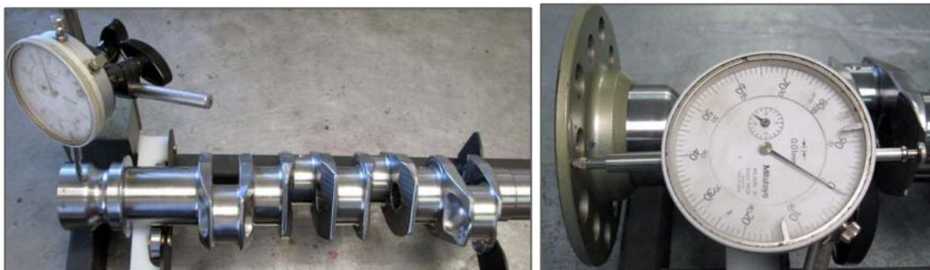
Figure 66 – Crankshaft Measurement
