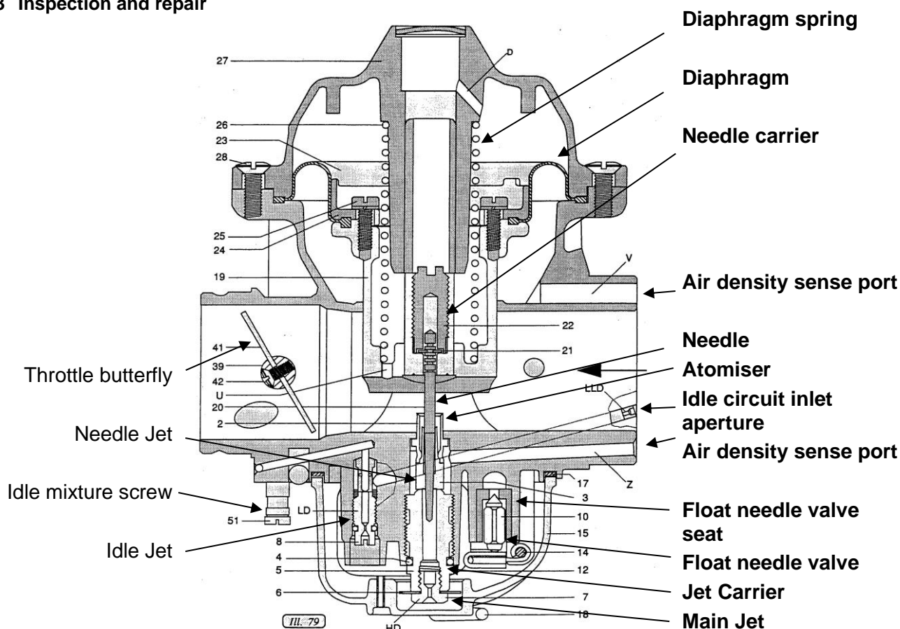
Figure 114 – Carburettor Schematic
