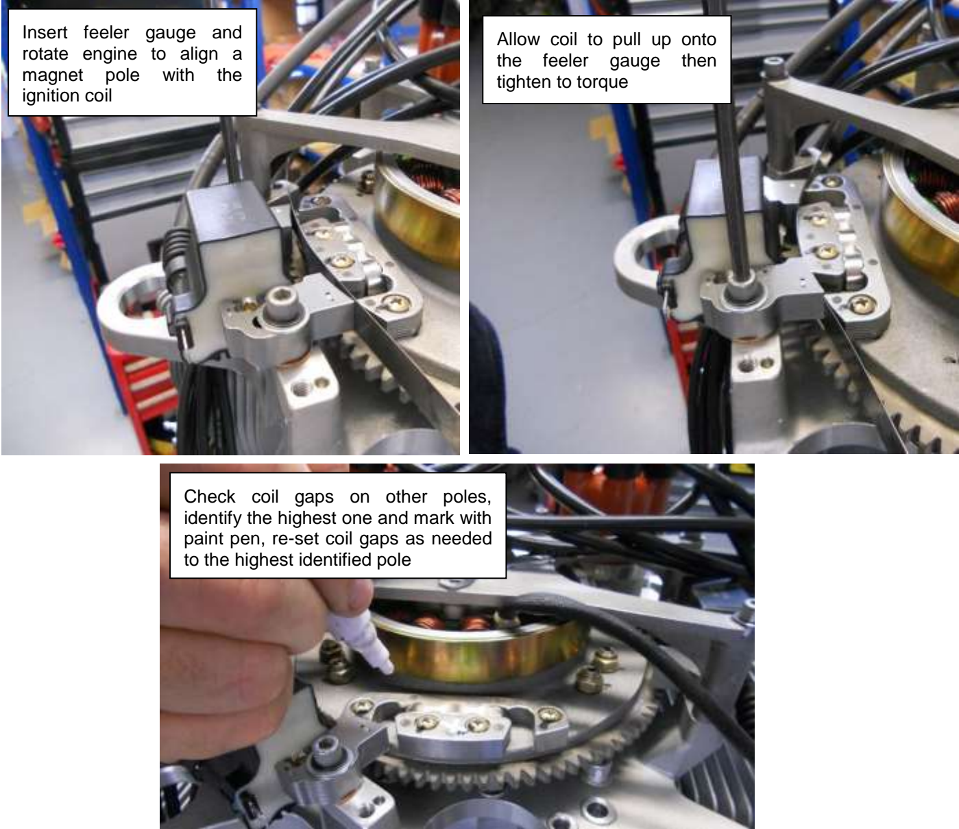
Figure 188 - Setting ignition coil gaps
