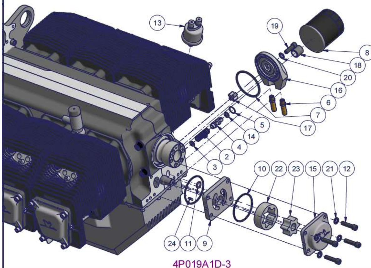
Figure 166 – 3300 Oil pump and filter installation (billet crankcase) – Parts List
