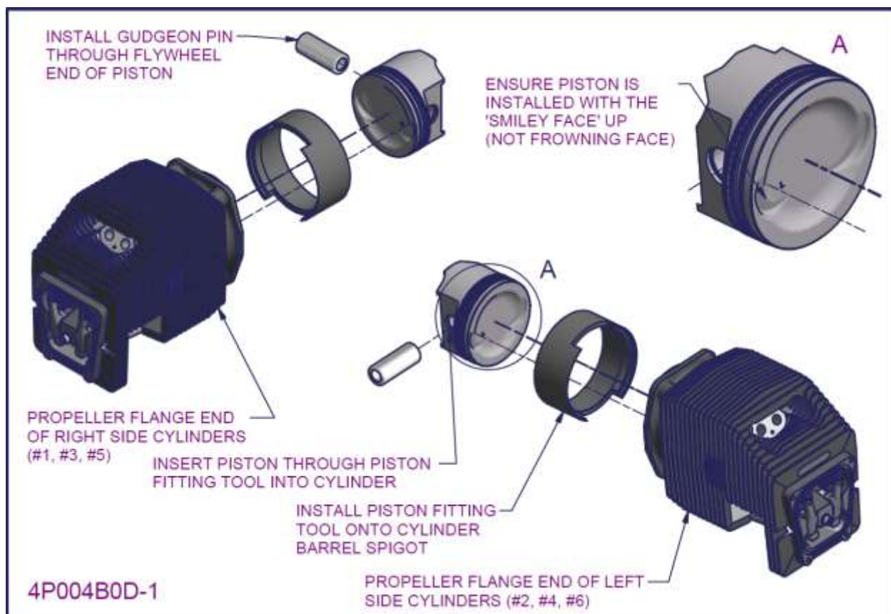
Figure 67 – 2200/3300 cylinder assembly 9
