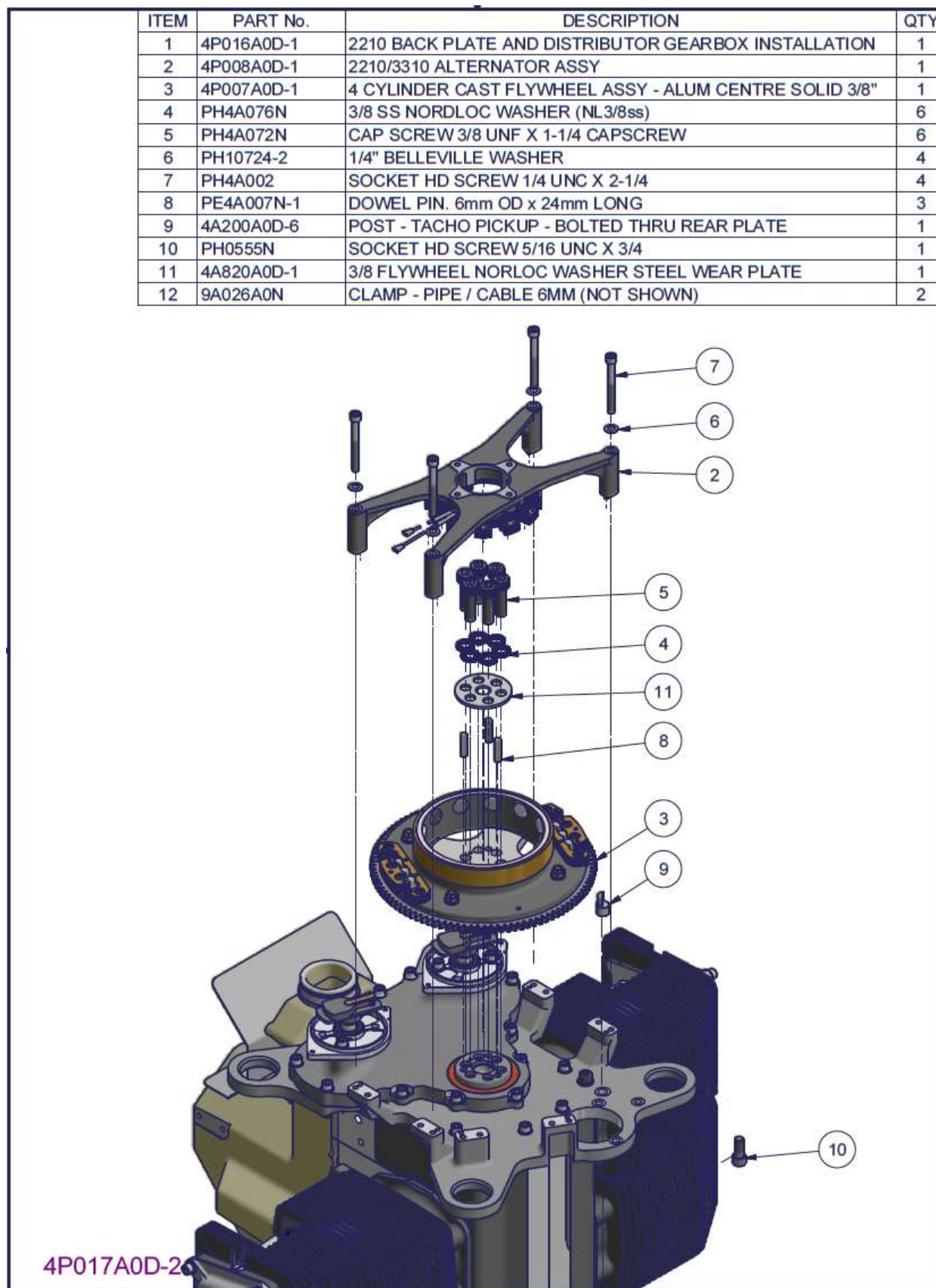
Figure 151 – 2200 flywheel and alternator installation – Parts List
