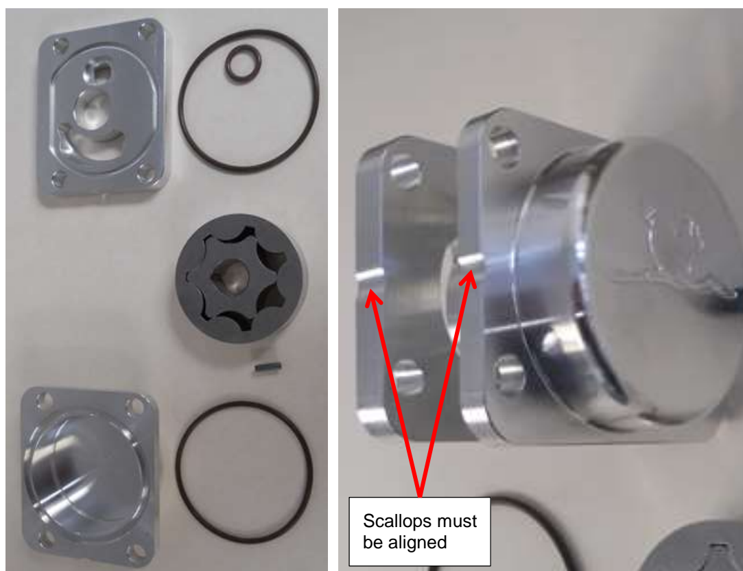
Figure 171 – Details on the six lobe oil pump
