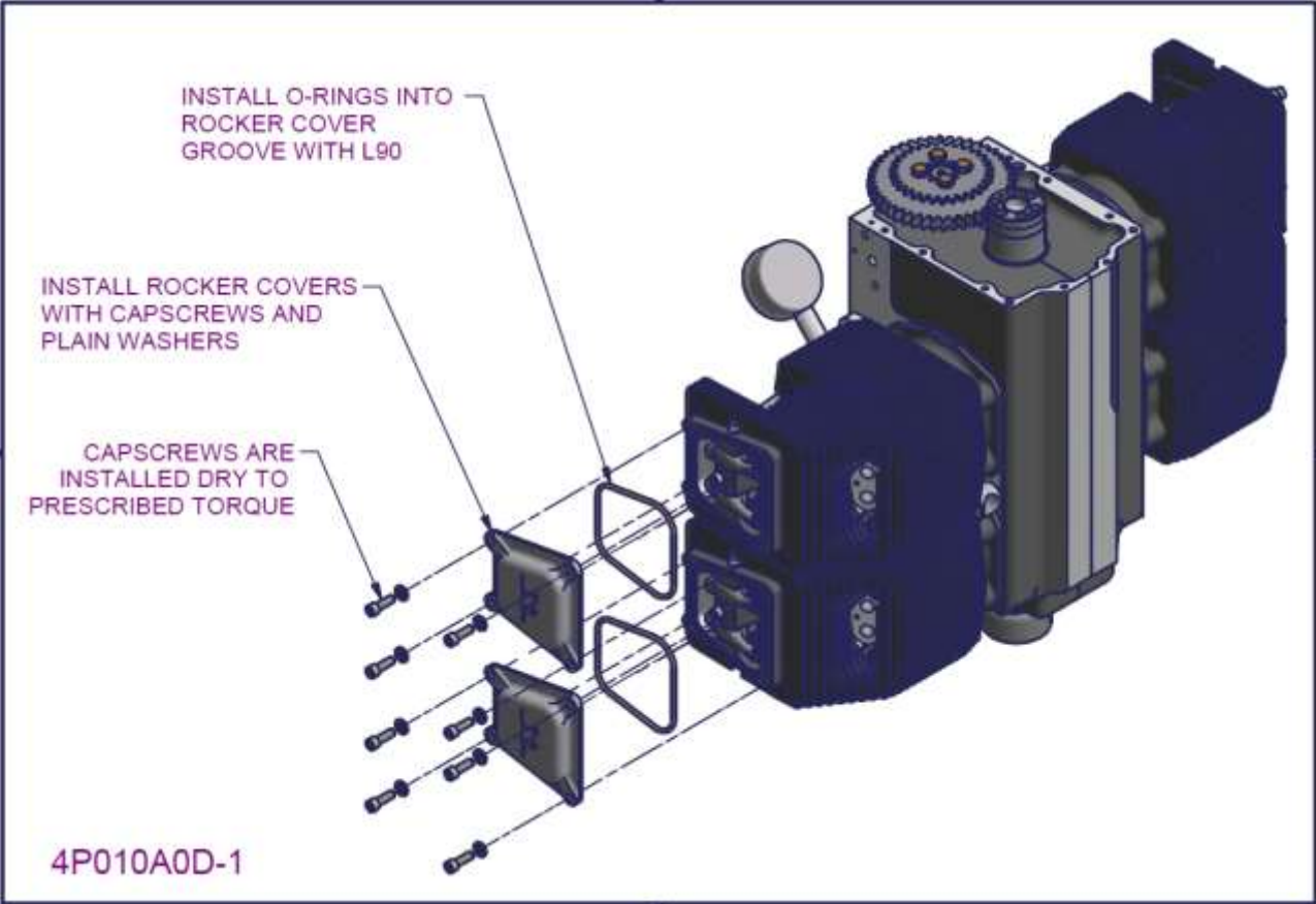
Figure 120 - 2200/3300 Joint engine assembly 6
