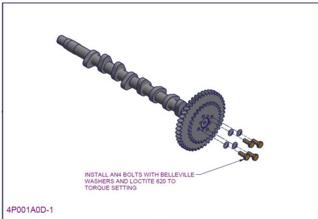
Figure 33 – 2200/3300 camshaft subassembly 2
