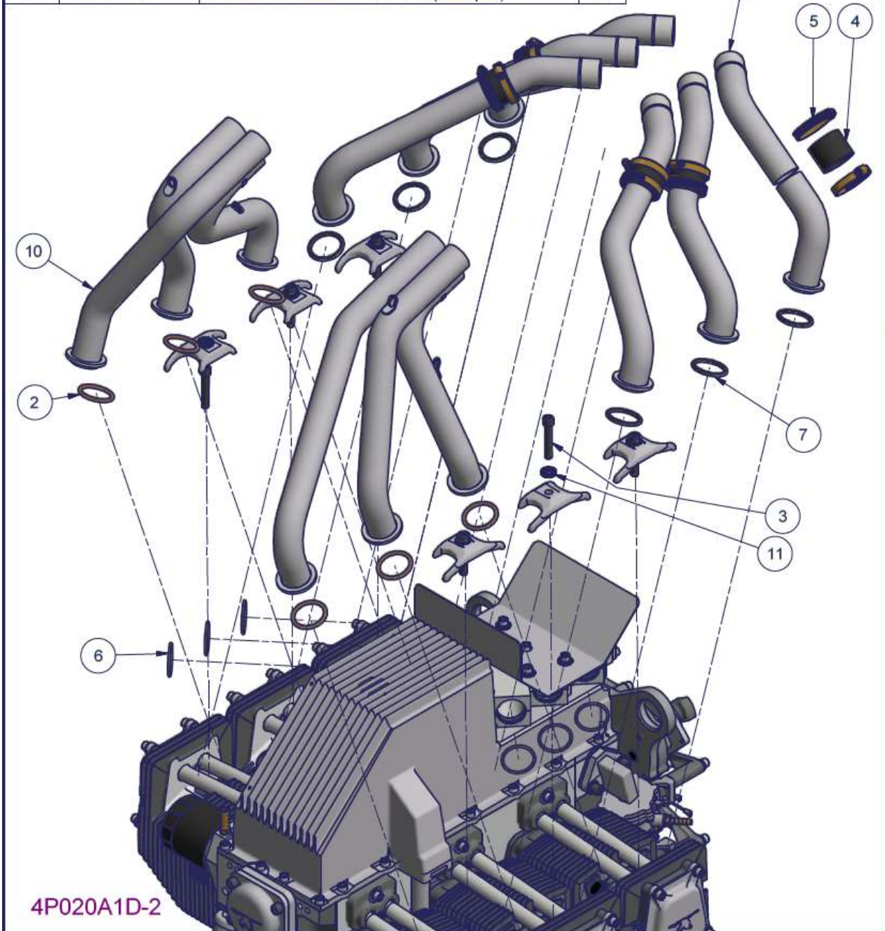
Figure 176 – 3300 Exhaust and induction pipe installation
