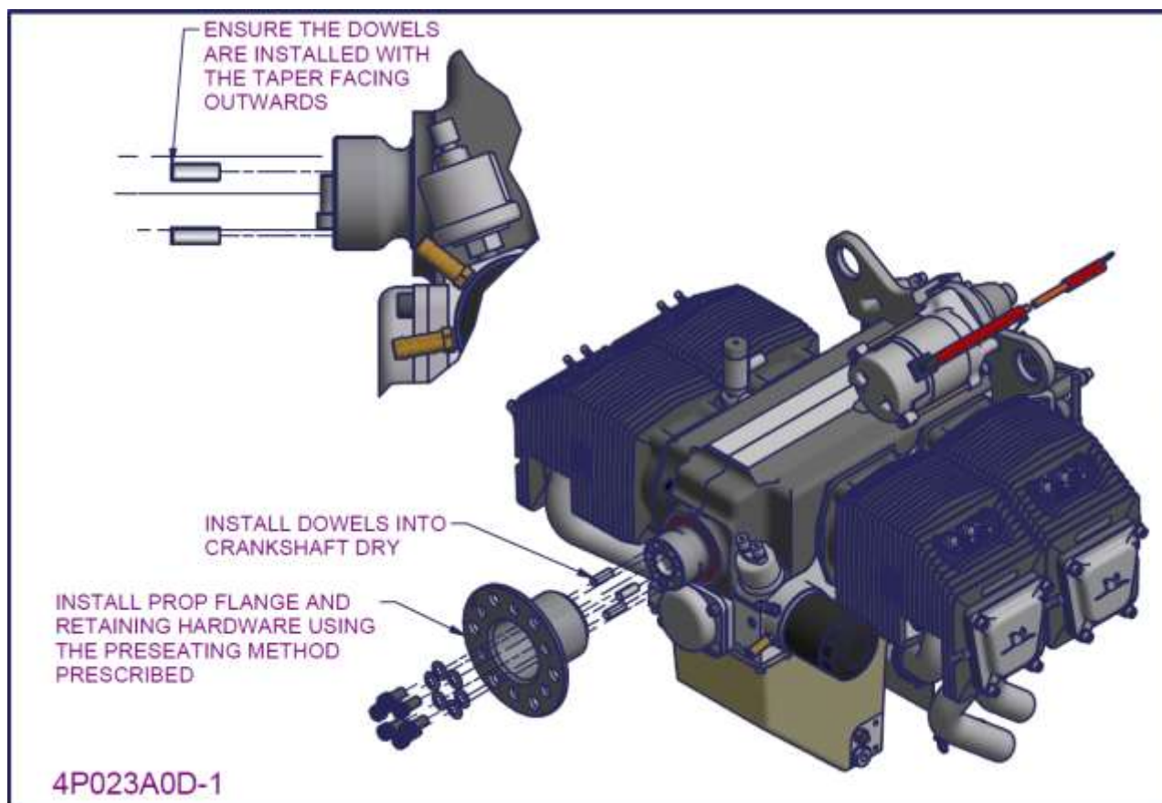
Figure 202 – 2200/3300 Front seal and propeller flange installation 3
