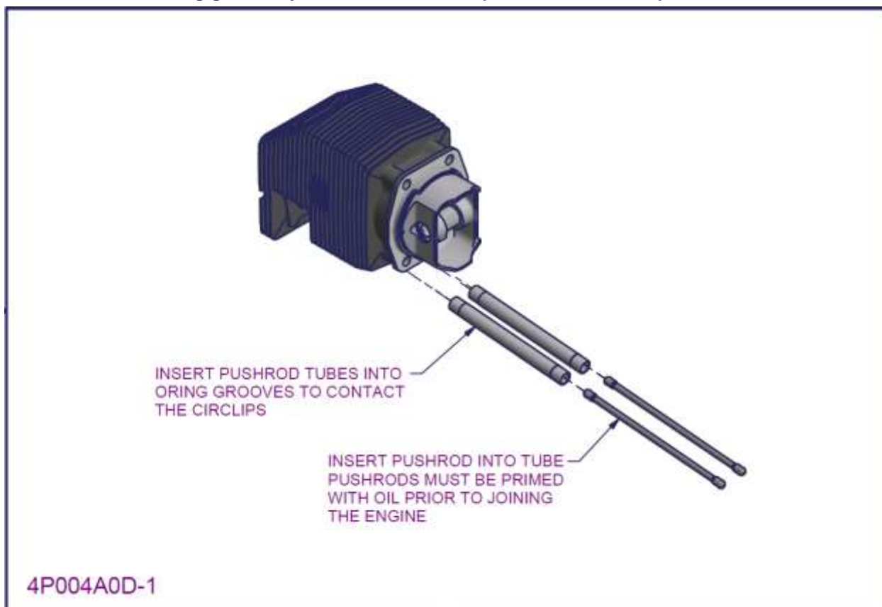
Figure 70 - 2200/3300 cylinder assembly 10b (Internal O-ring groove cylinder head)
