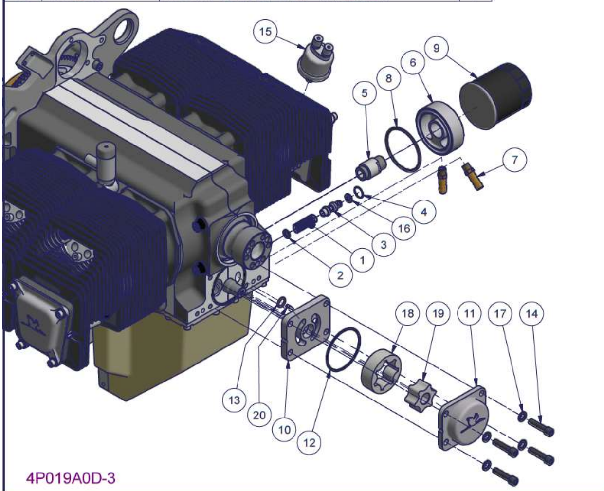
Figure 164 – 2200/3300 Oil pump and filter installation – Parts List
