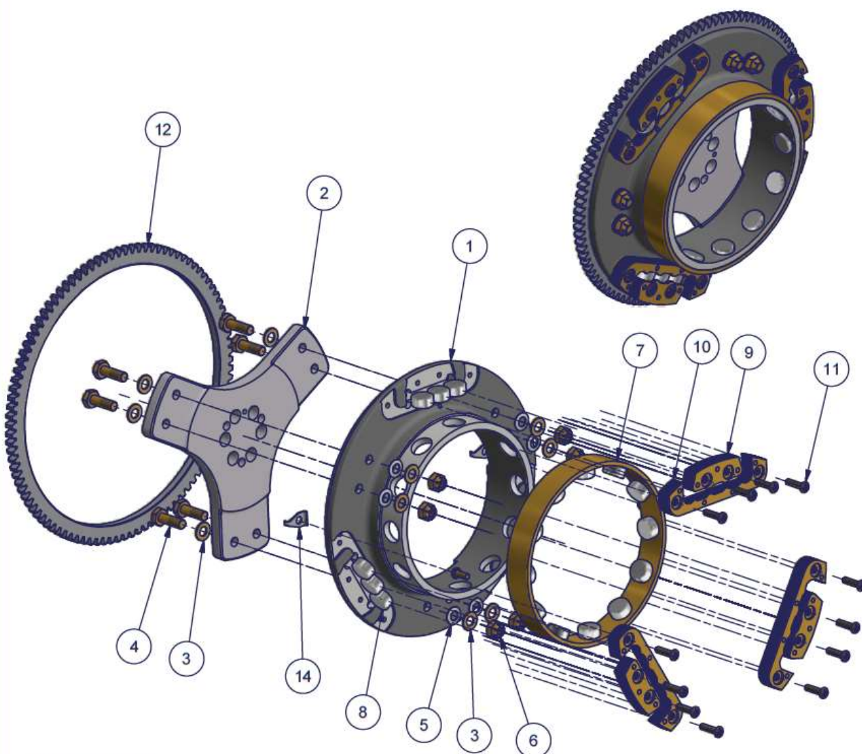
Figure 87 - 3300 flywheel subassembly (aluminium cross piece) - Parts list
