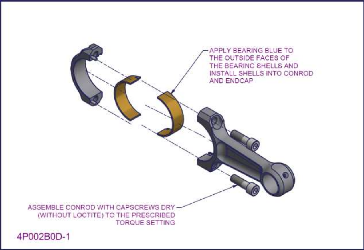
Figure 39 - 2200/3300 crankshaft subassembly 3
