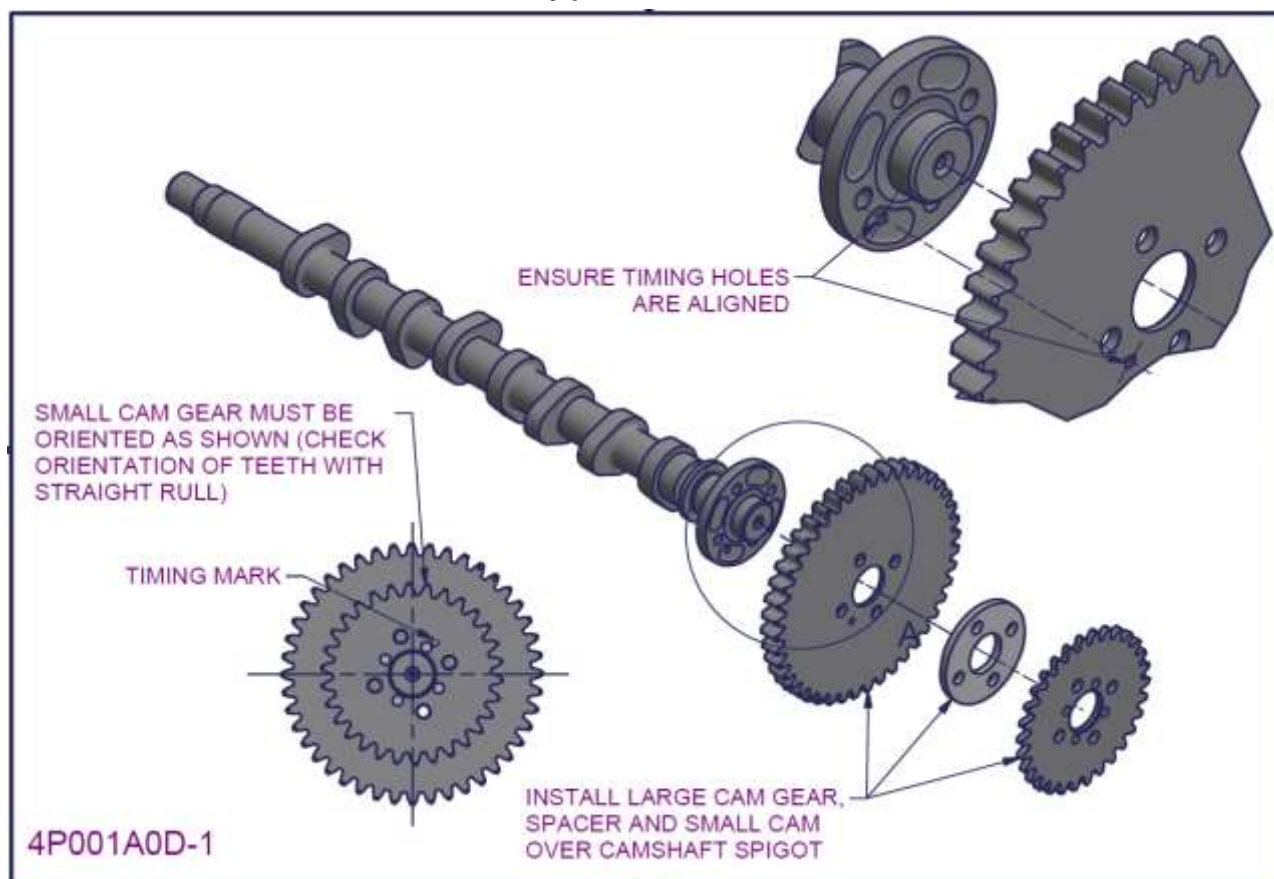
Figure 31 – 2200/3300 camshaft subassembly 1
