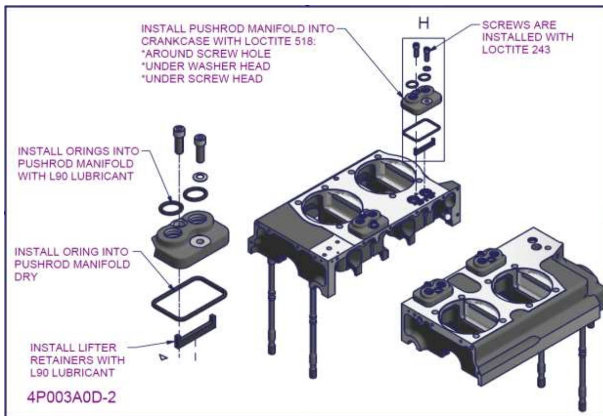
Figure 24 – 2200/330 crankcase subassembly 9
