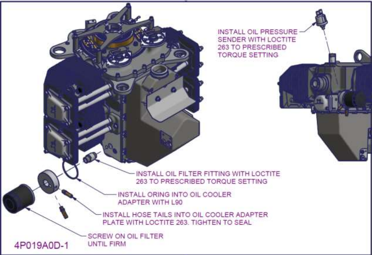
Figure 173 – 2200/3300 Oil pump and filter installation 3
