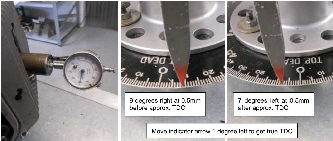
Figure 124 - Locating true TDC
