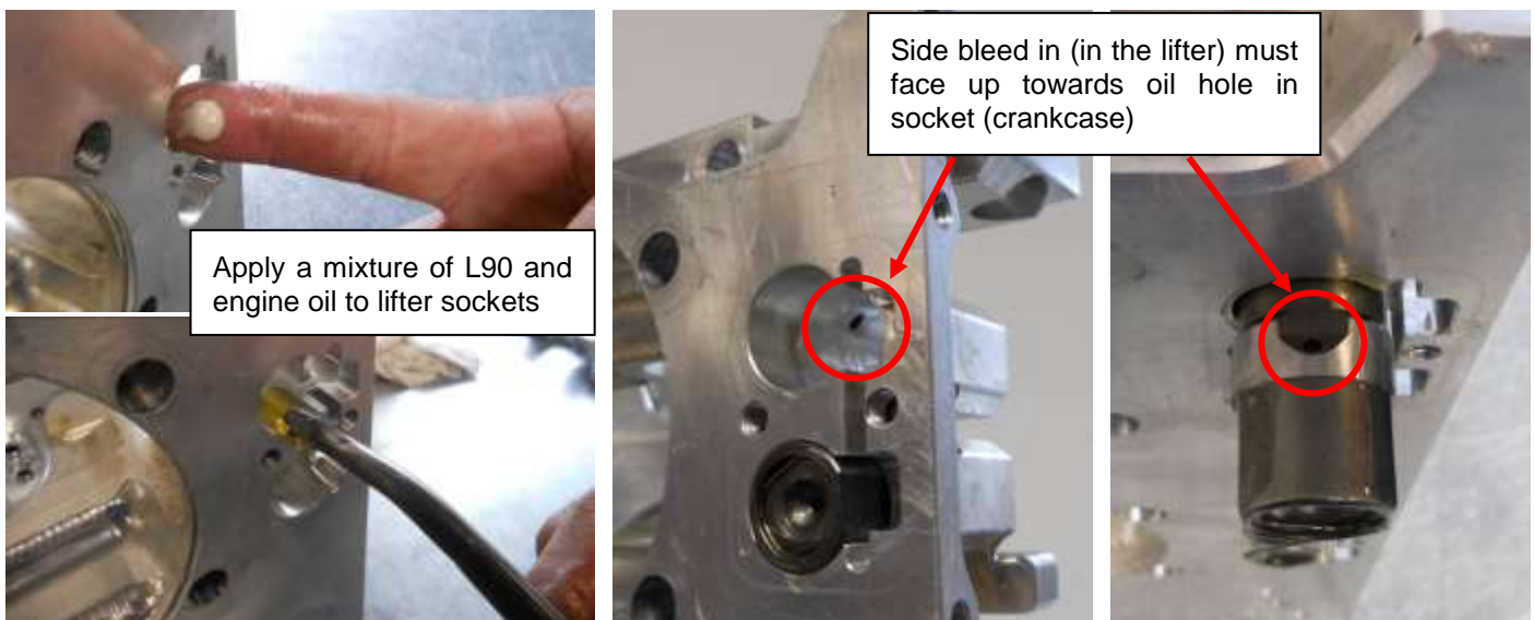
Figure 23 - Roller hydraulic lifter installation
