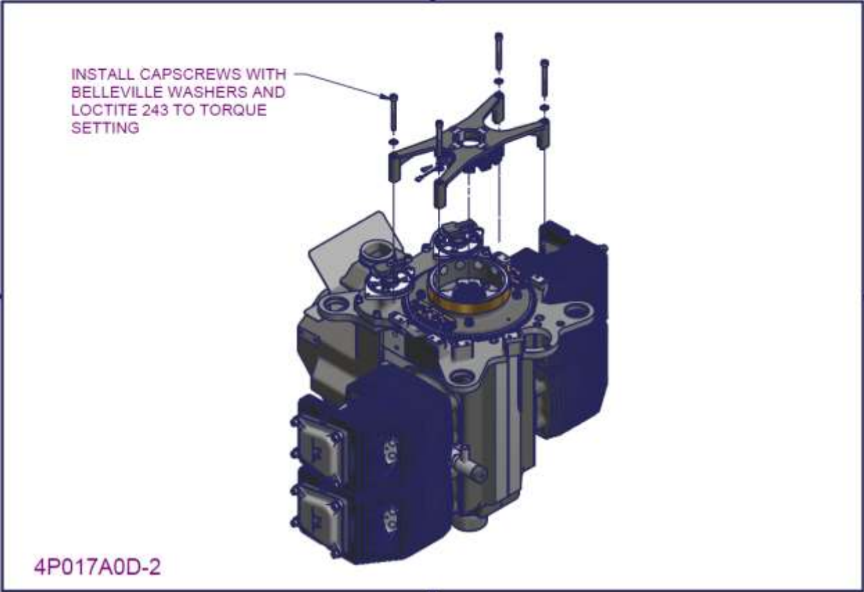
Figure 156 – 2200/3300 flywheel and alternator installation 2
