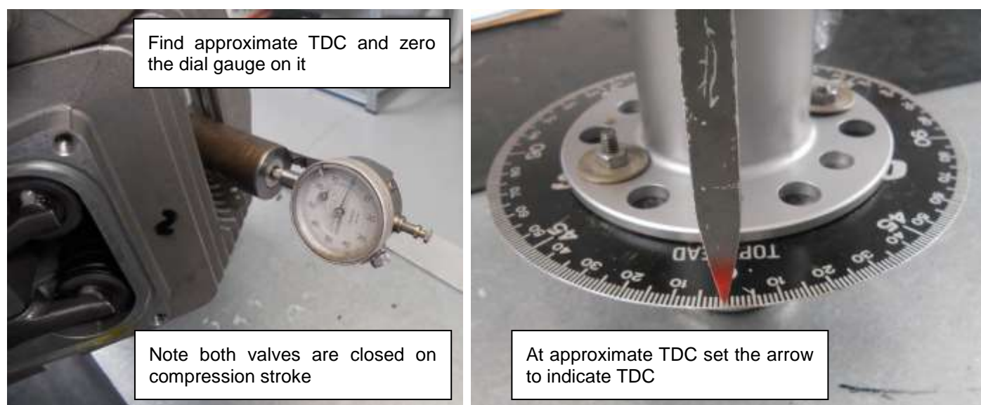
Figure 123 - set dial gauge and arrow indicator at approximate TDC
