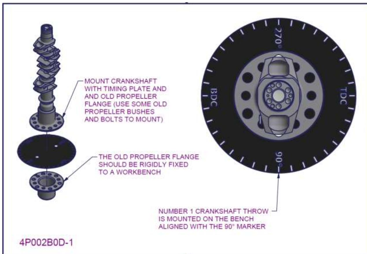
Figure 46 – 2200/3300 crankshaft subassembly 6
