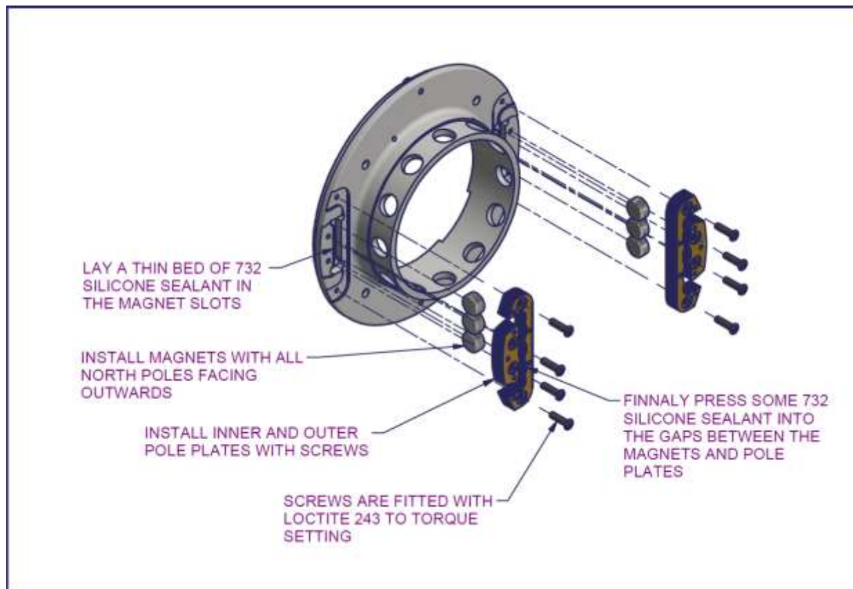
Figure 89 – 2200/3300 Flywheel subassembly (aluminium cross piece) 1
