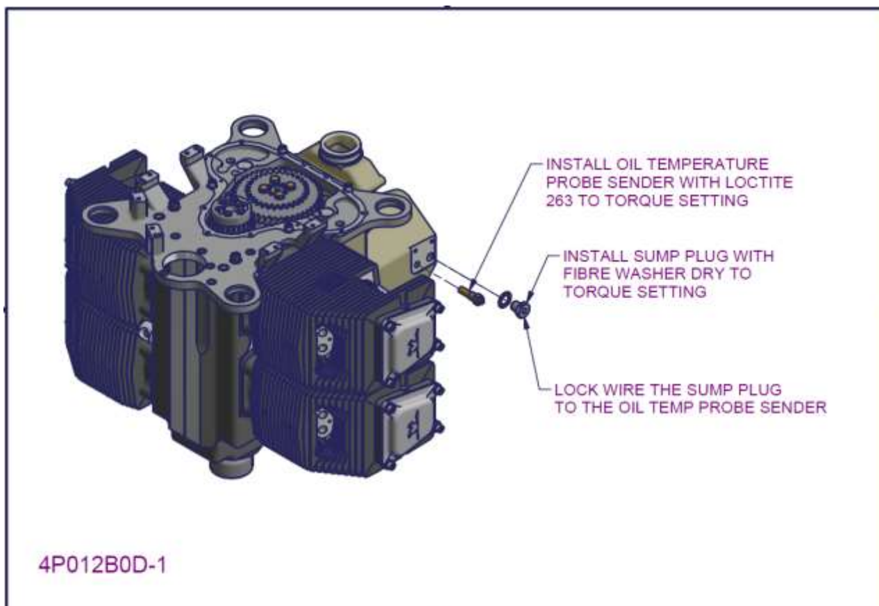
Figure 135 – 2200/3300 Sump installation 3
