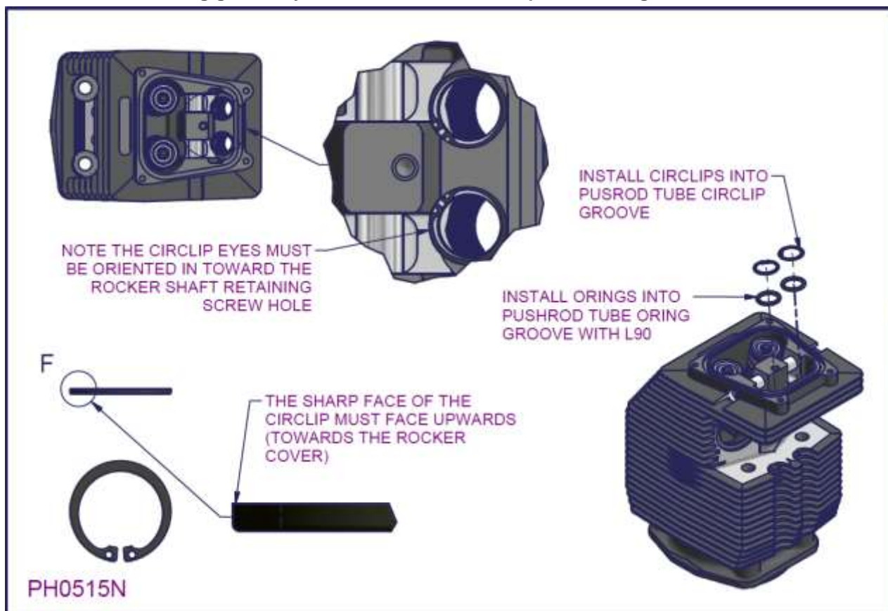
Figure 60 – 2200/3300 cylinder assembly 5b (Internal O-ring groove cylinder head)
