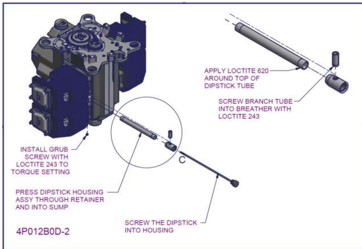
Figure 137 – 2200/3300 Sump installation 4
