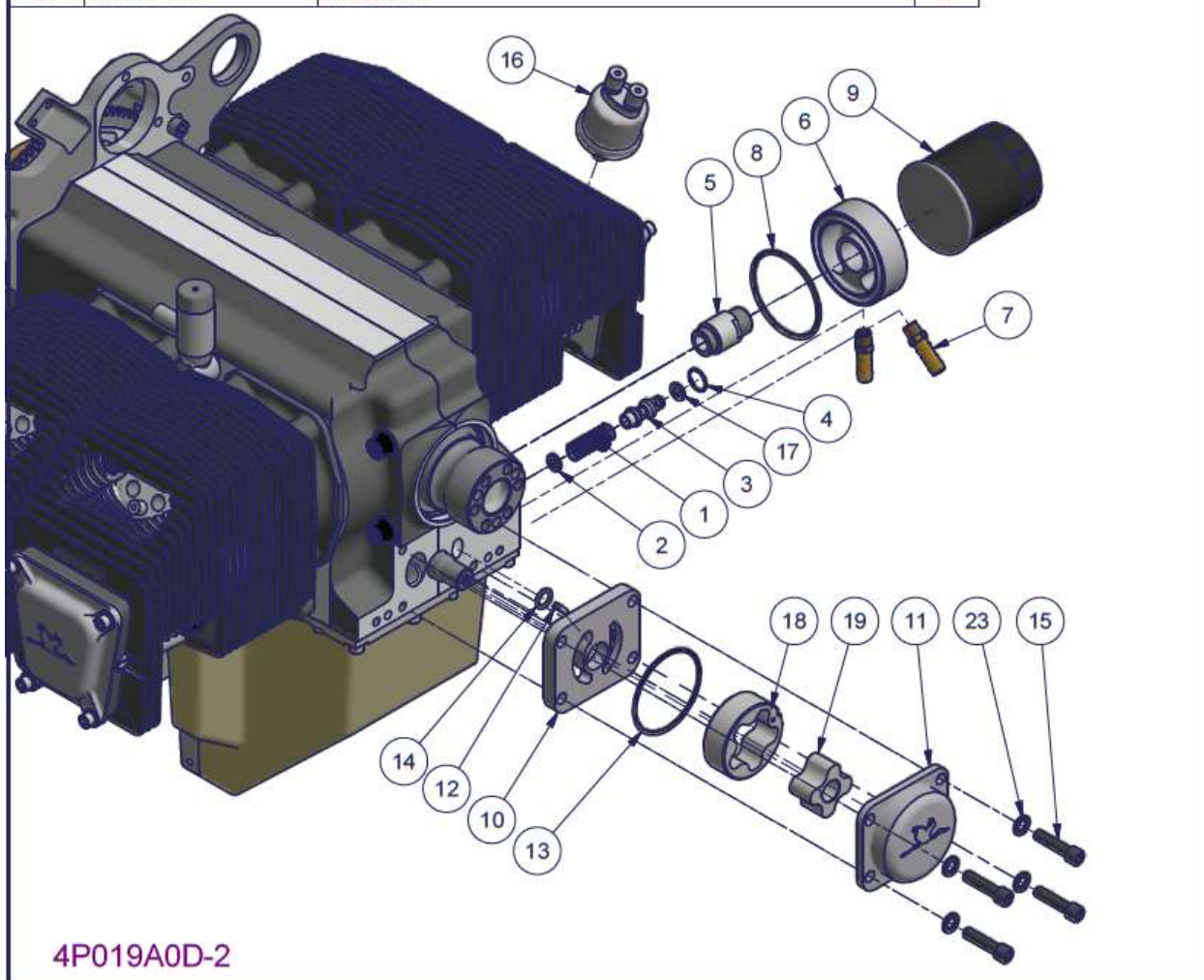
Figure 165 – 2200/3300 Oil pump and filter installation – Parts List
