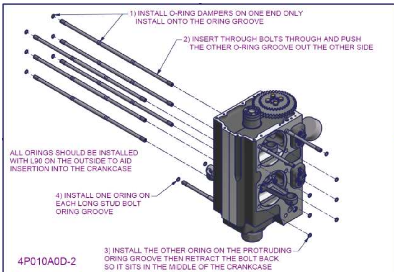
Figure 112 - 2200/3300 Joint engine assembly 2
