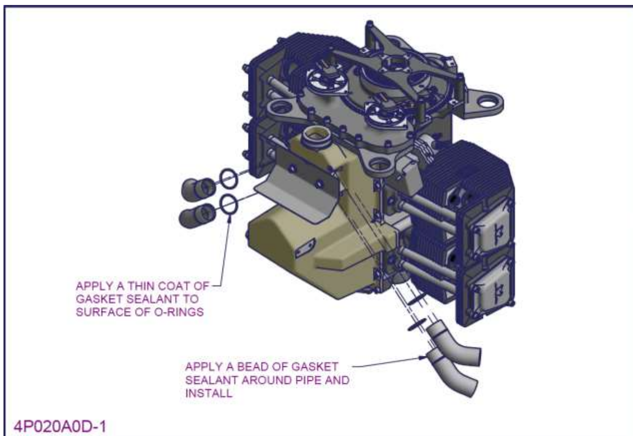
Figure 178 – 2200/3300 Exhaust and induction pipe installation 2
