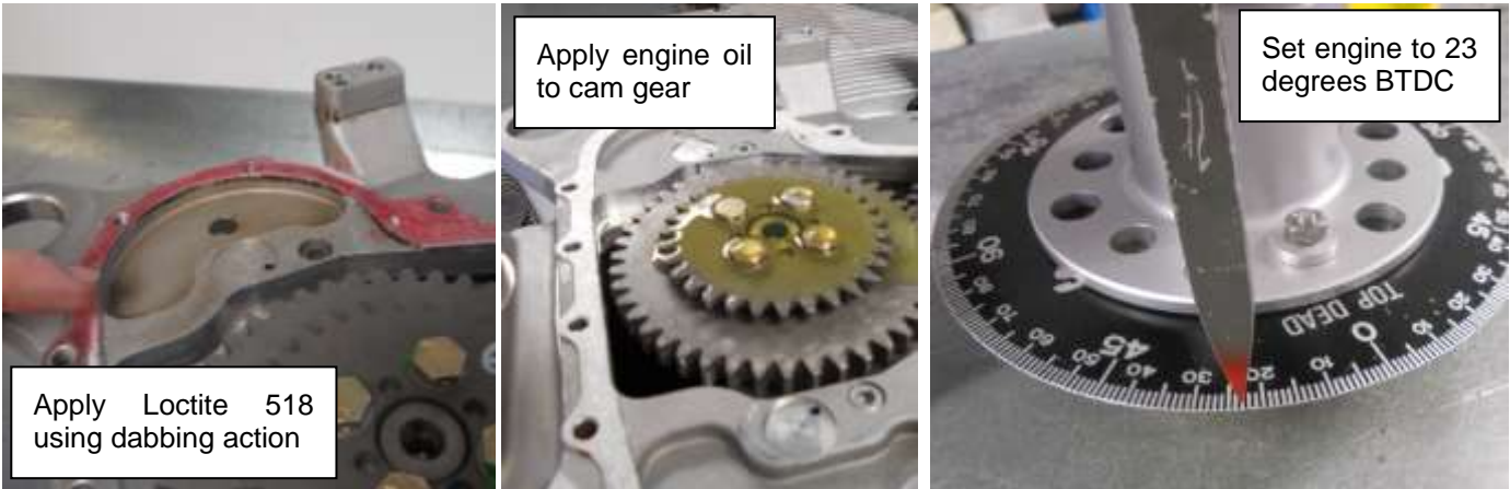
Figure 150 - Distributor gearbox installation
