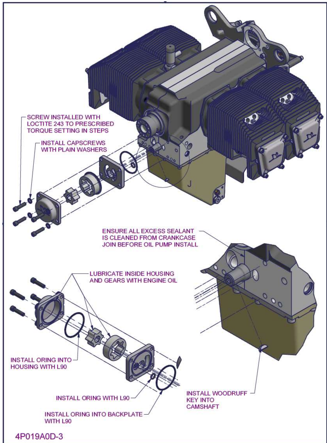
Figure 170 –2200/3300 Oil pump and filter installation 1B
