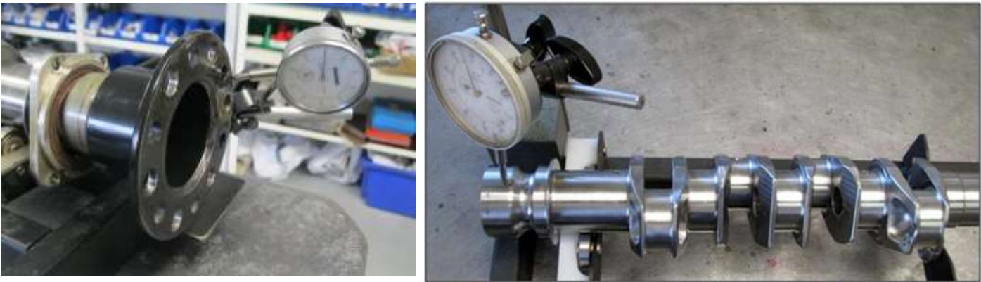
Figure 38 - Measuring propeller flange and crankshaft runout
