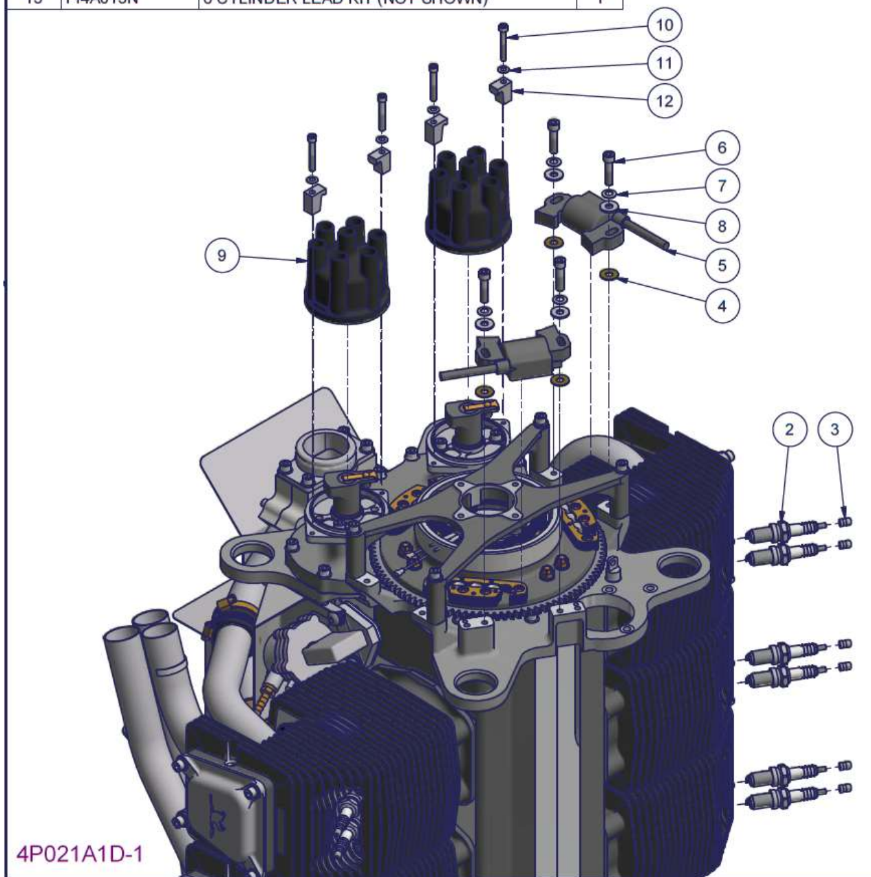
Figure 185 – 3300 Ignition system installation – Parts List
