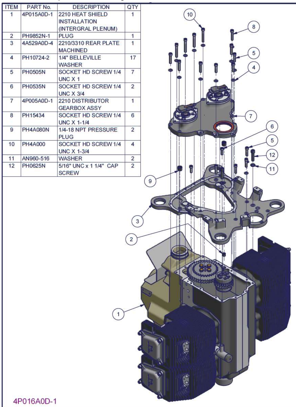
Figure 144 – 2200 back plate and distributor gearbox installation – Parts List
