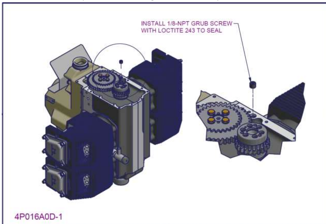
Figure 146 – 2200/3300 back plate and distributor gearbox installation 1
