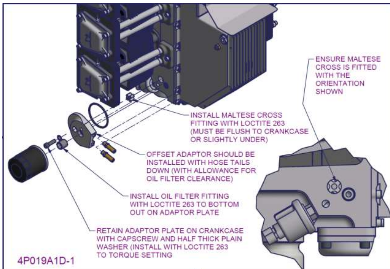
Figure 174 – Reworked Billet crankcase oil filter adaptor installation
