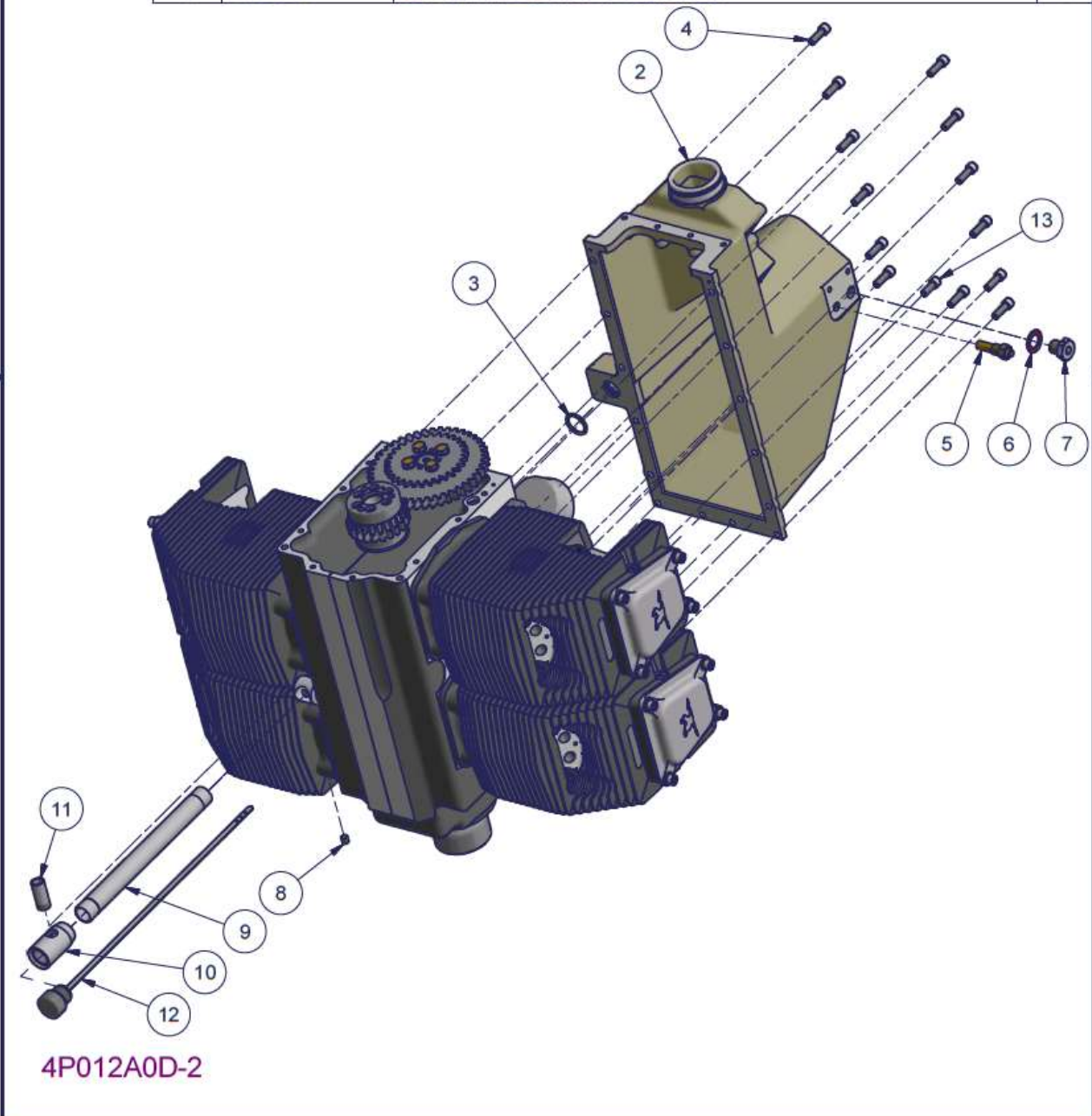
Figure 128 – 2200 Sump installation (integral plenum) – Parts List
