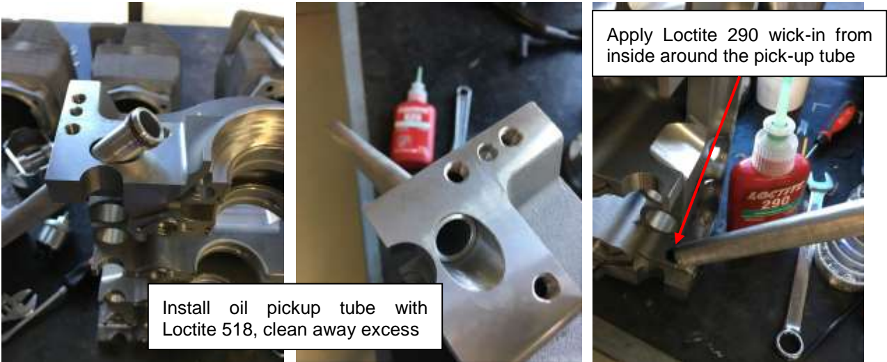
Figure 27 - Oil pickup tube installation
