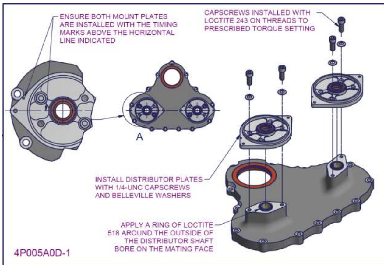
Figure 78 – 2200/3300 Distributor gearbox subassembly 3
