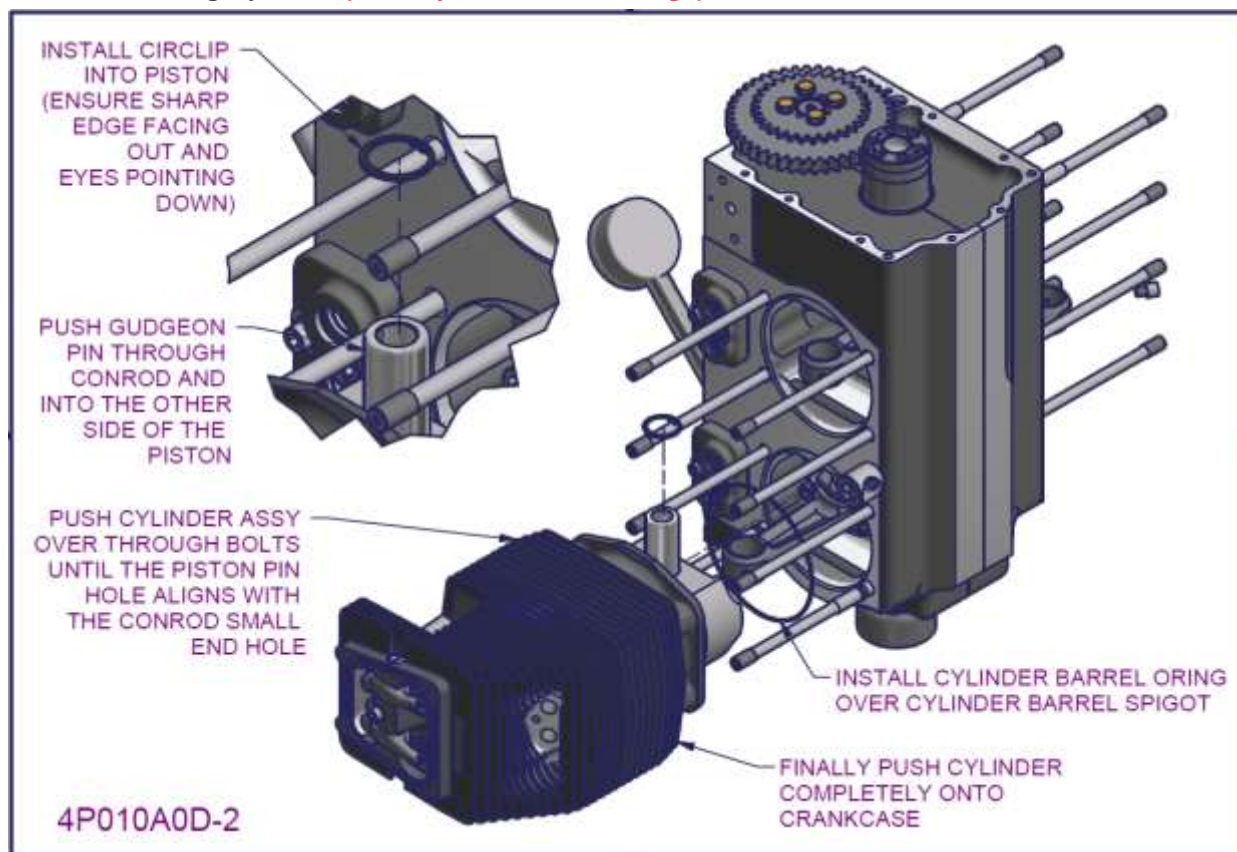
Figure 115 - 2200/3300 Joint engine assembly 3B
