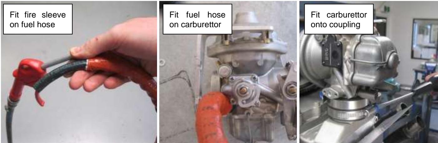
Figure 196 – Carburettor installation
