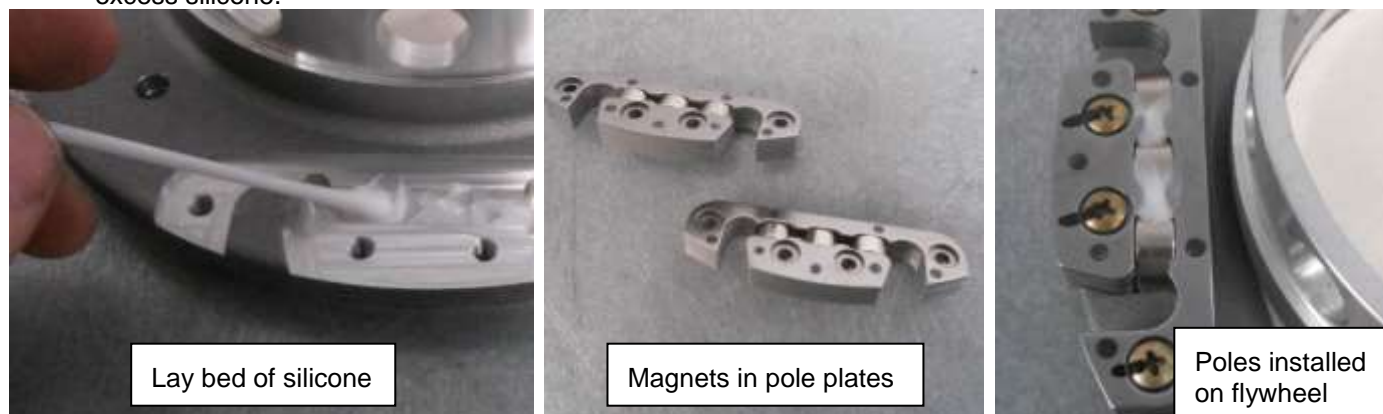
Figure 90 - Flywheel ignition magnets and pole plate installation
