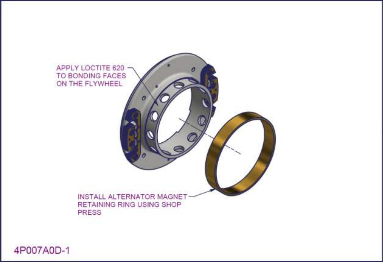
Figure 91 - 2200/3300 Flywheel subassembly (aluminium cross piece) 2
