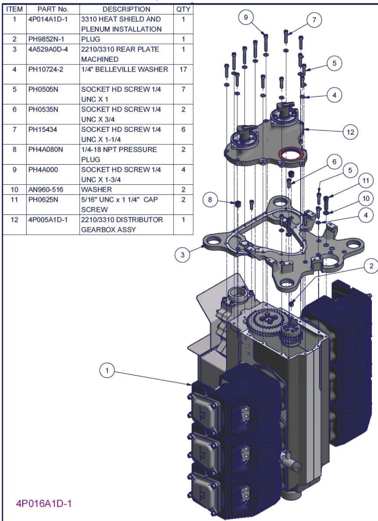
Figure 145 – 3300 back plate and distributor gearbox installation – Parts List
