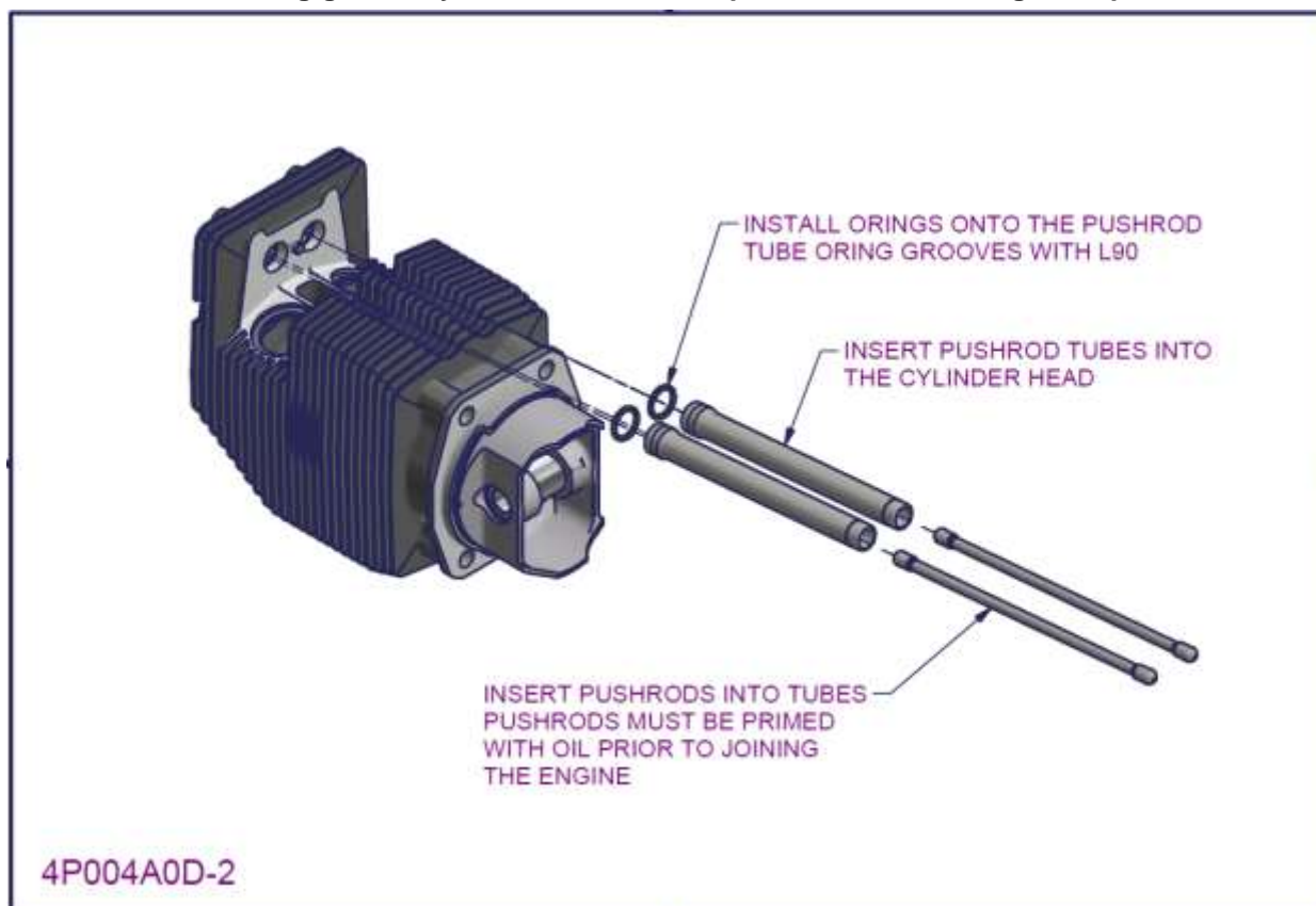
Figure 69 - 2200/3300 cylinder assembly 10a (external O-ring groove cylinder head)
