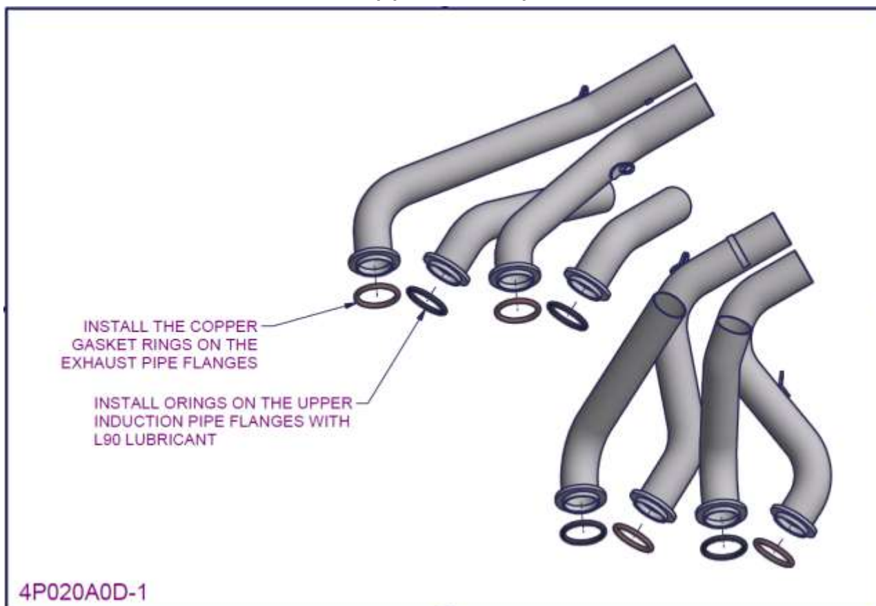
Figure 177 – 2200/3300 Exhaust and induction pipe installation 1
