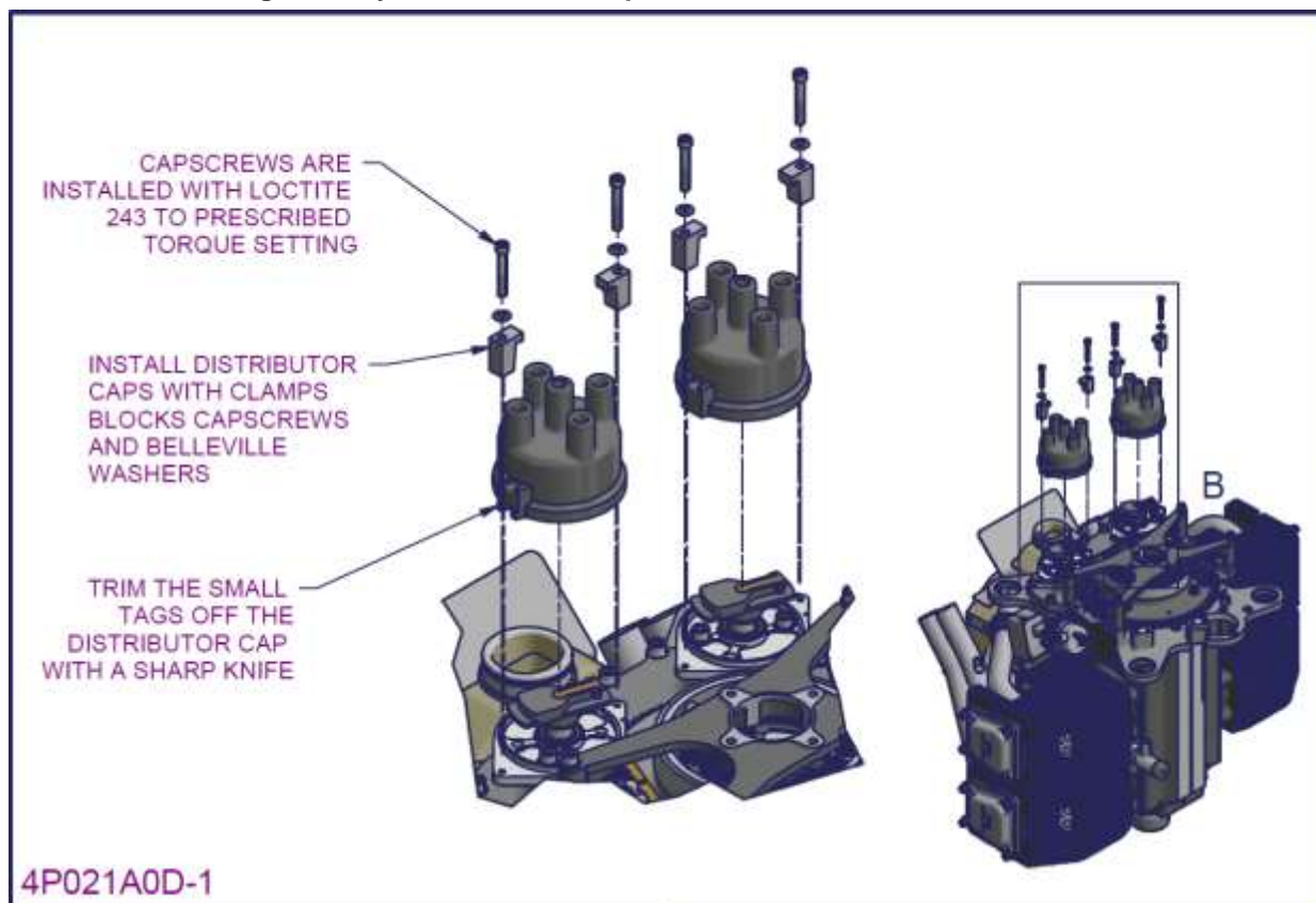
Figure 186 – 2200/3300 Ignition system installation 1
