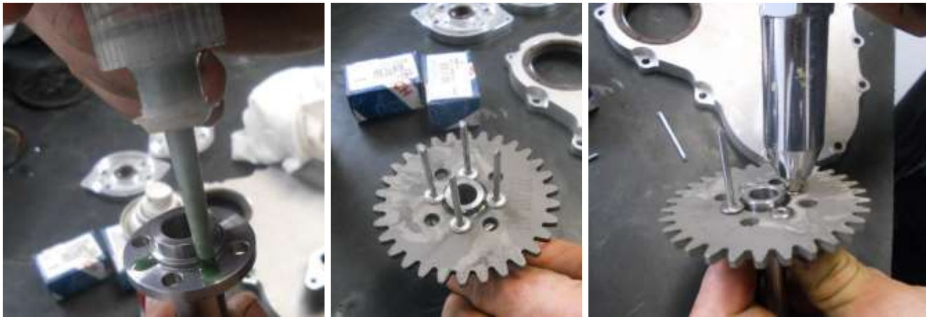
Figure 81 - Rotor shaft assembly
