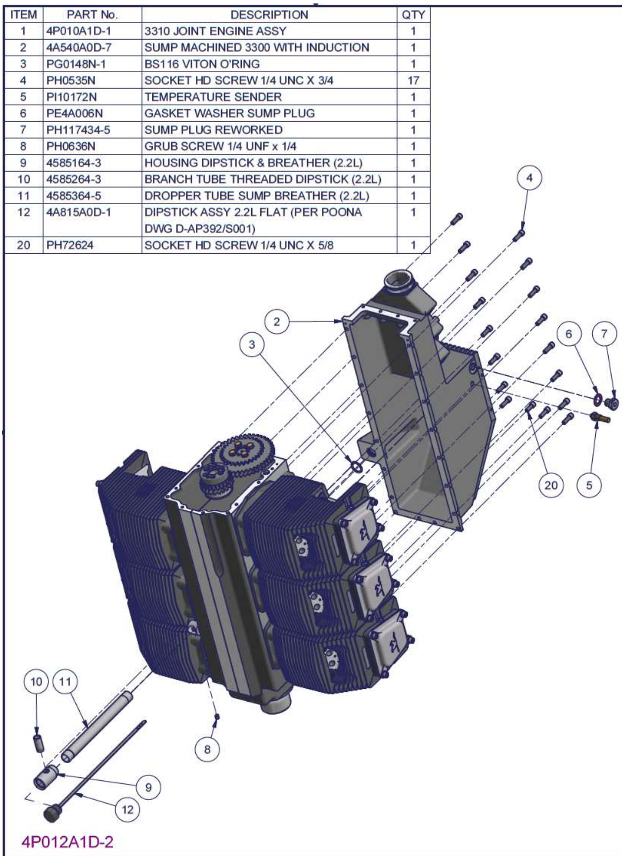
Figure 130 – 3300 Sump installation (integral plenum) – Parts List
