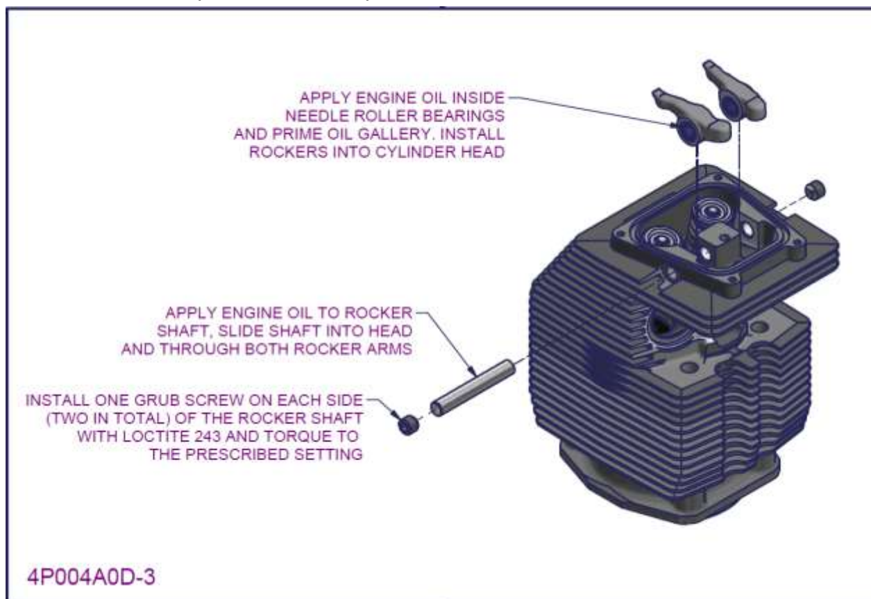
Figure 61 – 2200/3300 cylinder assembly 6a (10mm needle roller rocker shaft cylinder head)
