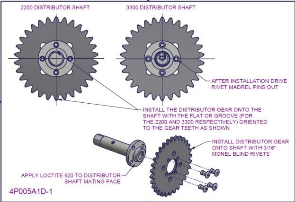
Figure 80 – 2200/3300 Distributor gearbox subassembly 4
