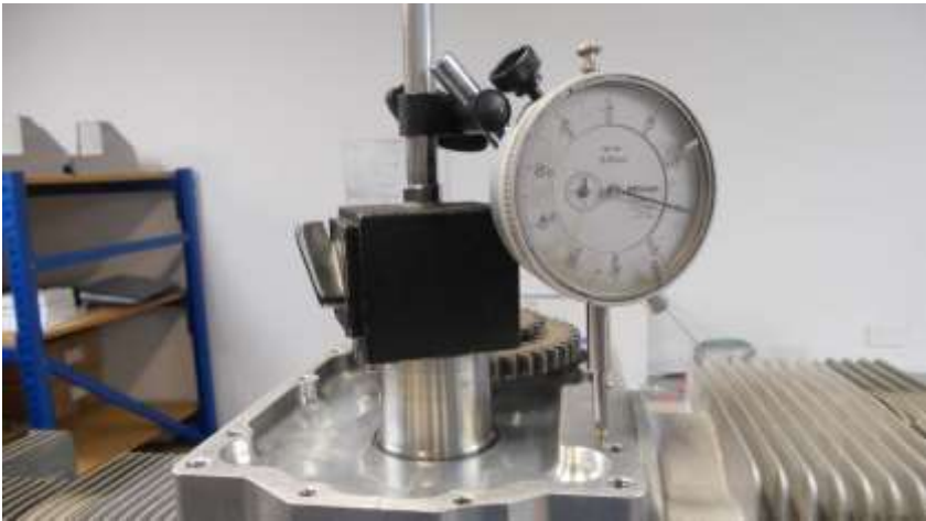
Figure 119 - Verifying end float using a dial gauge
