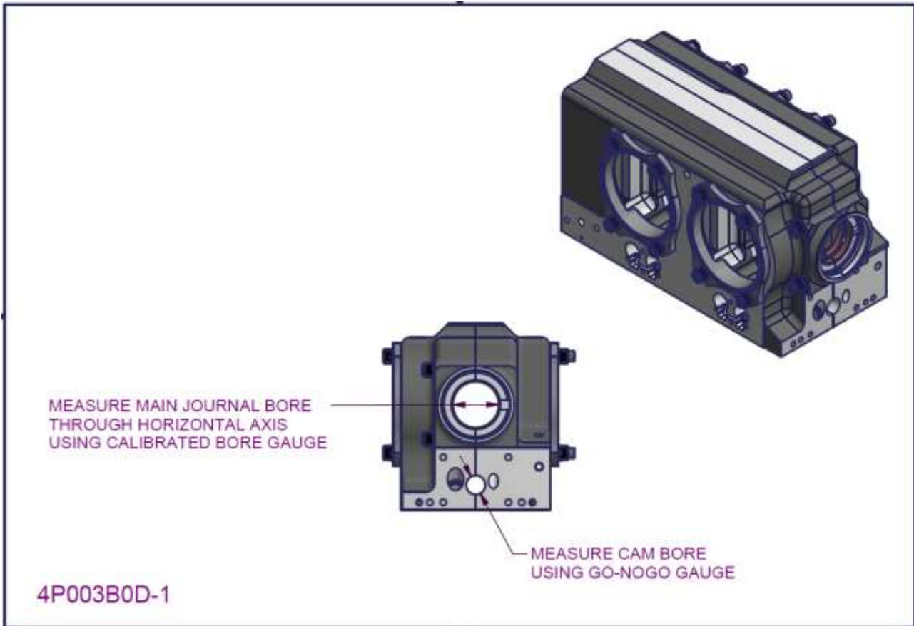
Figure 15 – 2200/330 crankcase subassembly 4
