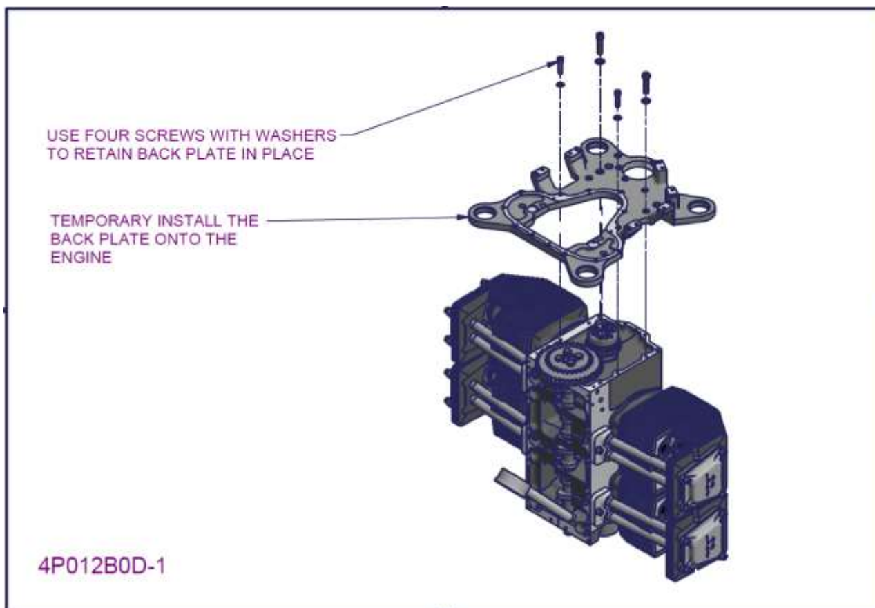
Figure 132 – 2200/3300 Sump installation 1
