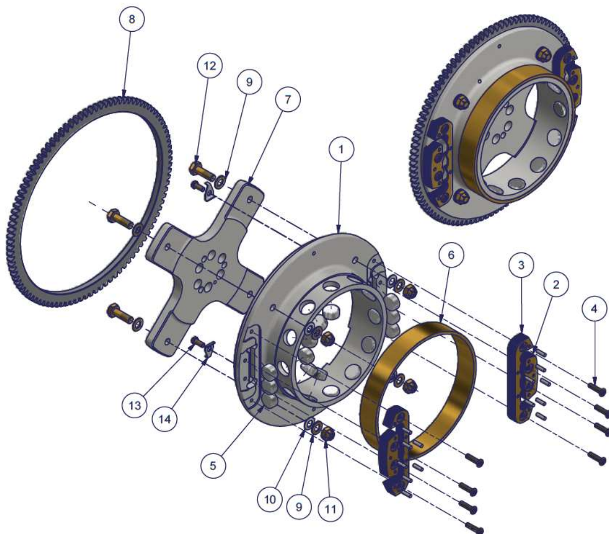
Figure 85 - 2200 Flywheel subassembly (aluminium cross piece) - Parts list
