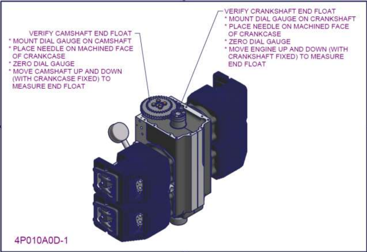
Figure 118 - 2200/3300 Joint engine assembly 5
