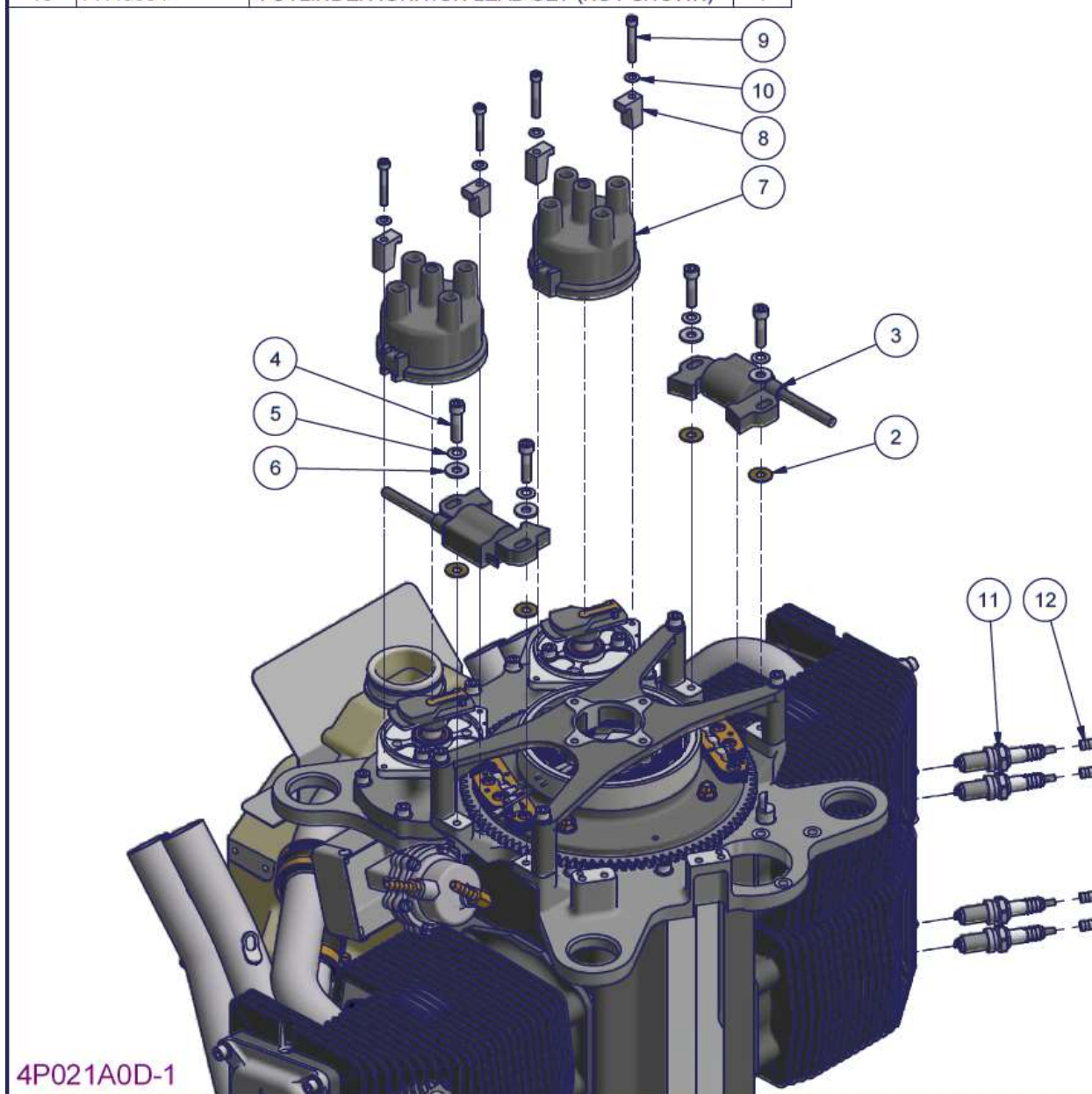
Figure 184 – 2200 Ignition system installation – Parts List
