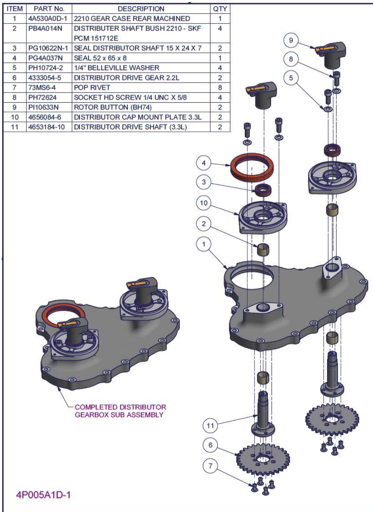
Figure 73 - 3300 Distributor gearbox subassembly - Parts list
