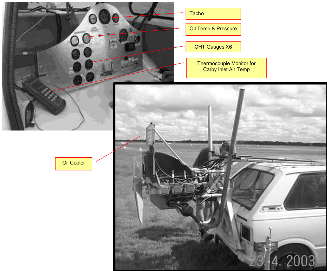
Figure 206 – Engine Ground Running Rig
