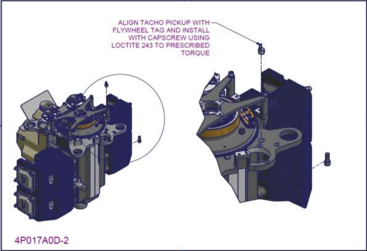
Figure 158 – 2200/3300 flywheel and alternator installation 3
