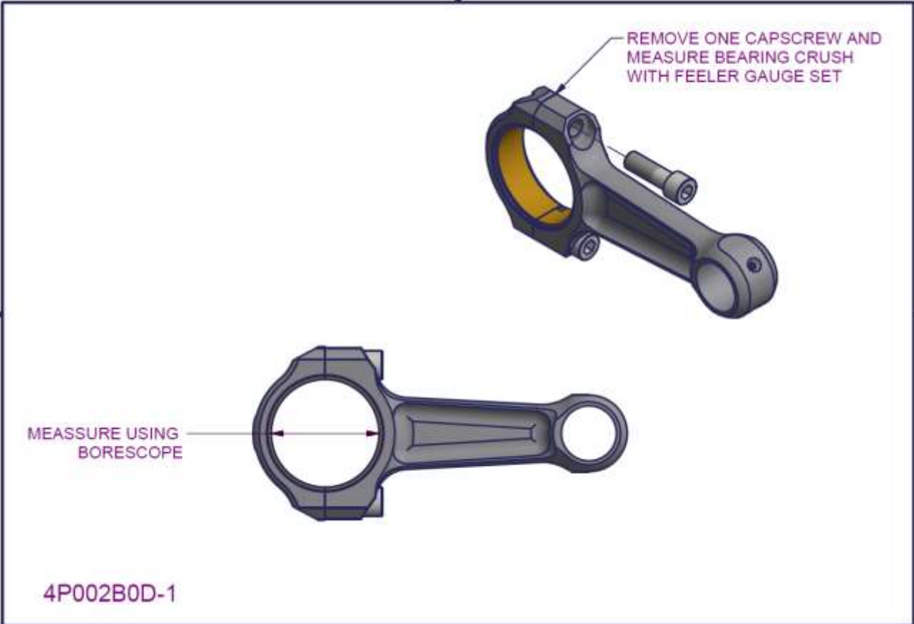
Figure 42 - 2200/3300 crankshaft subassembly 4
