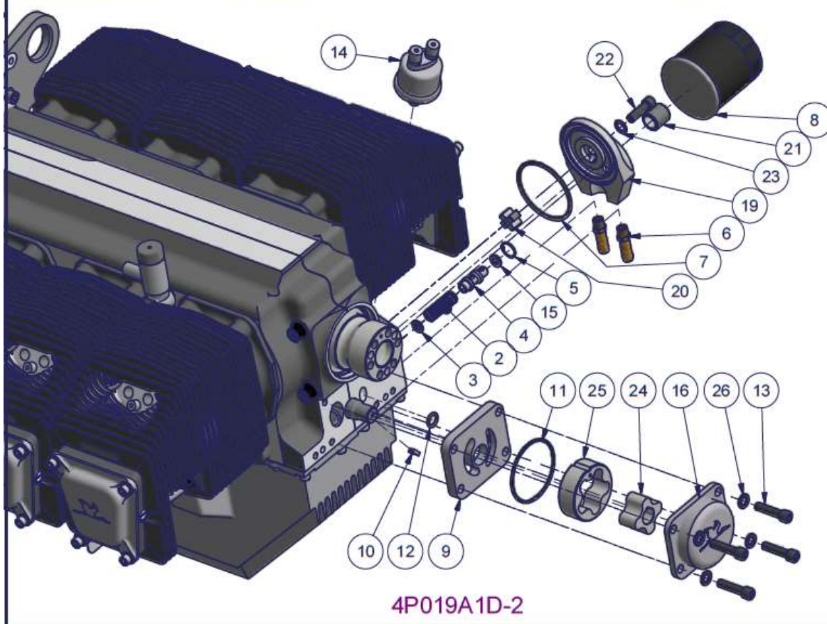
Figure 167 – 3300 Oil pump and filter installation (billet crankcase) – Parts List
