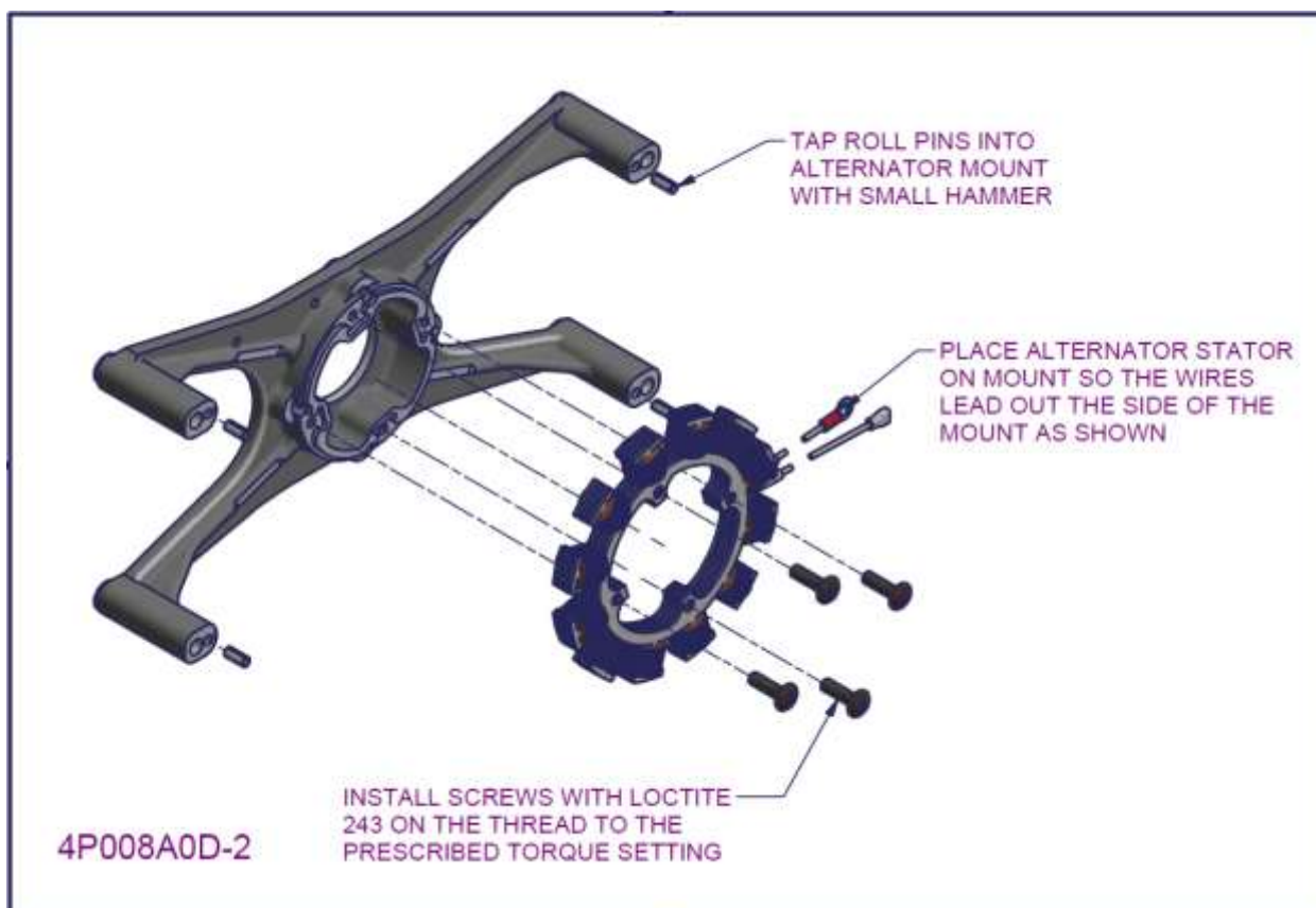
Figure 103 – 2200/ 3300 alternator stator subassembly 1
