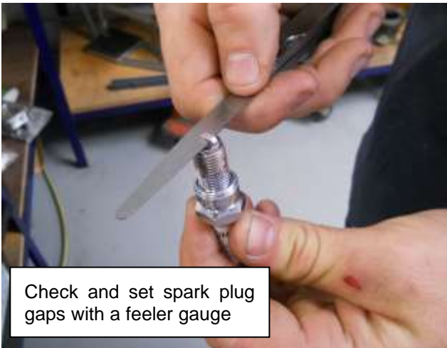
Figure 190 - Checking and setting spark plug gaps
