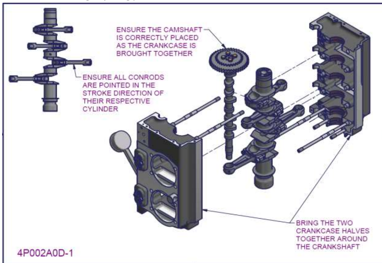
Figure 110 - 2200/3300 Joint engine assembly 1
