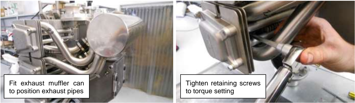
Figure 183 - Pipe positioning and torqueing
