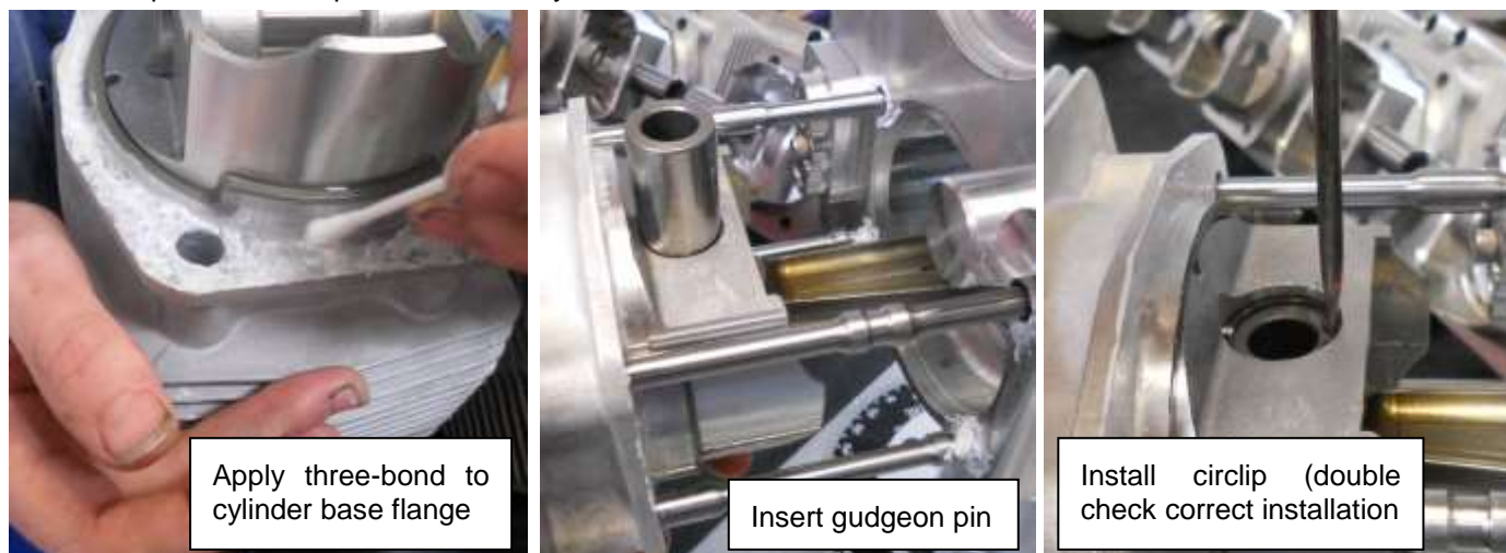
Figure 114 - Cylinder installation
