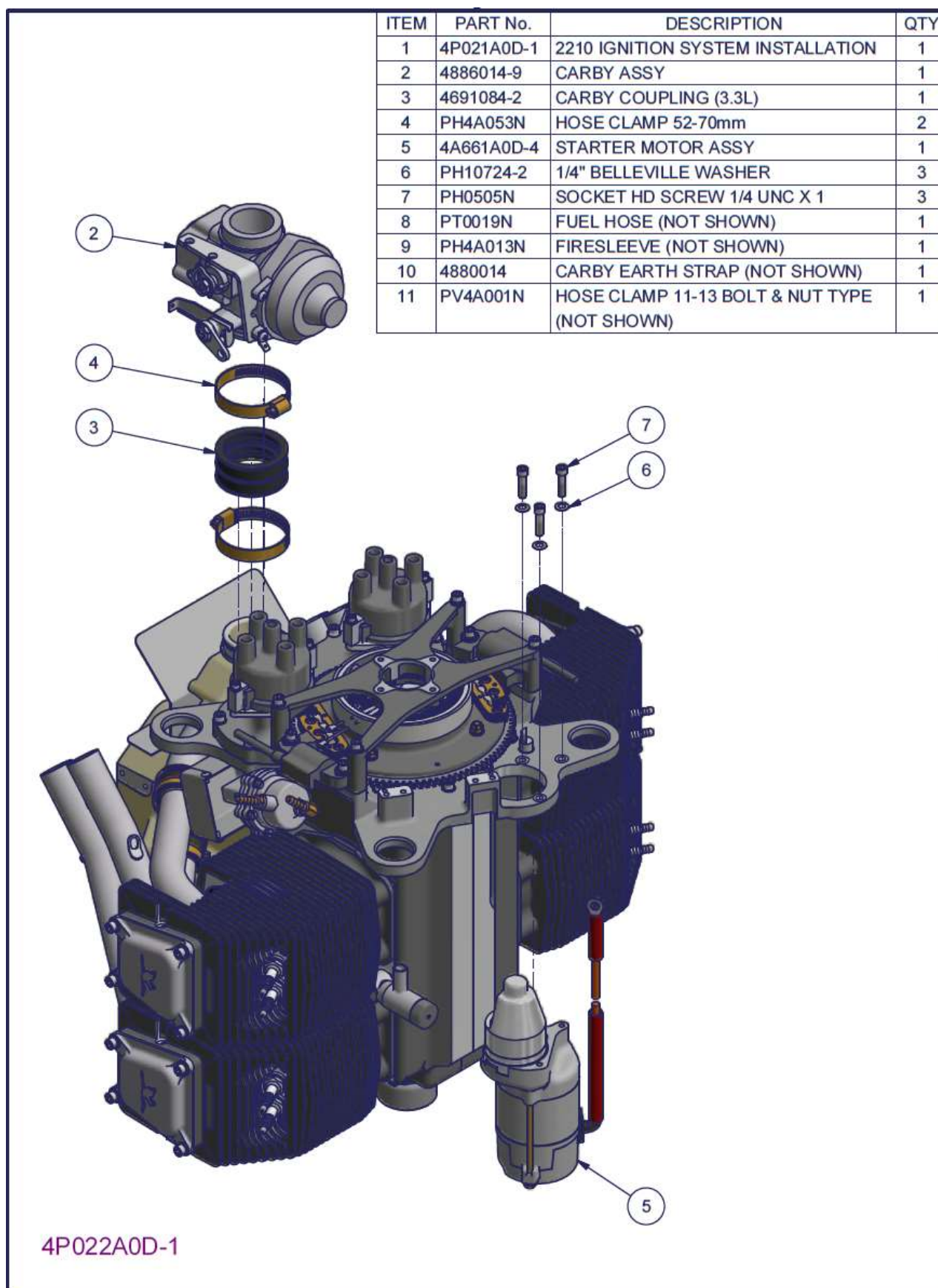
Figure 193 – 2200 Carburettor and Starter installation – Parts List
