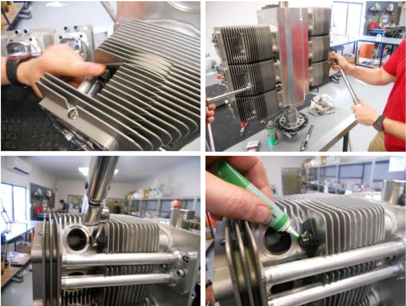
Figure 117 - Installing washers, nuts and tightening to torque
