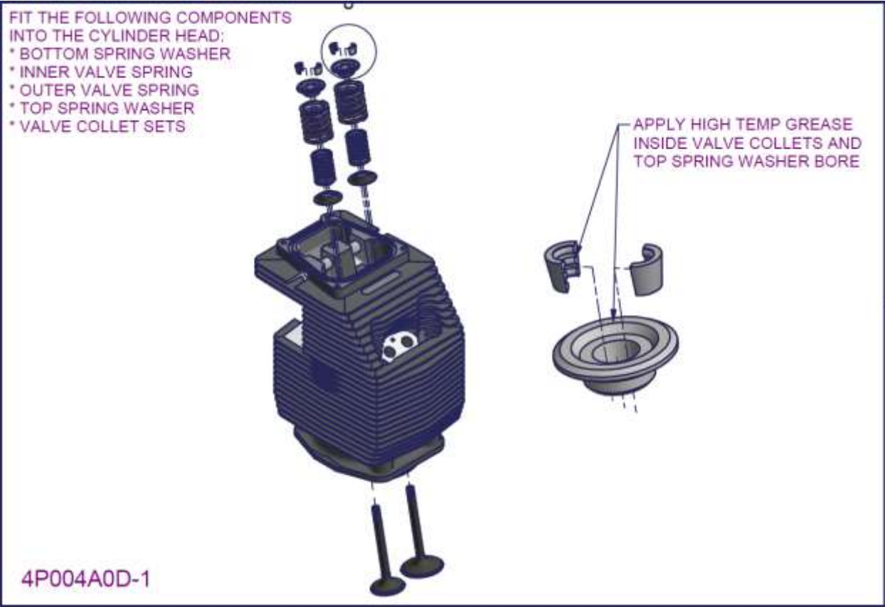
Figure 57 – 2200/3300 cylinder assembly 4
