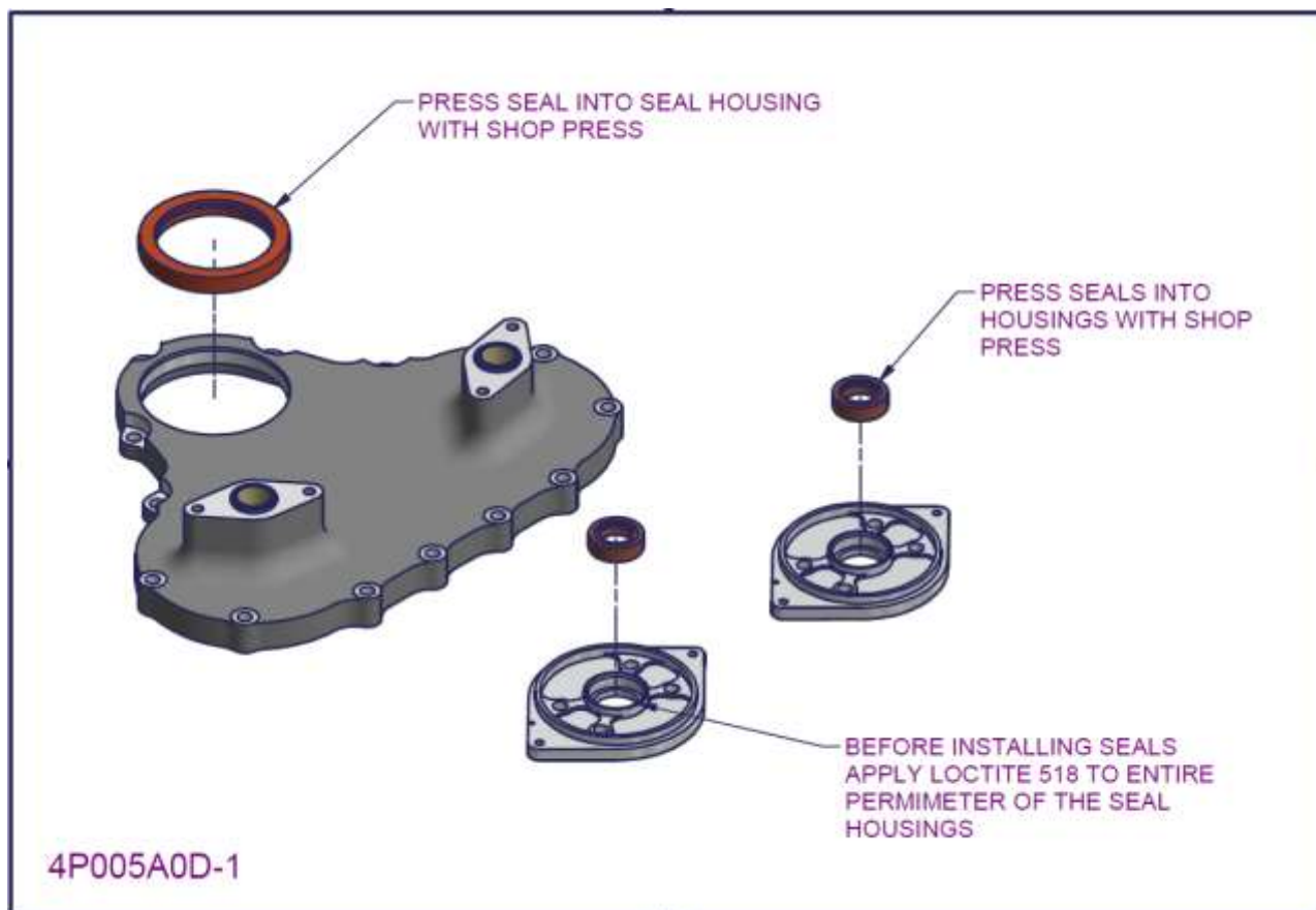
Figure 76 – 2200/3300 Distributor gearbox subassembly 2
