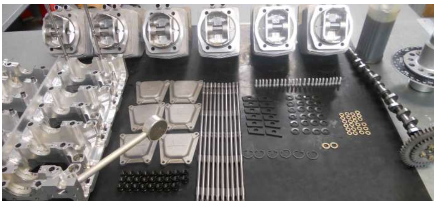
Figure 109 - Engine assemblages, hardware and tools laid out ready to join the engine
