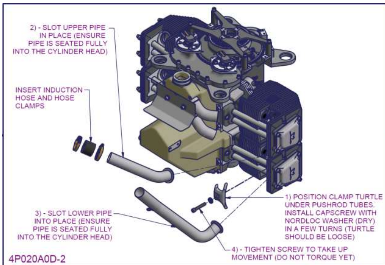
Figure 180 – 2200/3300 Exhaust and induction pipe installation 3
