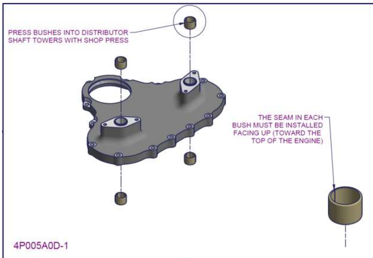
Figure 74 – 2200/3300 Distributor gearbox subassembly 1
