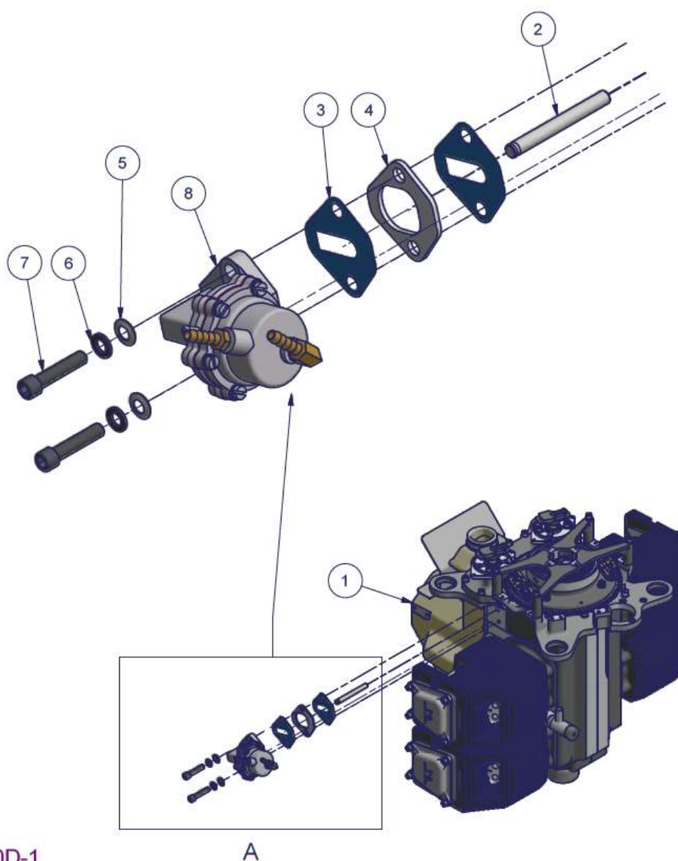
Figure 160 – 2200 Fuel pump installation – Parts List
