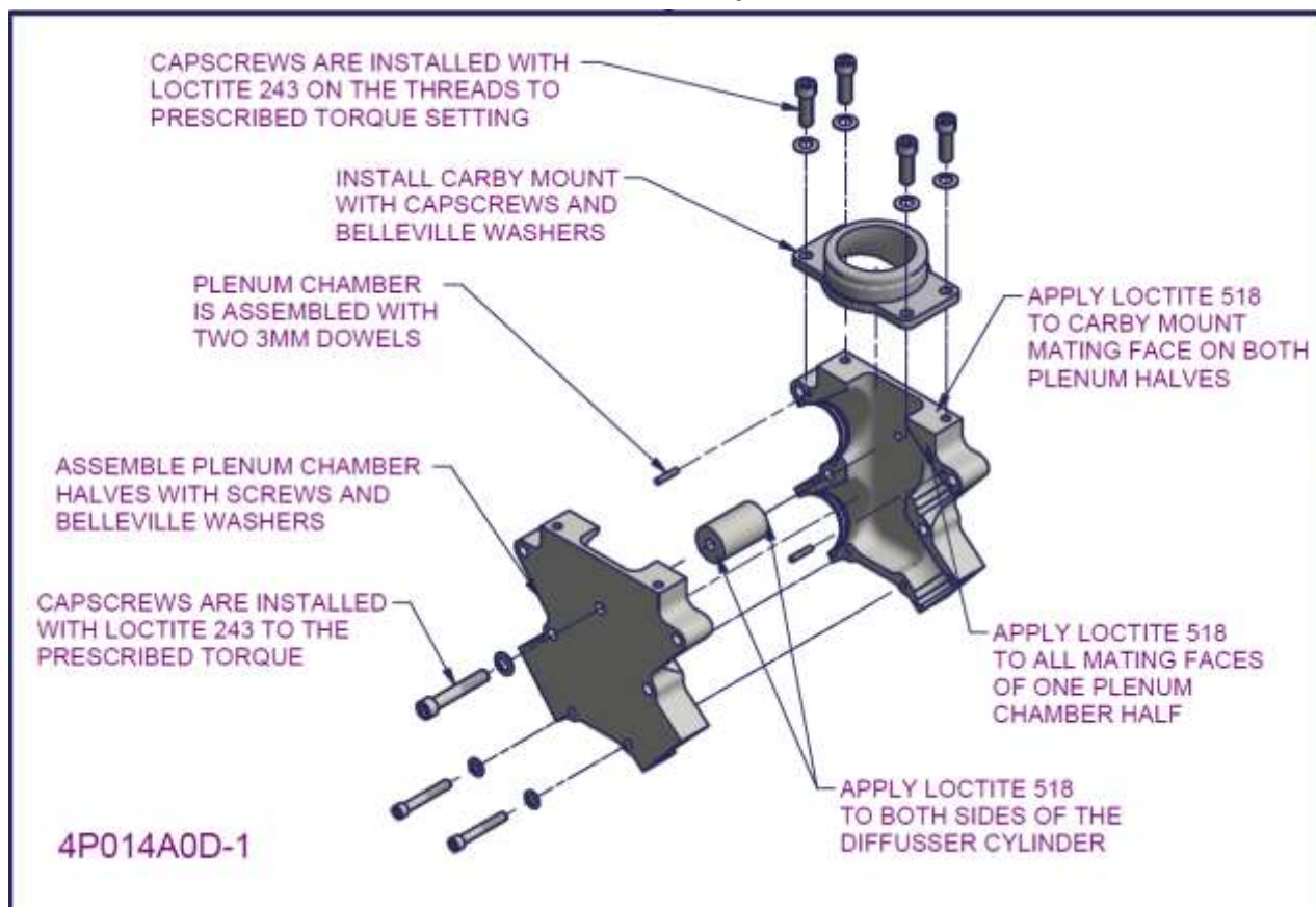
Figure 142 – 2200/3300 Plenum and Heat shield installation 1
