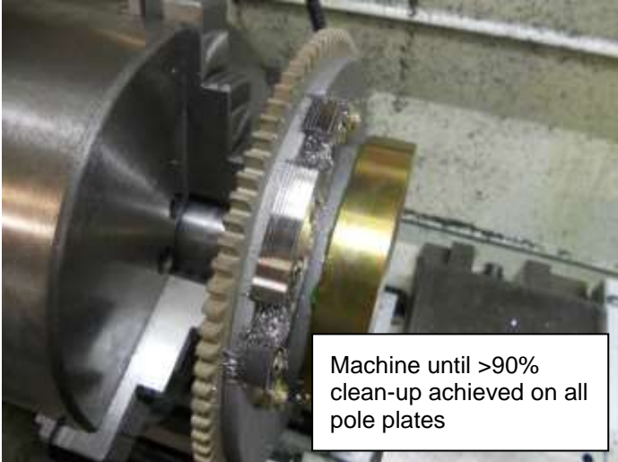
Figure 100 - Flywheel pole plate skimming
