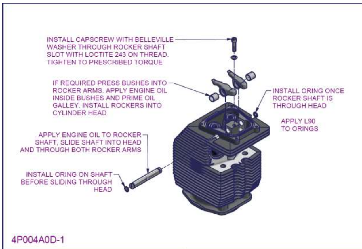
Figure 62 – 2200/3300 cylinder assembly 6b (Legacy 12mm rocker shaft cylinder head)
