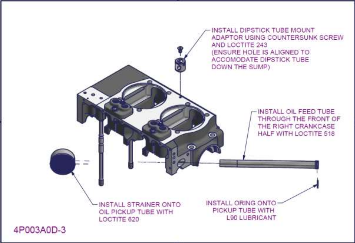
Figure 26 – 2200/330 crankcase subassembly 10
