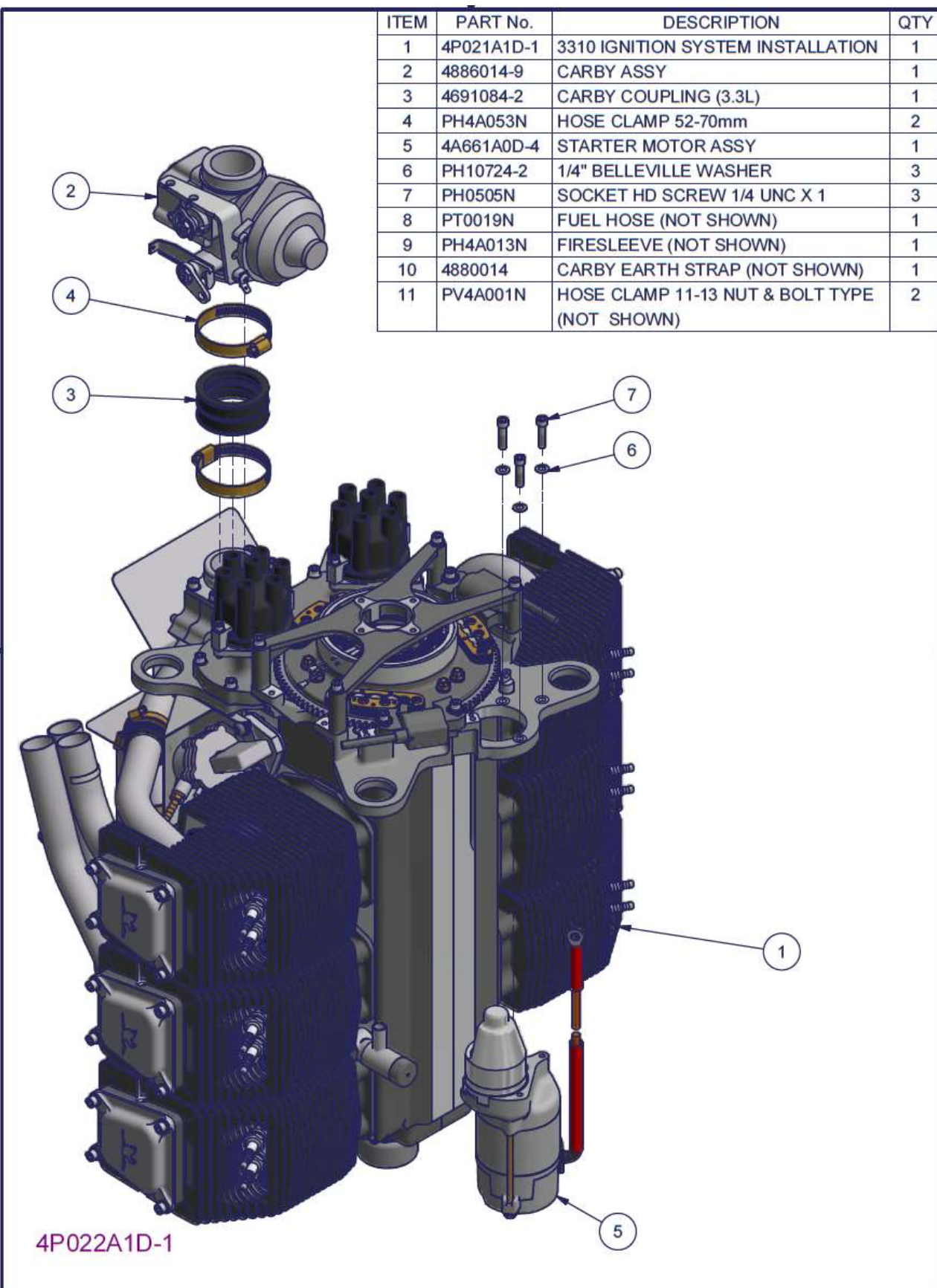
Figure 194 – 3300 Carburettor and Starter installation – Parts List
