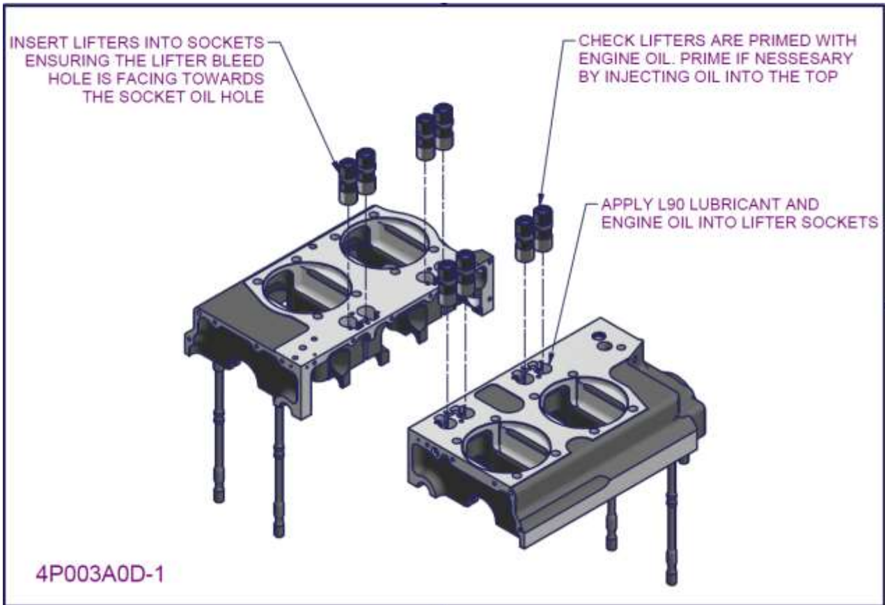
Figure 22 – 2200/330 crankcase subassembly 8
