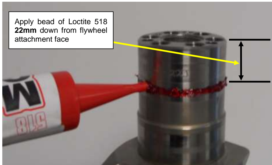
Figure 122 - Apply bead of Loctite 518 around perimeter of crank-gear
