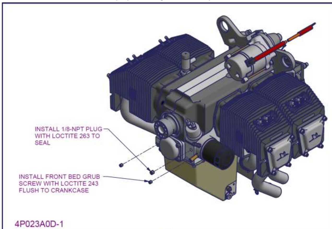
Figure 200 – 2200/3300 Front seal and propeller flange installation 1
