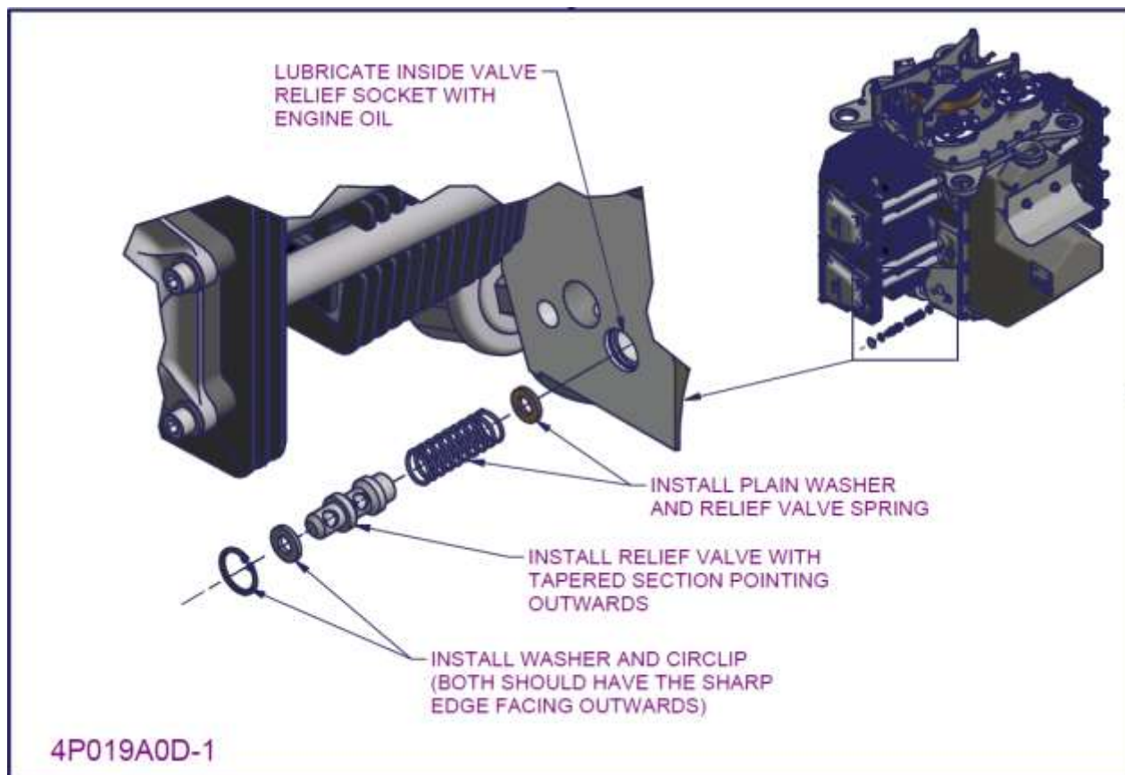
Figure 172 – 2200/3300 Oil pump and filter installation 2
