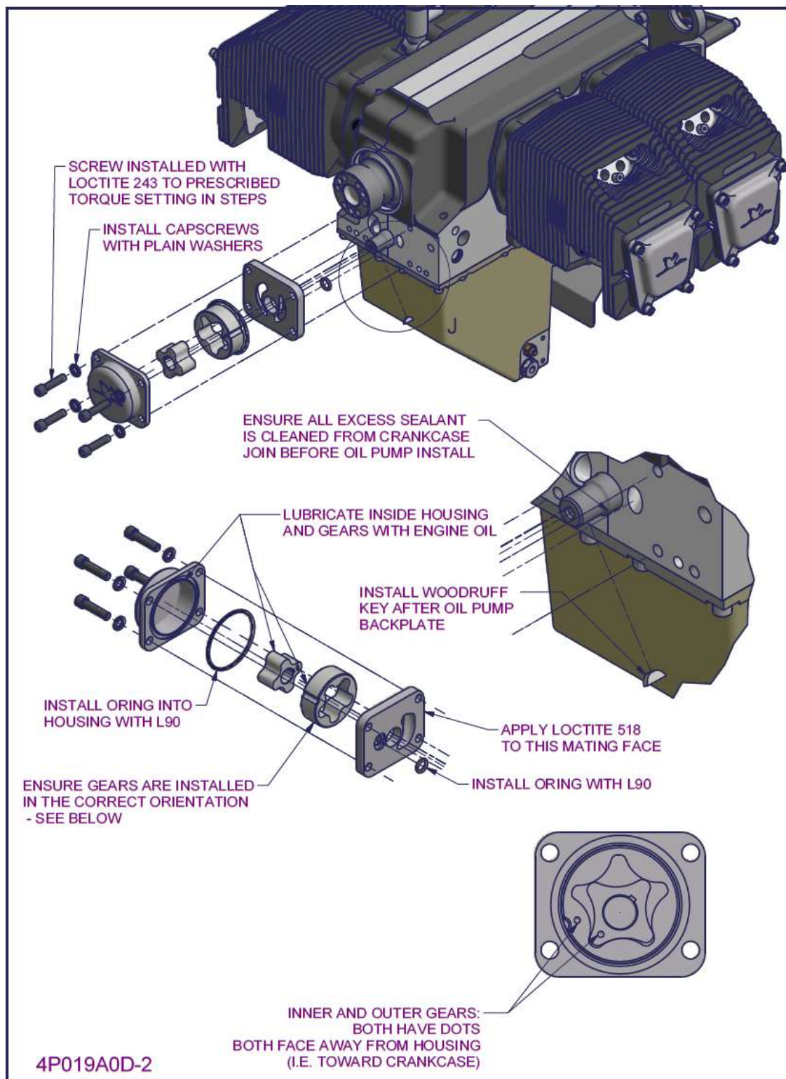
Figure 168 –2200/3300 Oil pump and filter installation 1A
