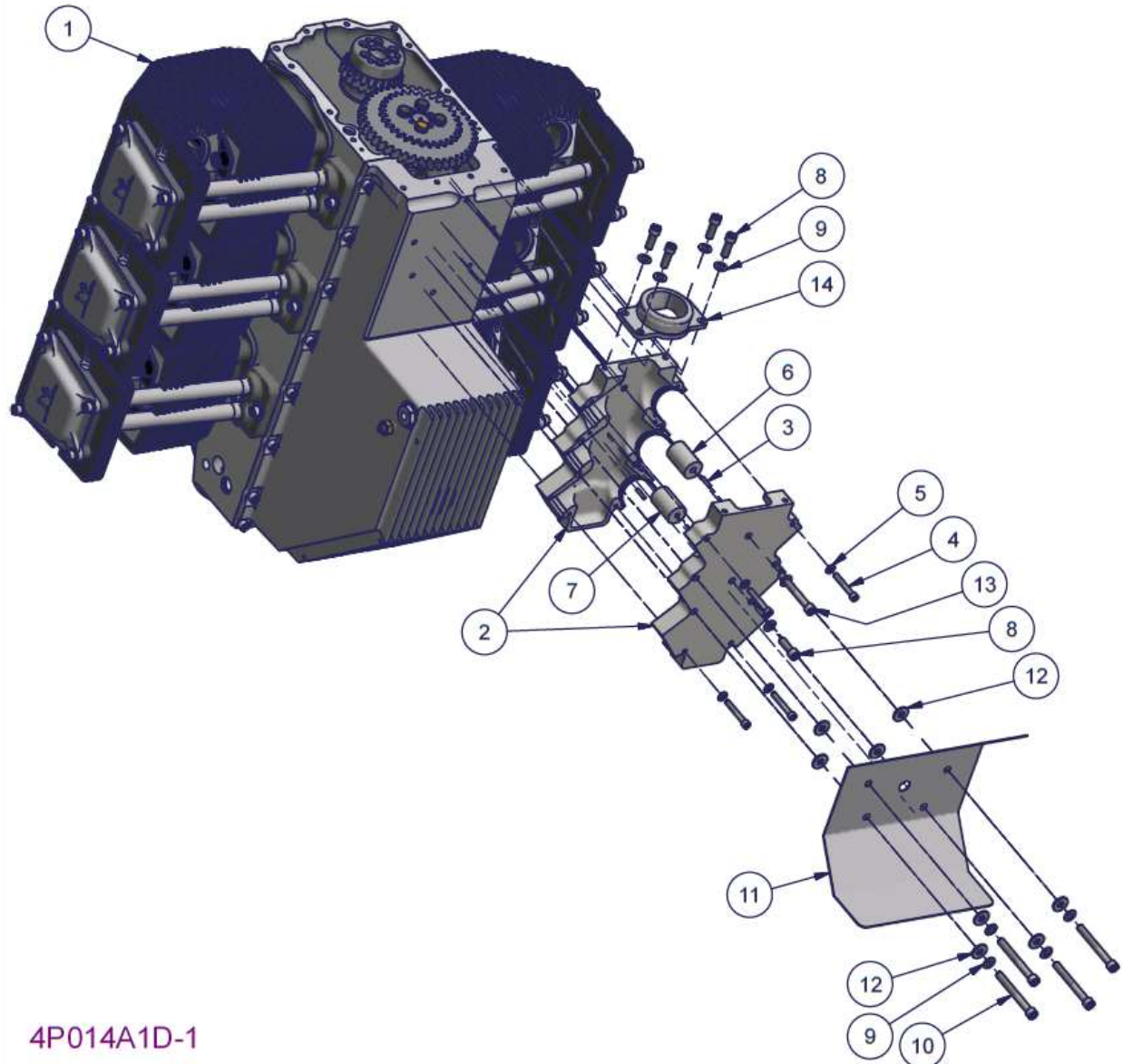
Figure 141 – 3300 Plenum and heat shield installation – Parts List
