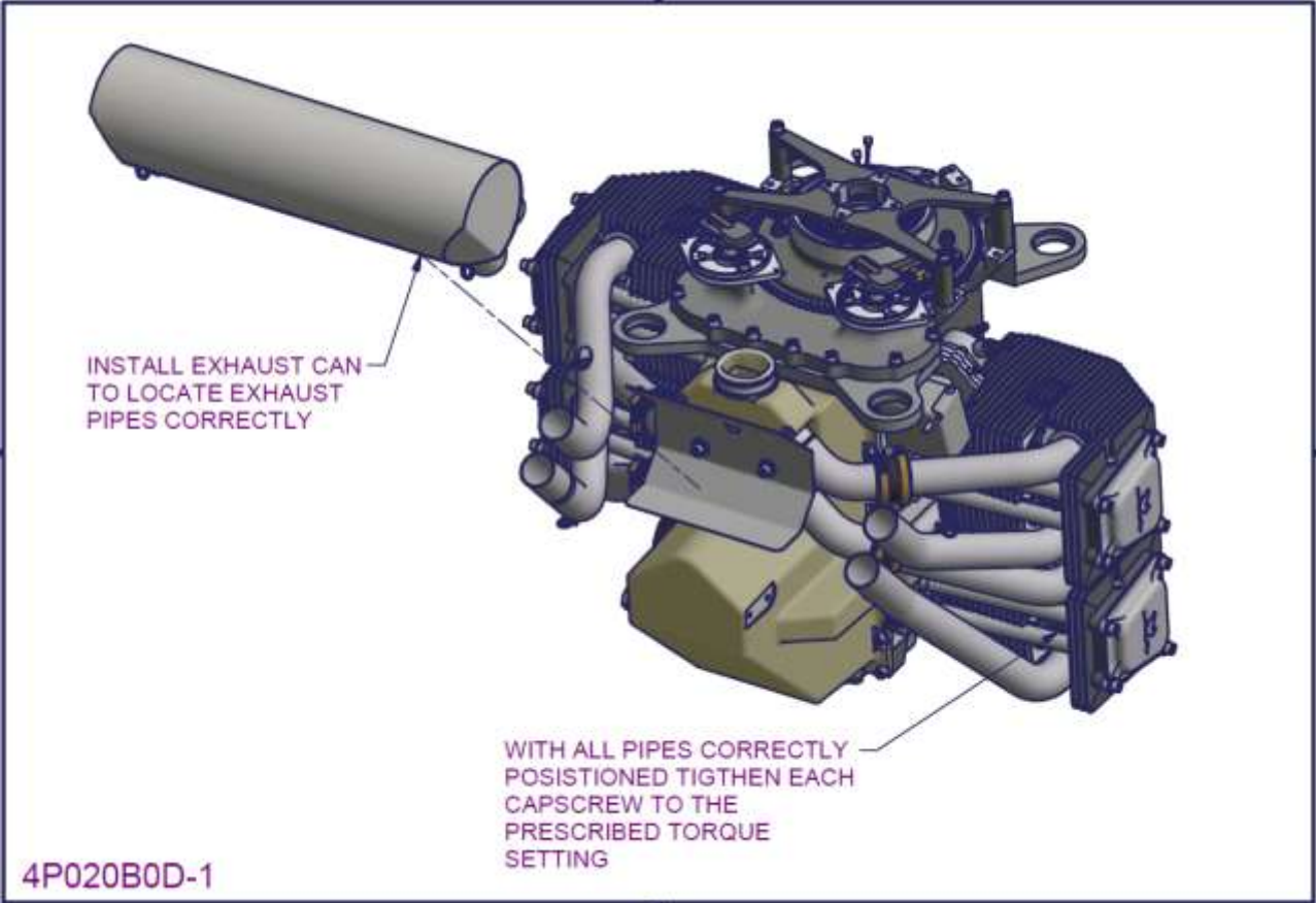
Figure 182 – 2200/3300 Exhaust and induction pipe installation 4
