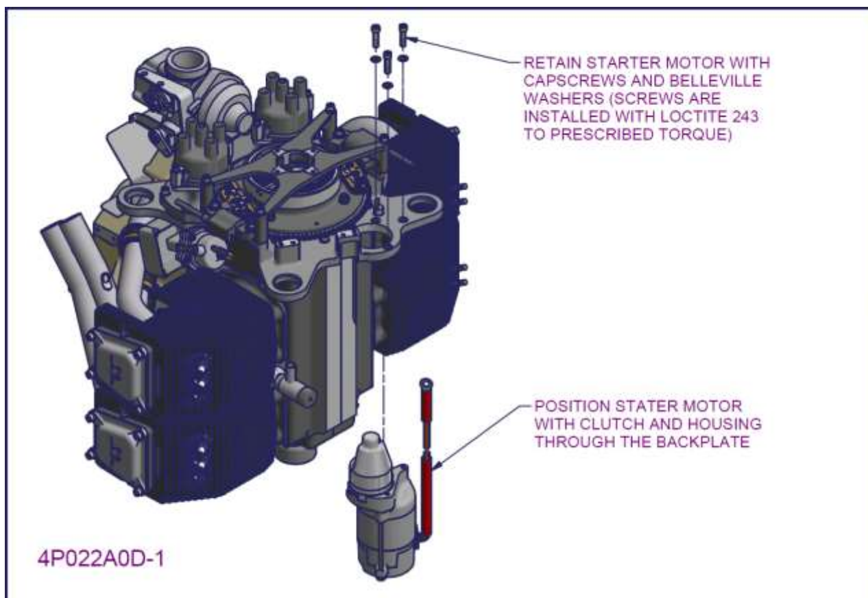
Figure 197 – 2200/3300 Carburettor and starter installation 2
