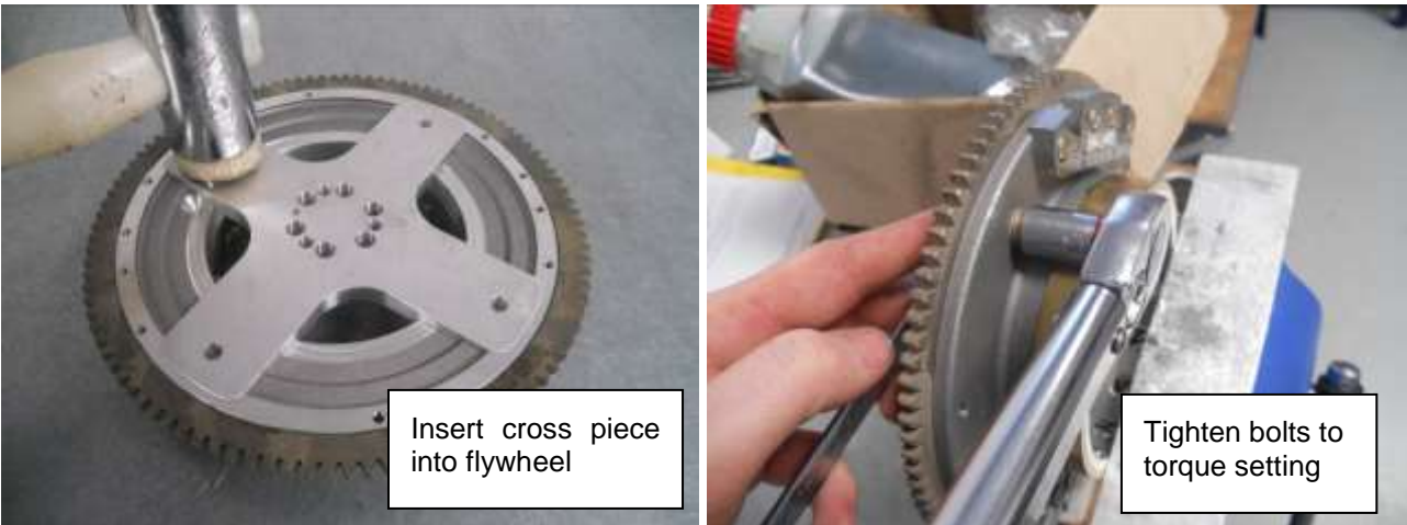
Figure 98 - Inner hub cross piece installation
