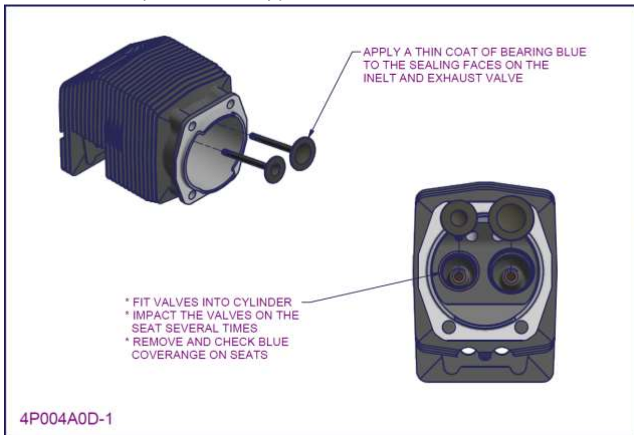
Figure 51 – 2200/3300 cylinder assembly 1
