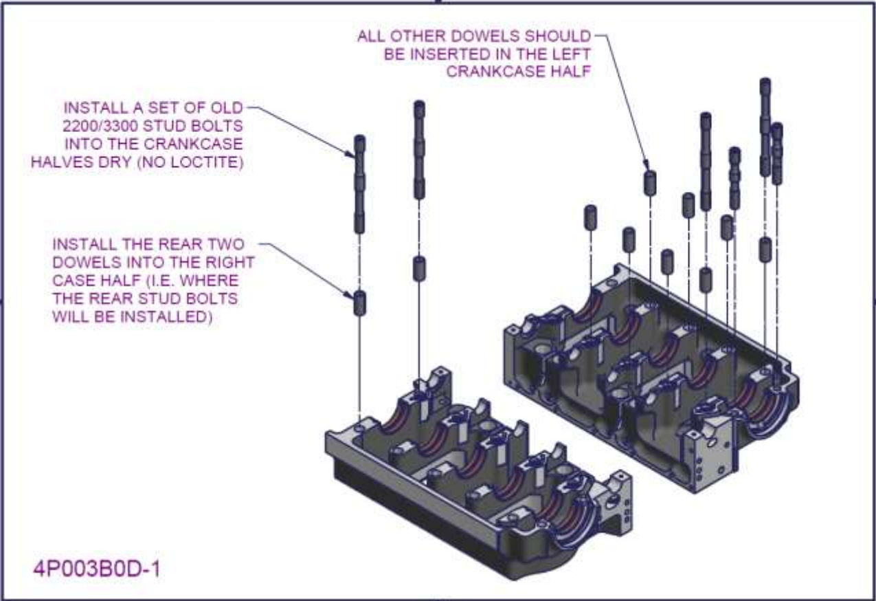
Figure 12 – 2200/330 crankcase subassembly 2
