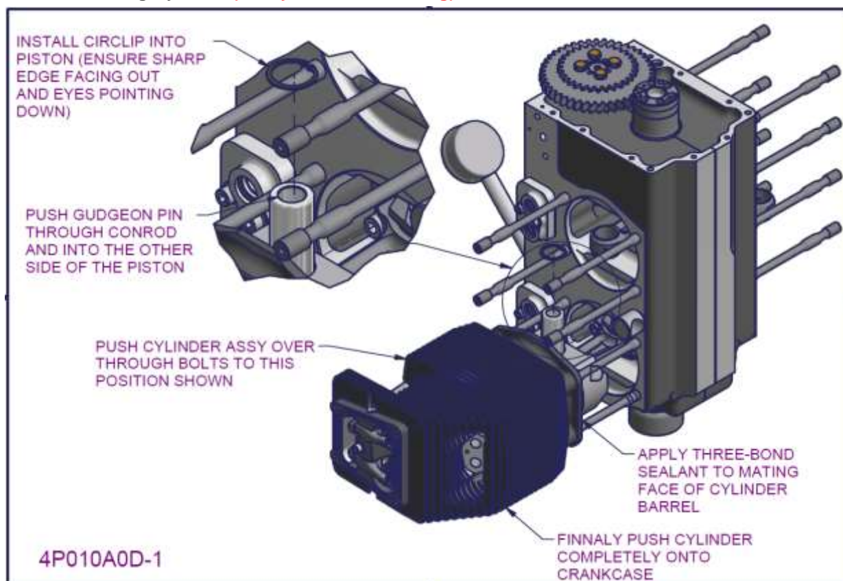
Figure 113 - 2200/3300 Joint engine assembly 3A
