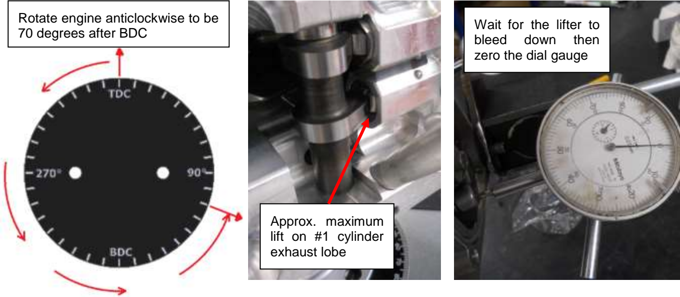
Figure 126 – setting zero on the dial gauge at approximate maximum lift (exhaust #1)
