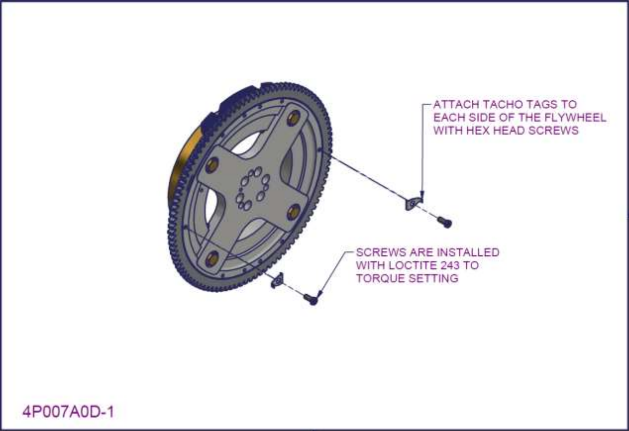
Figure 101 - 2200/3300 Flywheel subassembly (aluminium cross piece) 5
