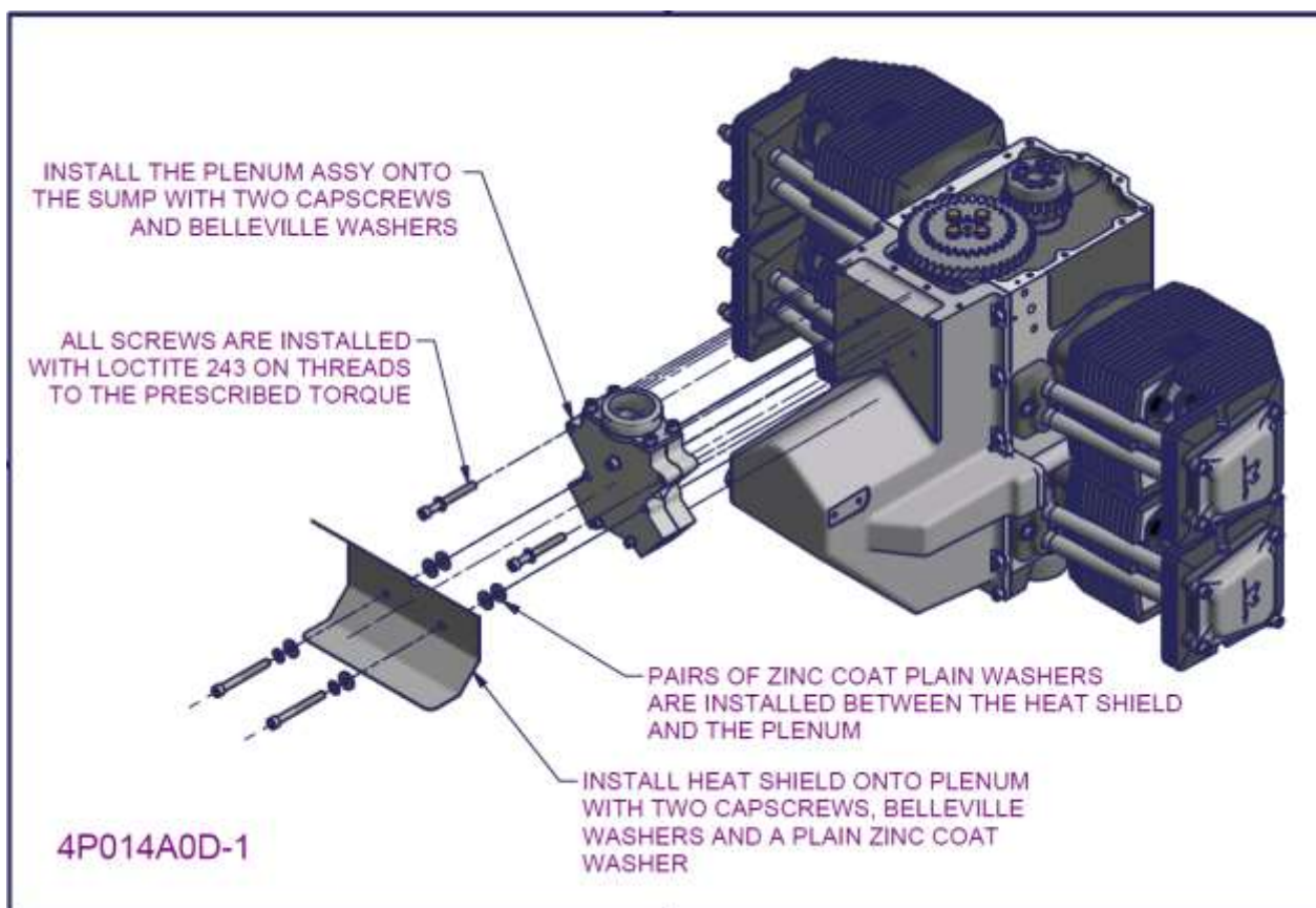
Figure 143- 2200/3300 Plenum and Heat shield installation 1
