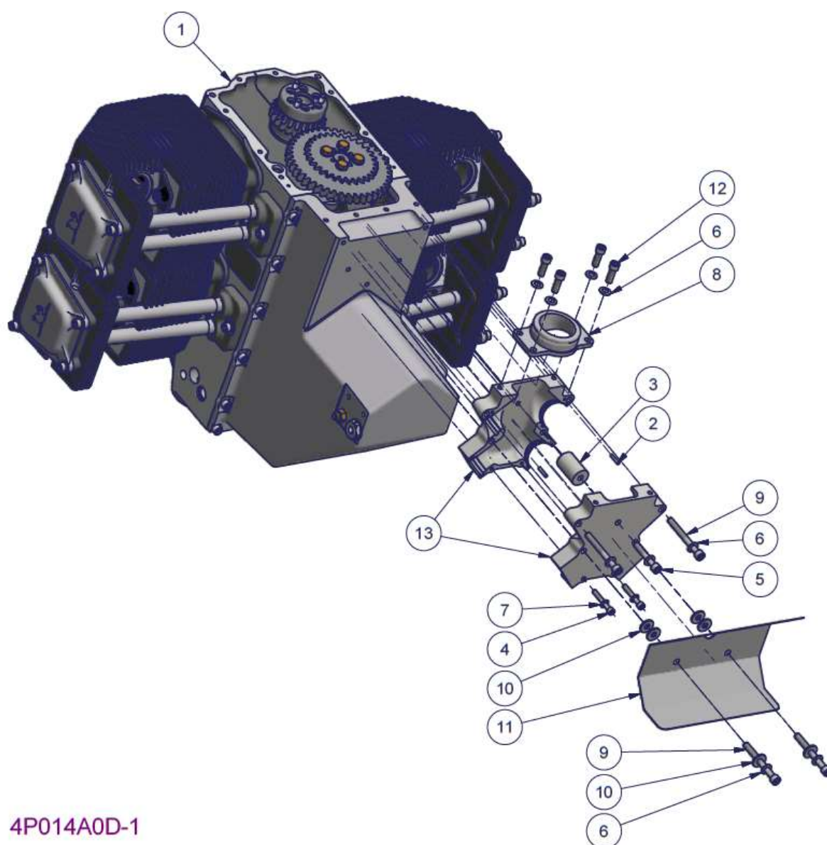
Figure 139 – Plenum and Heat shield installation – Parts List
