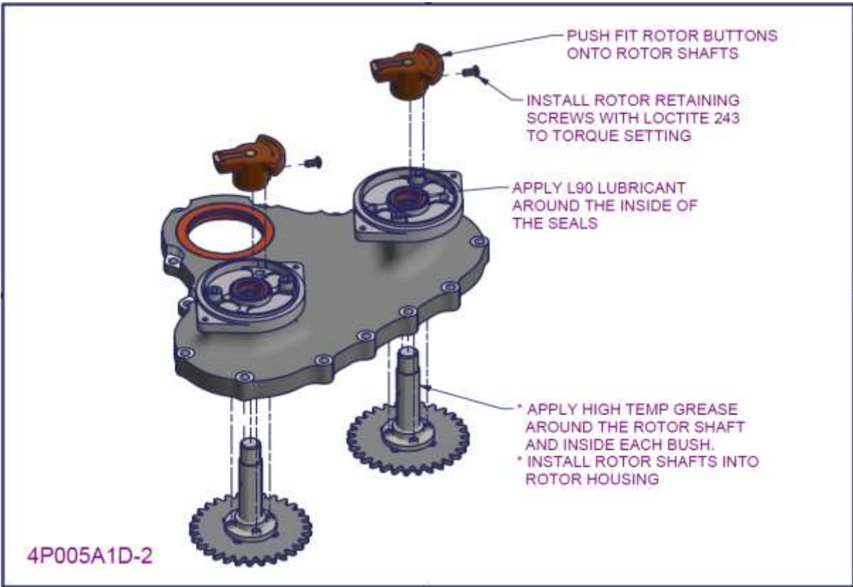
Figure 84 – 2200/3300 Distributor gearbox subassembly 6
