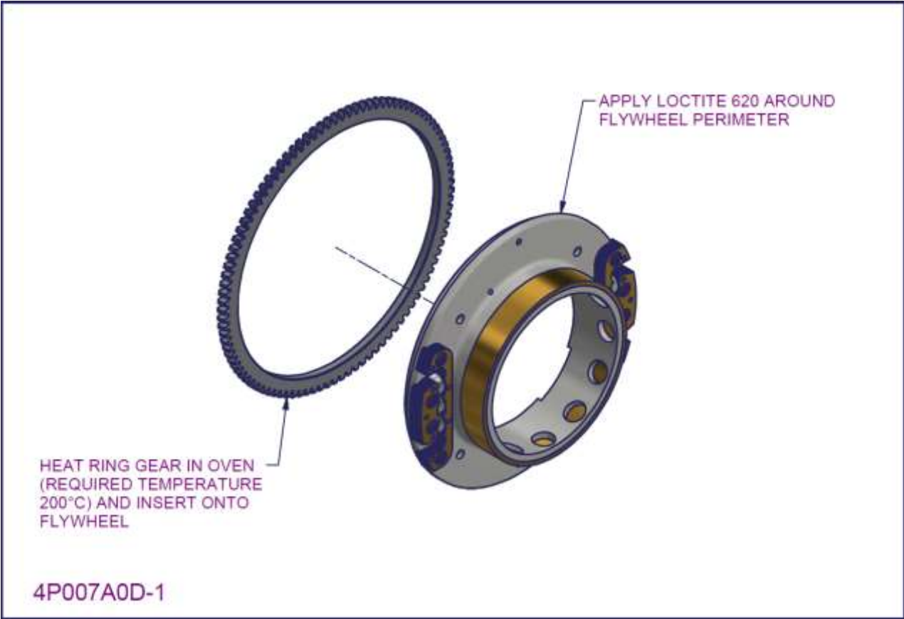
Figure 93 – 2200/3300 Flywheel subassembly (aluminium cross piece) 3
