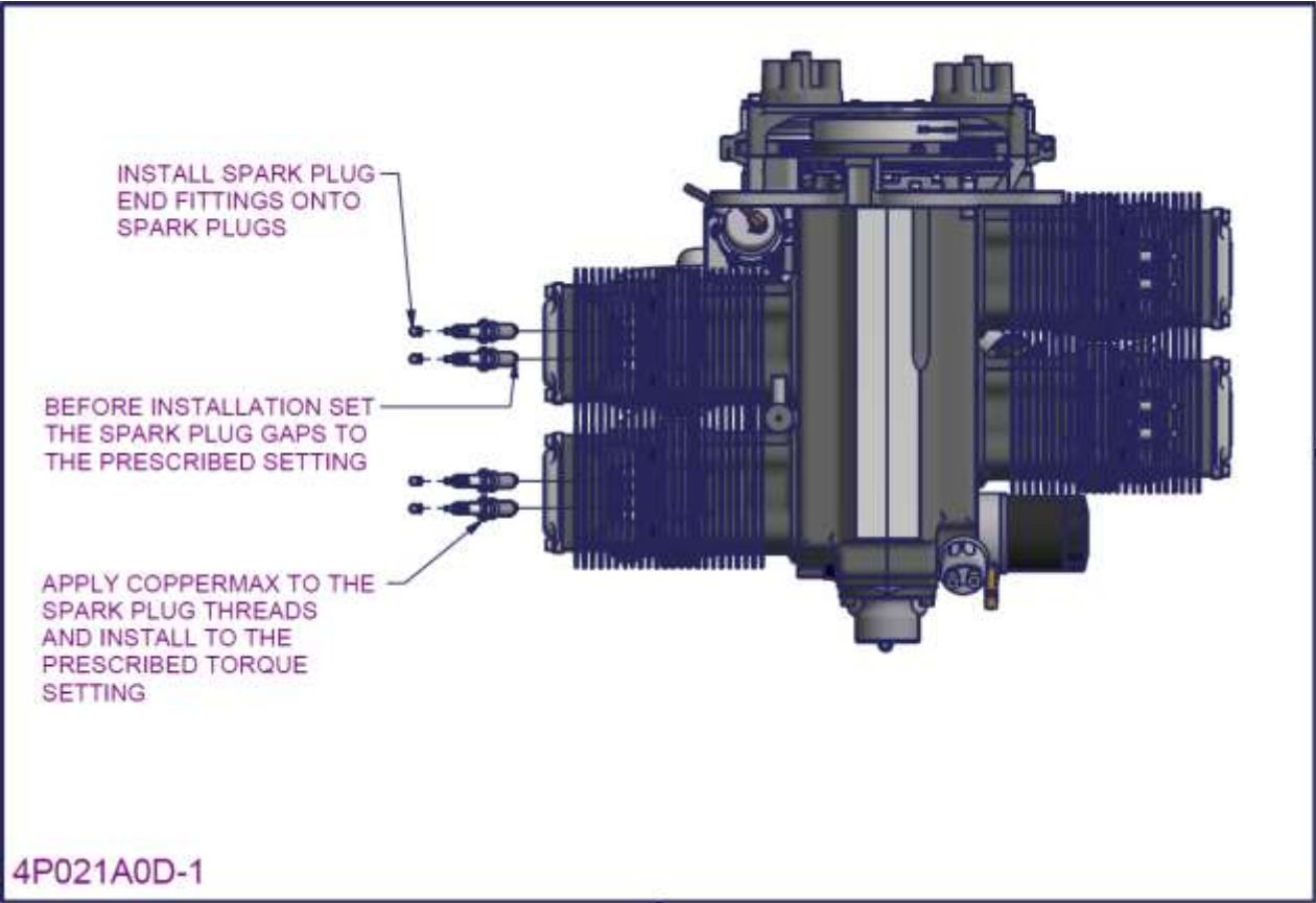
Figure 189 – 2200/3300 Ignition system installation 3
