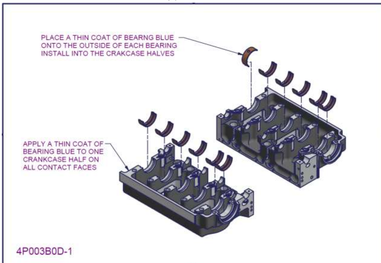
Figure 10 – 2200/3300 crankcase subassembly 1
