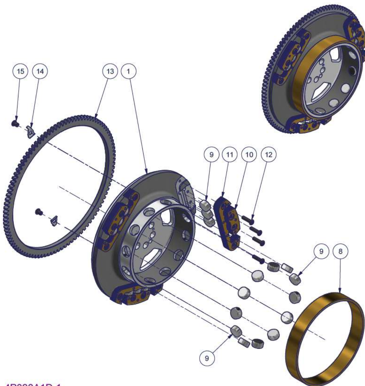
Figure 88 - 3300 Flywheel subassembly (integral cast centre) - Parts list
