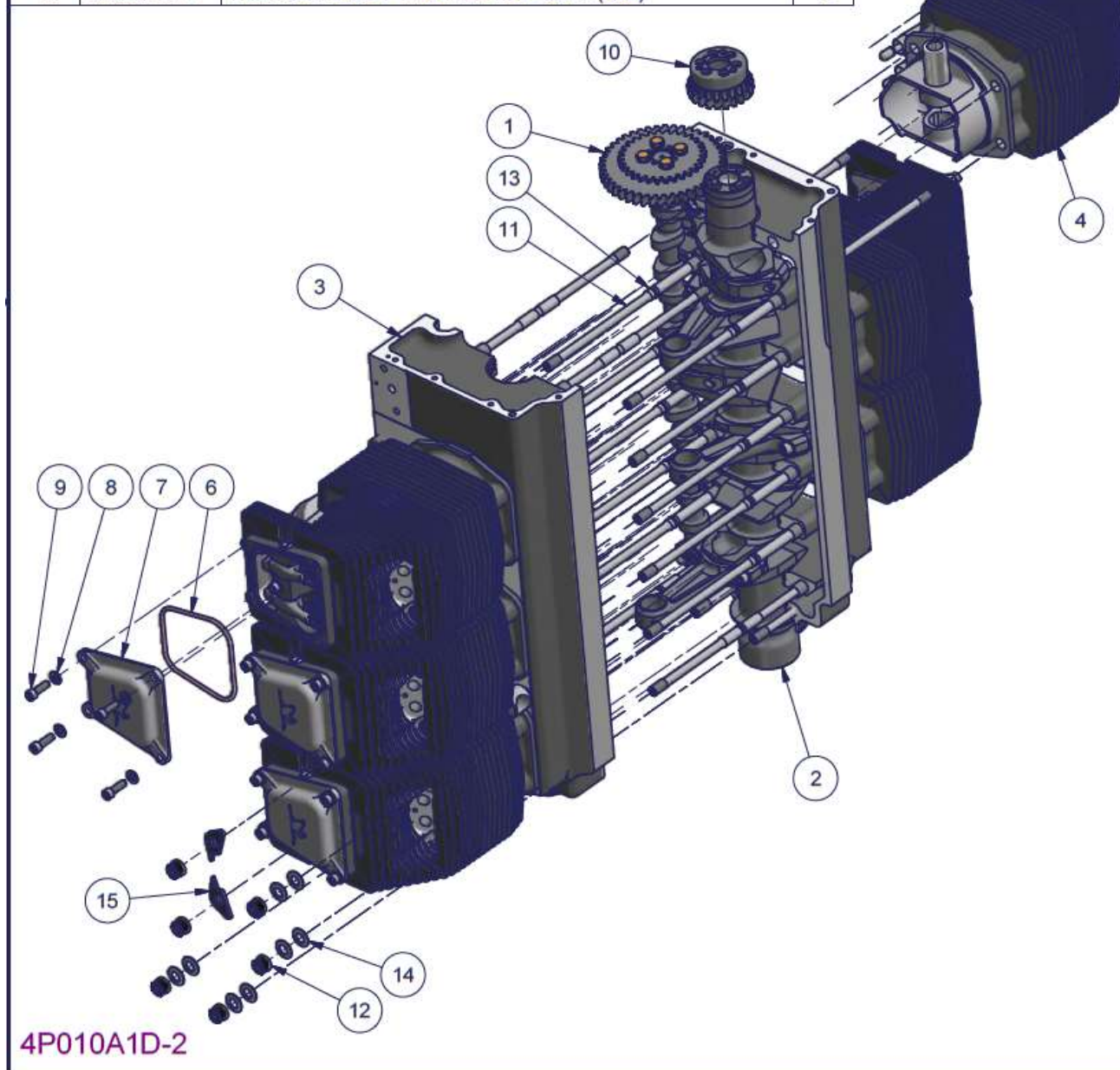
Figure 108 – 3300 joint engine – Parts List
