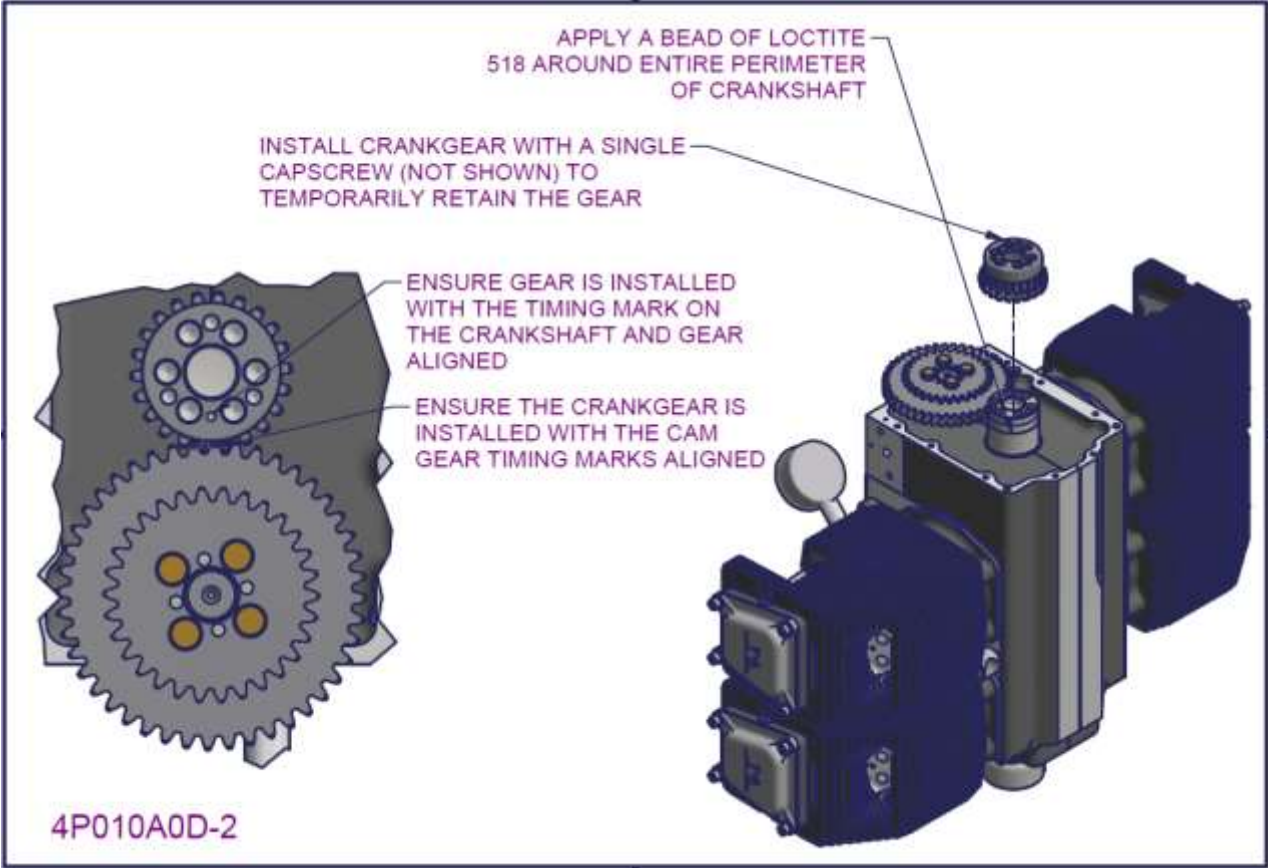
Figure 121 – 2200/3300 Joint engine assembly 7
