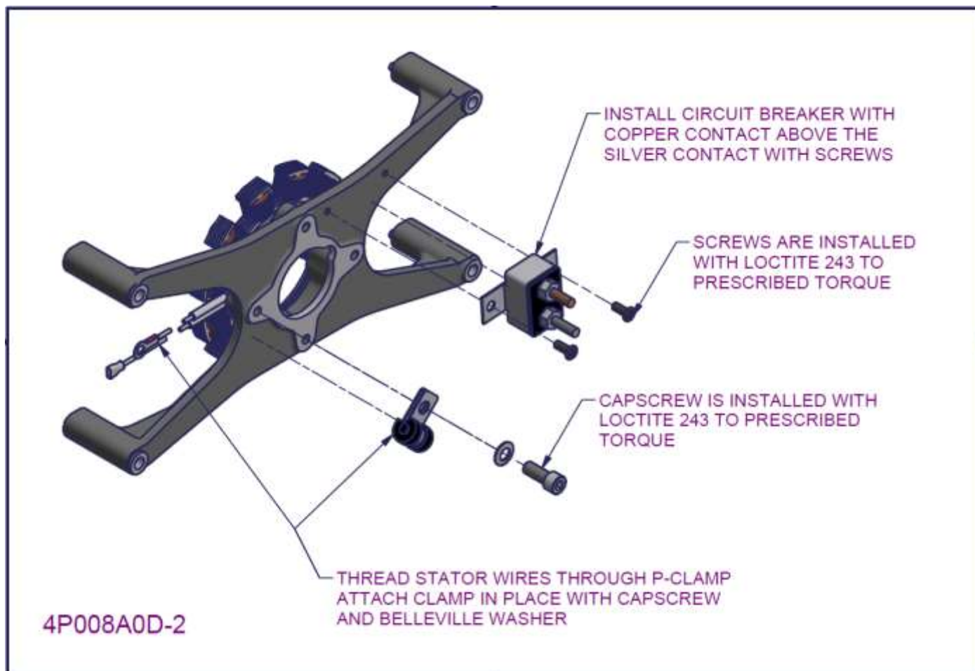
Figure 104 - 2200/ 3300 alternator stator subassembly 2
