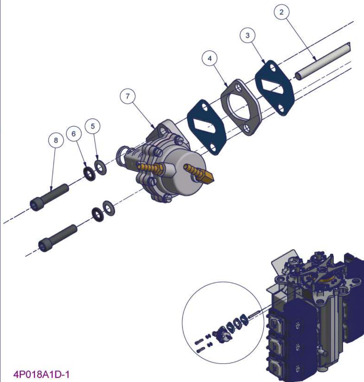
Figure 161 – 3300 Fuel pump installation – Parts List
