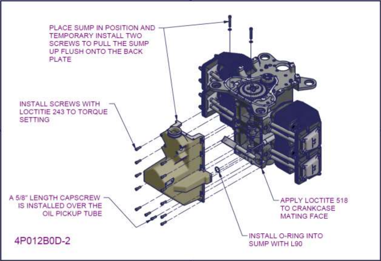
Figure 133 – 2200/3300 Sump installation 2
