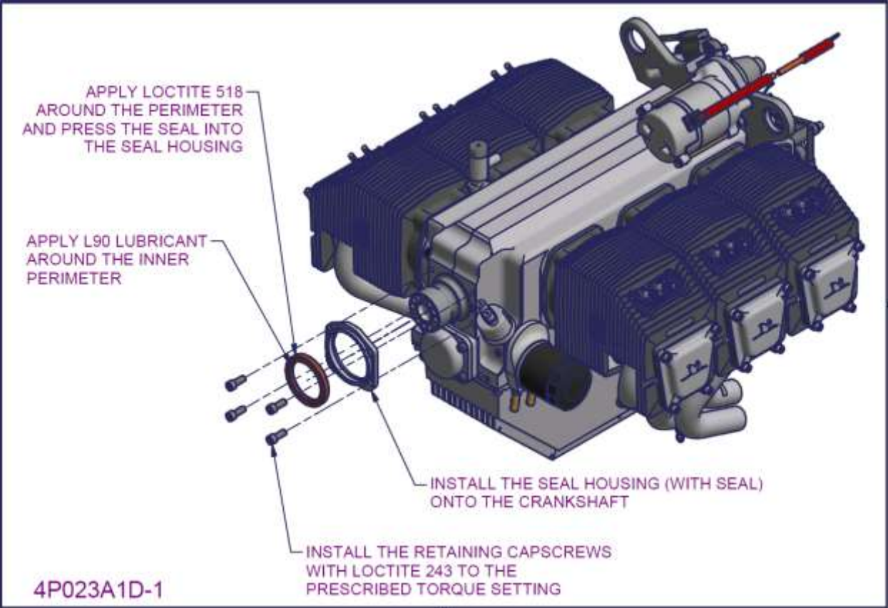
Figure 204 – Front seal installation for engines with a separate housing
