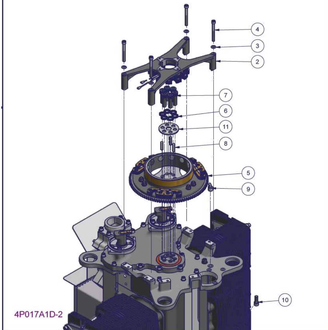
Figure 152 – 3300 flywheel and alternator installation – Parts List
