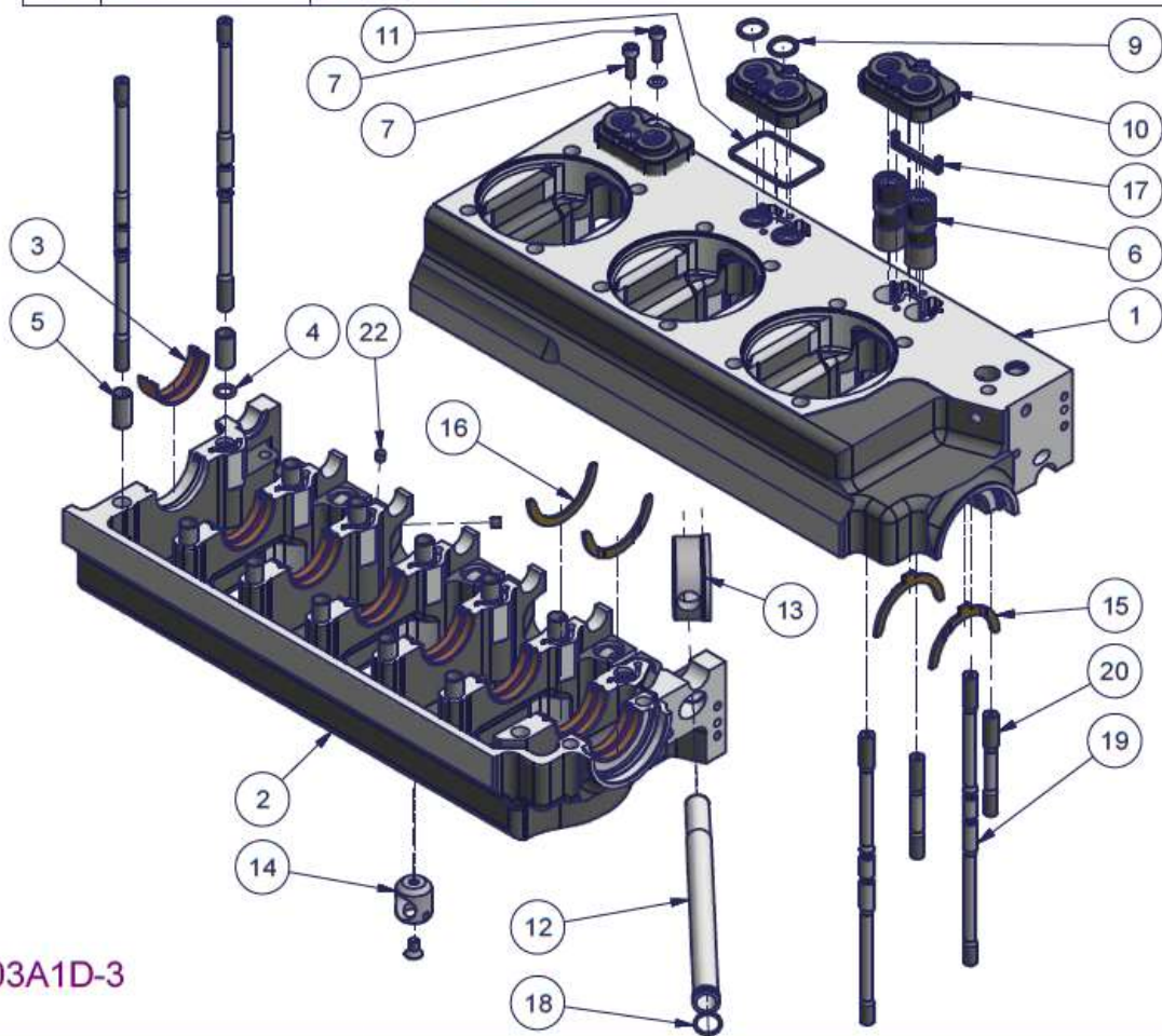
Figure 9 - 3300 Crankcase subassembly parts list
