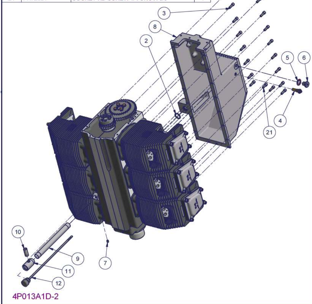
Figure 131 – 3300 Sump installation (No plenum) – Parts List
