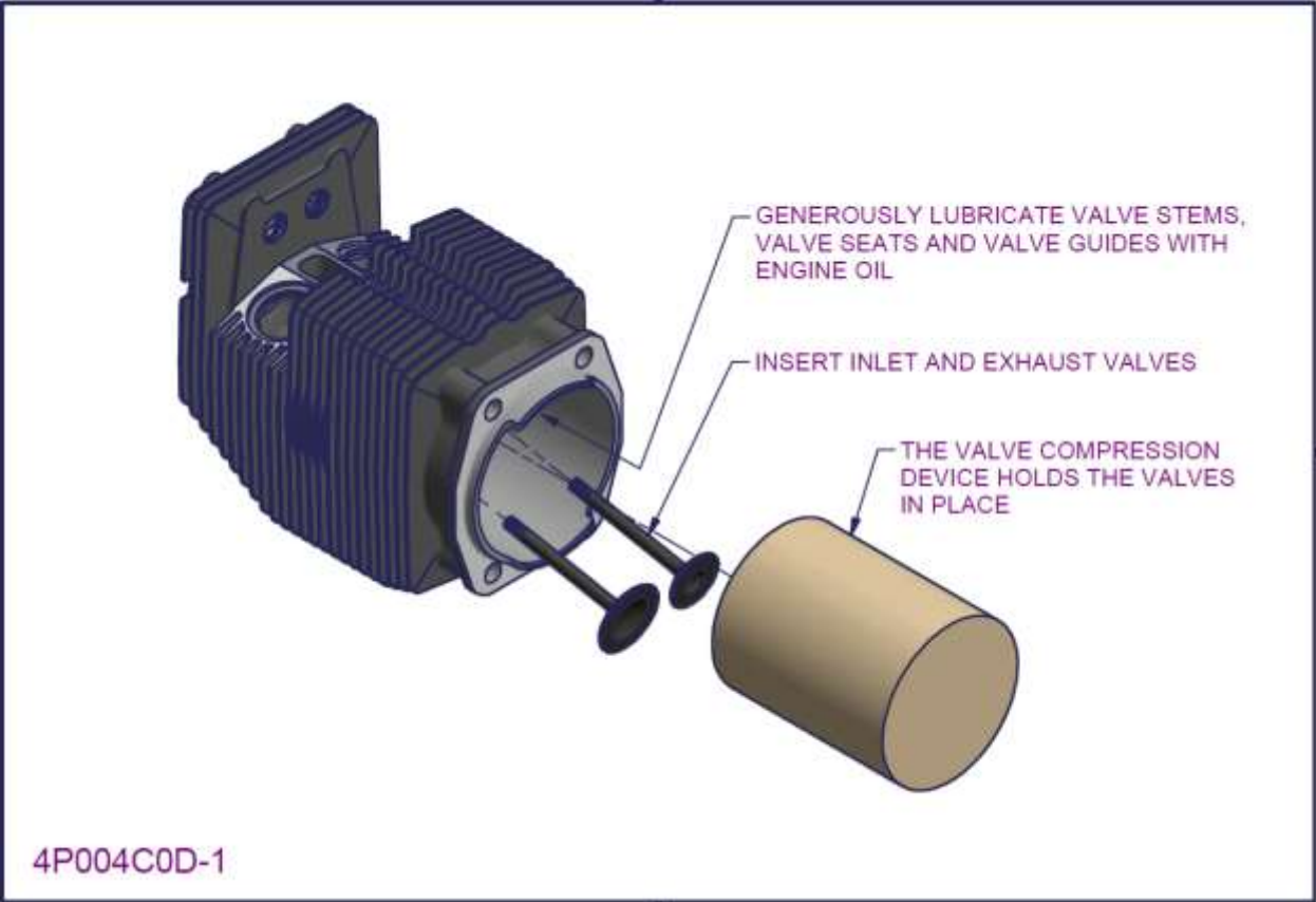
Figure 55 – 2200/3300 cylinder assembly 3
