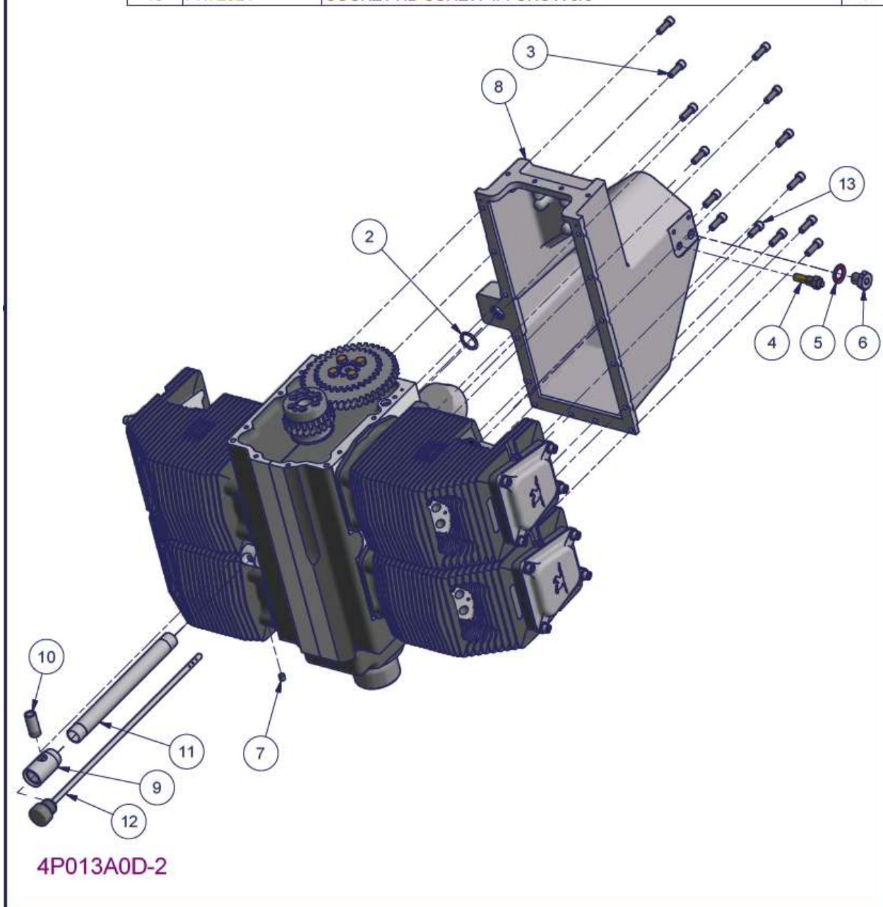
Figure 129 – 2200 Sump installation (machined plenum) – Parts List
