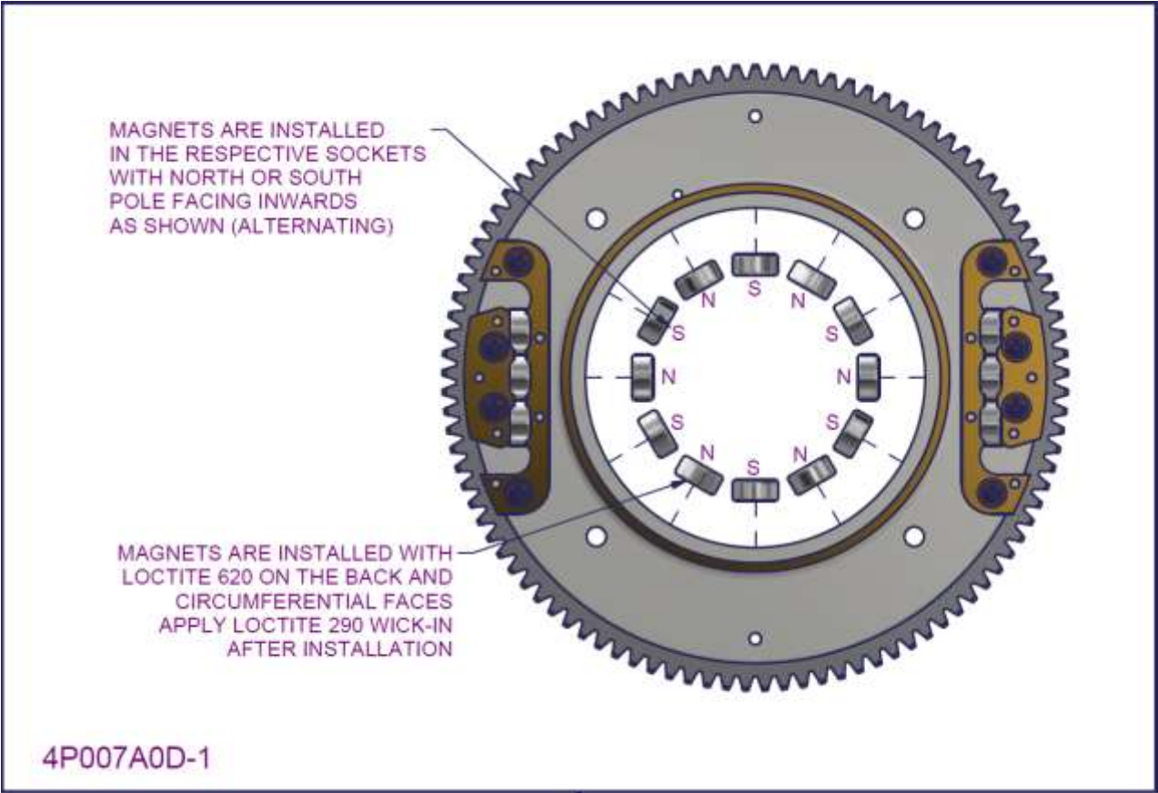
Figure 95 - 2200/3300 Flywheel subassembly (aluminium cross piece) 3
