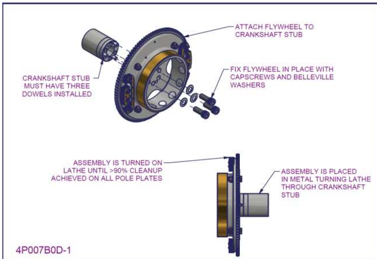
Figure 99 - 2200/3300 Flywheel subassembly (aluminium cross piece) 6
