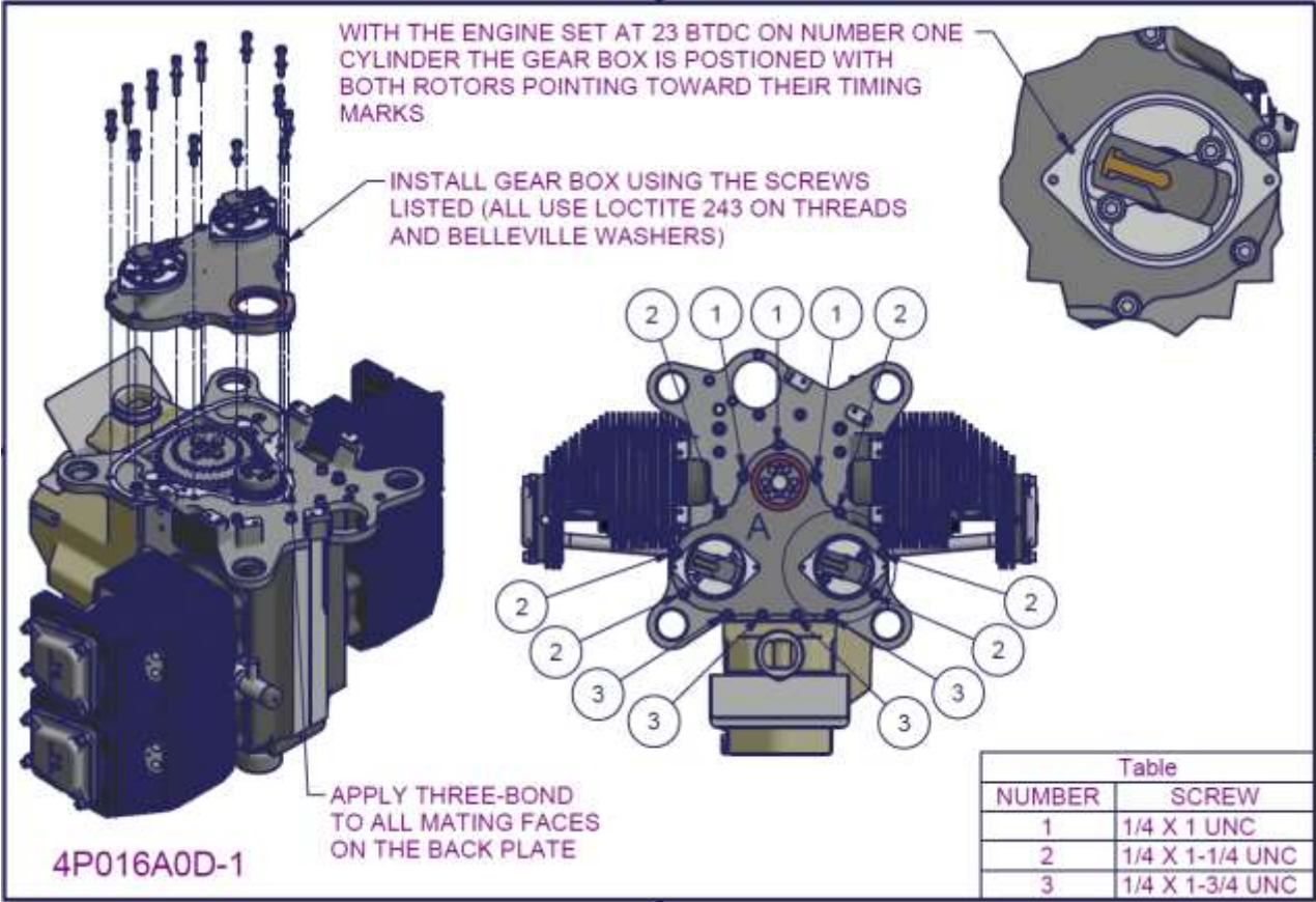
Figure 149 – 2200/3300 back plate and distributor gearbox installation 3
