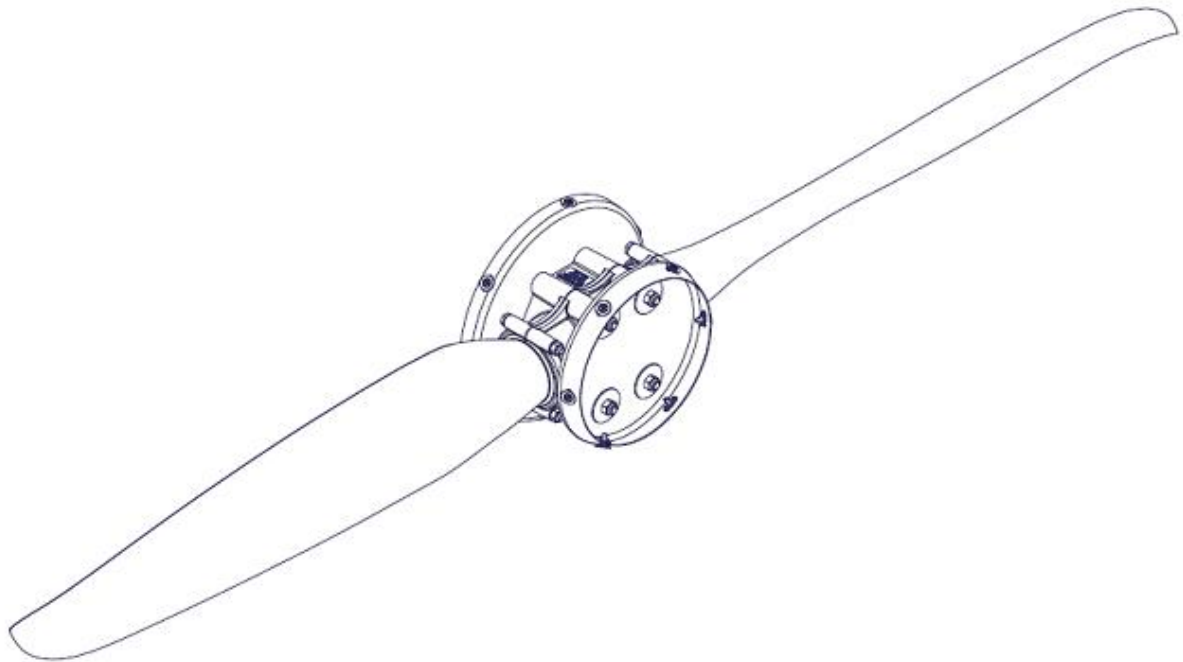
Figure 1 – 4A482U0D Propeller Assembly (Spinner Not Shown)
