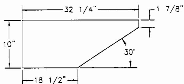
UP DEFLECTION TEMPLATE
