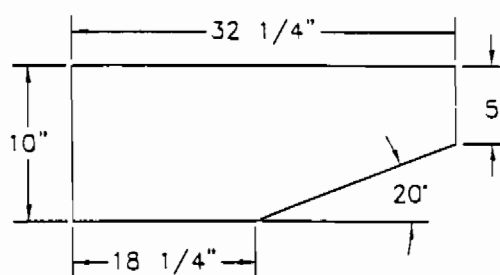
DOWN DEFLECTION TEMPLATE
