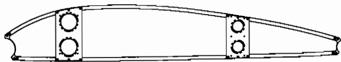
#1 RIB, LEFT HAND - (2) REQ'D. (2 USED IN THE LEFT HAND WING, POSITION #1 & 5.)
