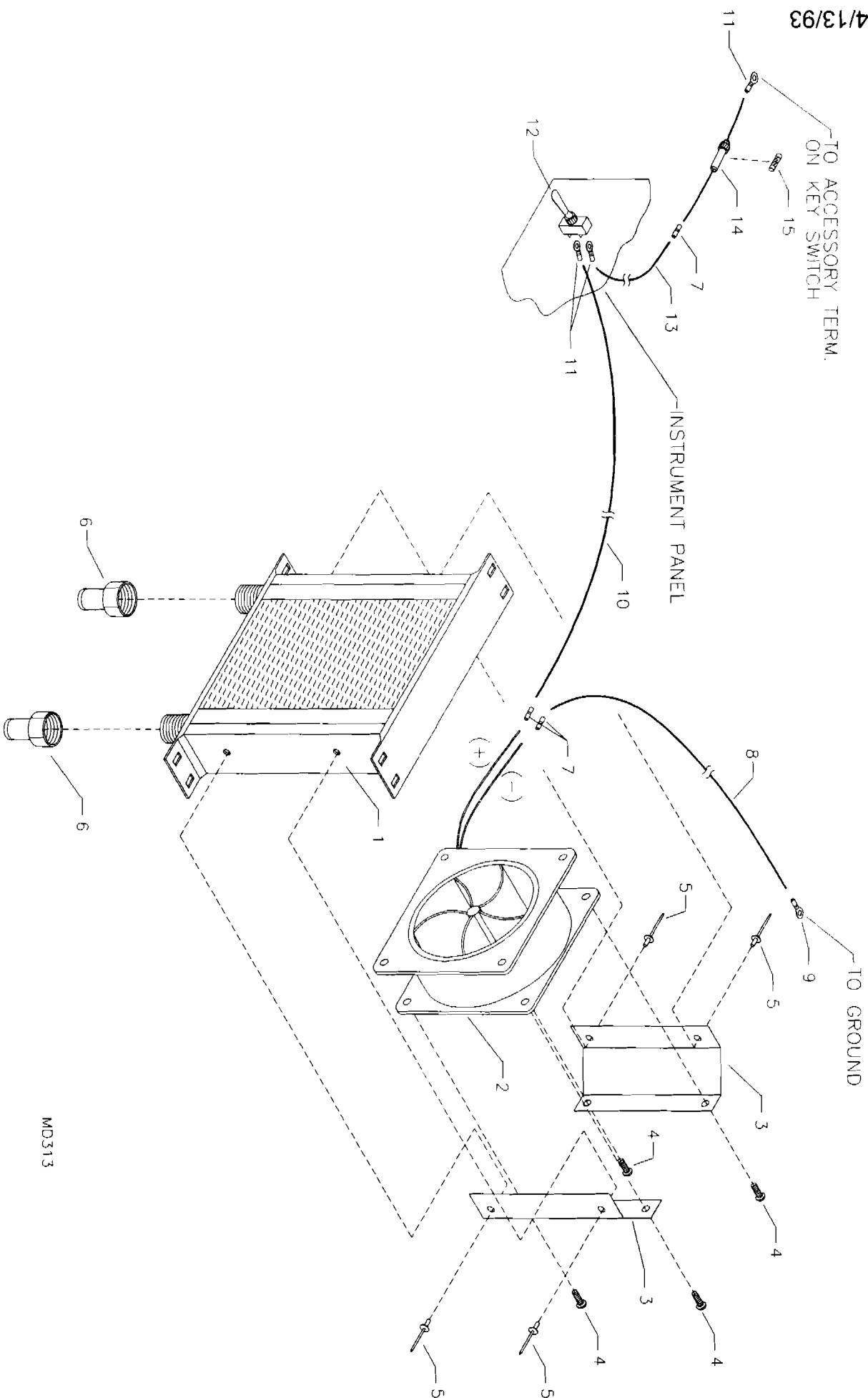
RRAD-63 S-6S COYOTE II HEATER CORE ASSEMBLY
