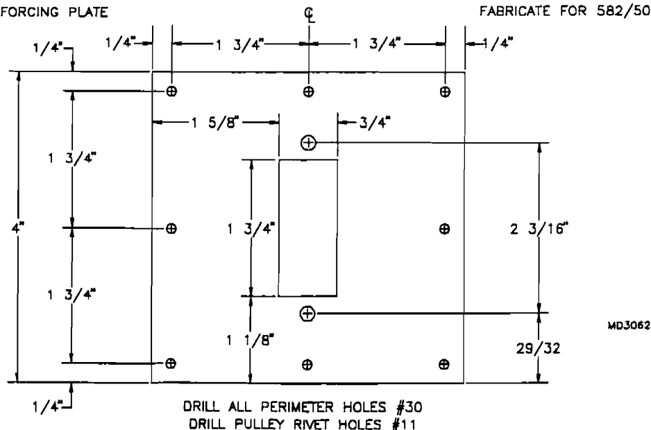
FIREWALL STARTER PULLEY REINFORCING PLATE
