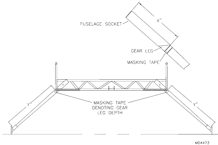
FIGURE 02-03-TAILDRAGGER
