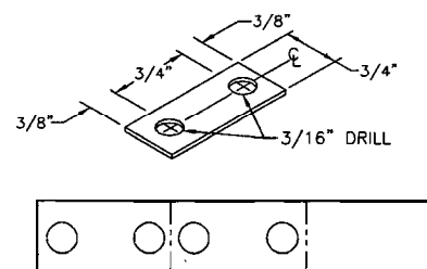
ADJUSTABLE STRUT SHIM
